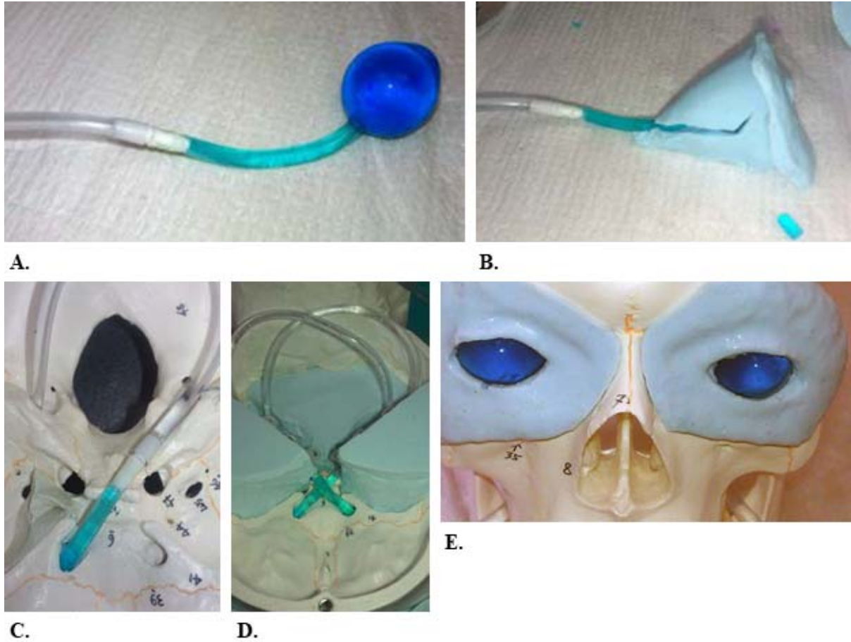
Figure 2. Connecting the Human Eye Model. A. Eye model ported to cannula line. B. Eye model inserted into eye holder. C. View of port connection from inside the cranium. D. View of overlapping ported ends of the optics nerves for mounting two eye models. E. Dual eye mounting into the skull headform.
