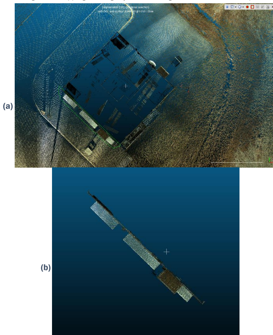
Figure 4. Cropping building façades with Segment Tool in CloudCompare.
