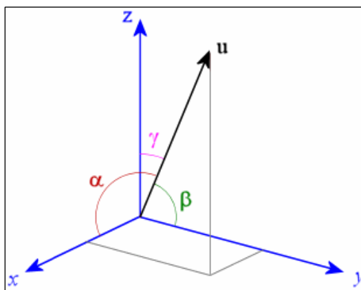
Figure 10. Backplane normal vector angles in 3D space.
