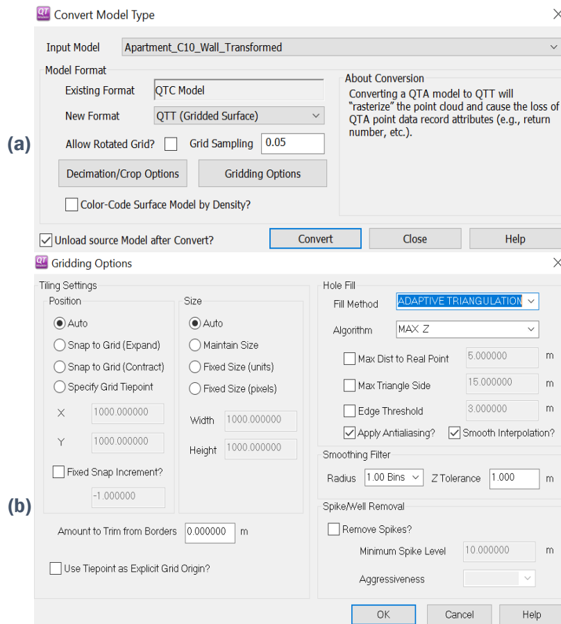
Figure 6. QT Modeler parameter settings for point cloud conversion (a) and gridding (b).
