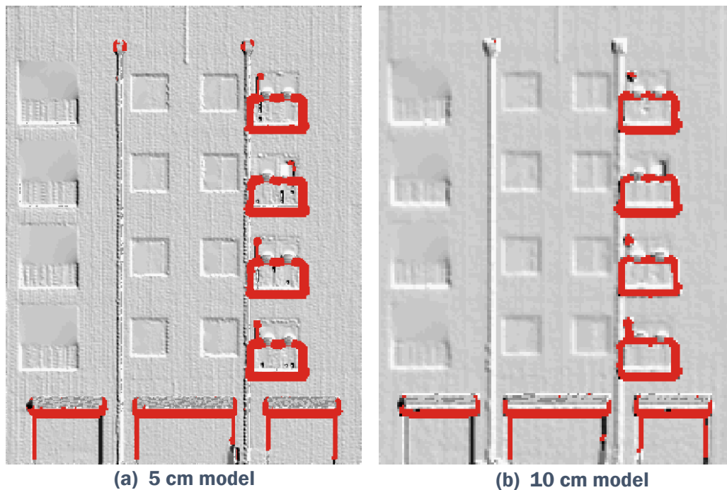
Figure 19. Breakline analysis for extruded features.
