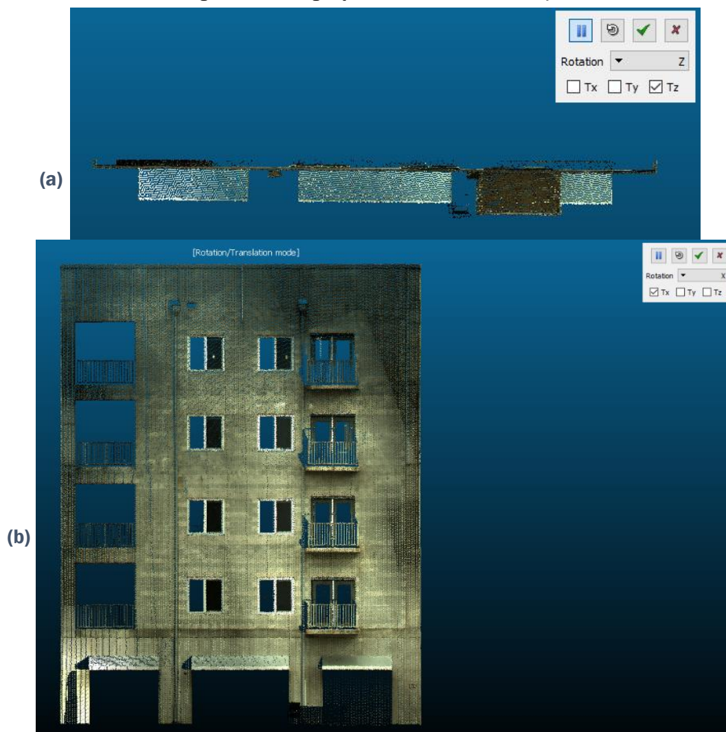
Figure 5. Building façade rotation in CloudCompare.
