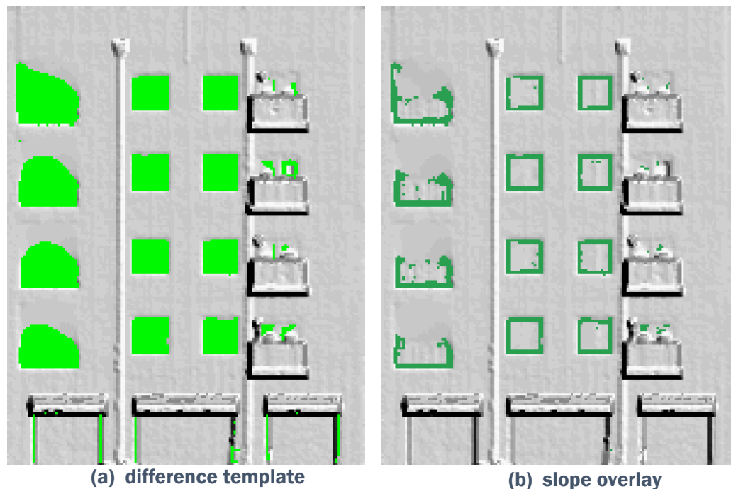
Figure 18. Slope analysis for intruded features (10 cm model).
