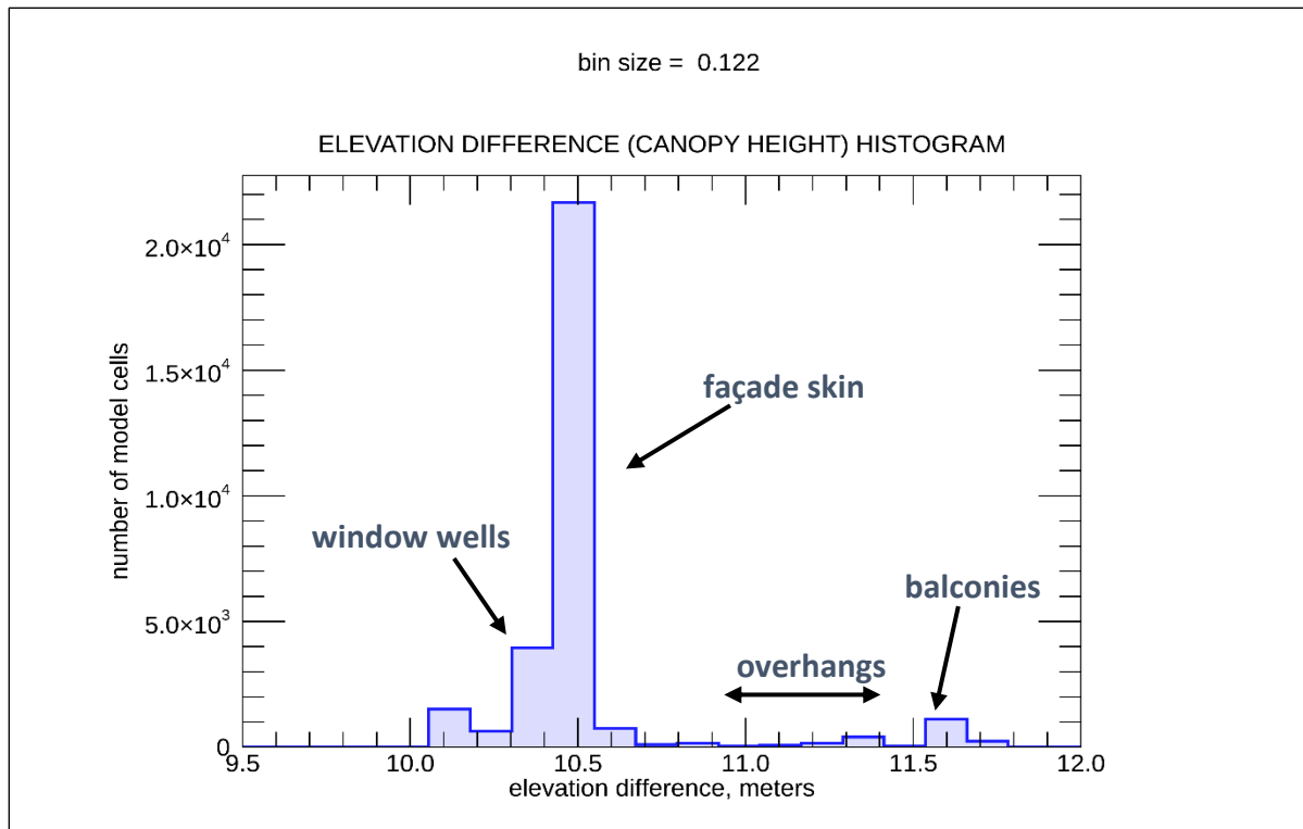
Figure 16. Elevation difference histogram for the 10 cm facade model.
