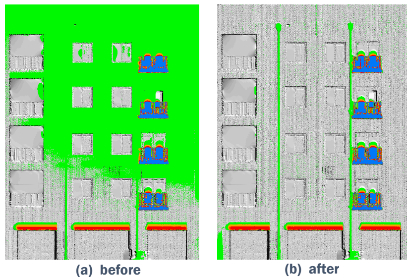
Figure 12. Results of backplane orientation adjustment.
