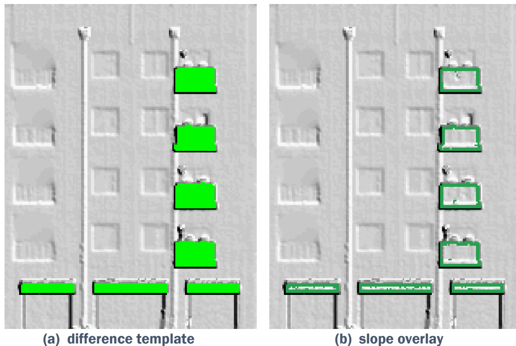
Figure 17. Slope analysis for extruded features (10 cm model).
