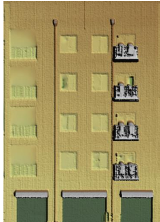
Figure 7. Gridded surface model derived from point cloud.
