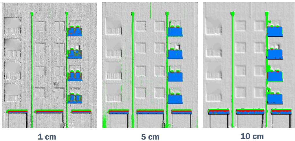
Figure 15. Differencing extruded feature overlays for three grid resolutions.
