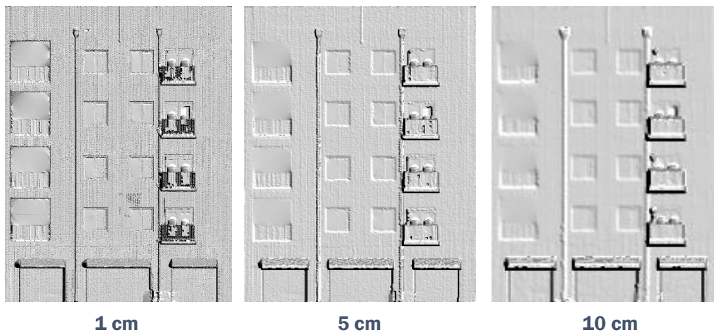
Figure 14. Façade model for three grid resolutions.
