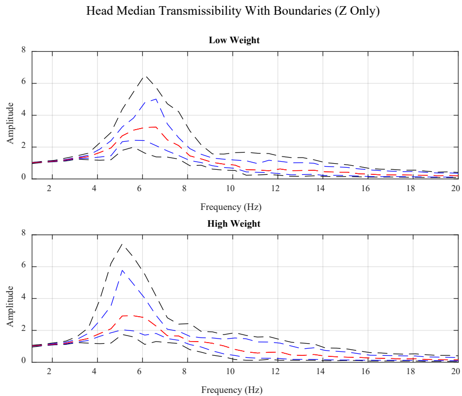
Figure 19. Head median transmissibility compared between the LW and HW categories.
