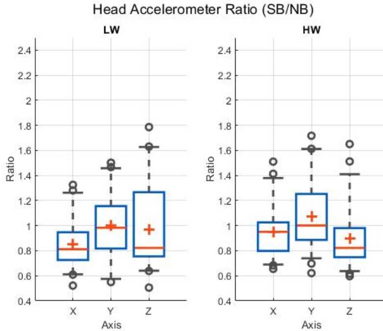
Figure 21. Box plot comparing the SB/NB RMS ratio for HW and LW categories.
