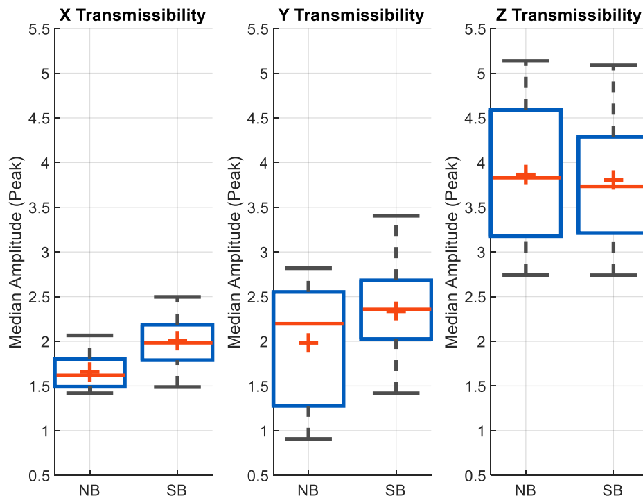
Figure 36: A plot comparing the peak median transmissibility of the non-immobilized and immobilized conditions. Transmissibilities are measured at the hip.
