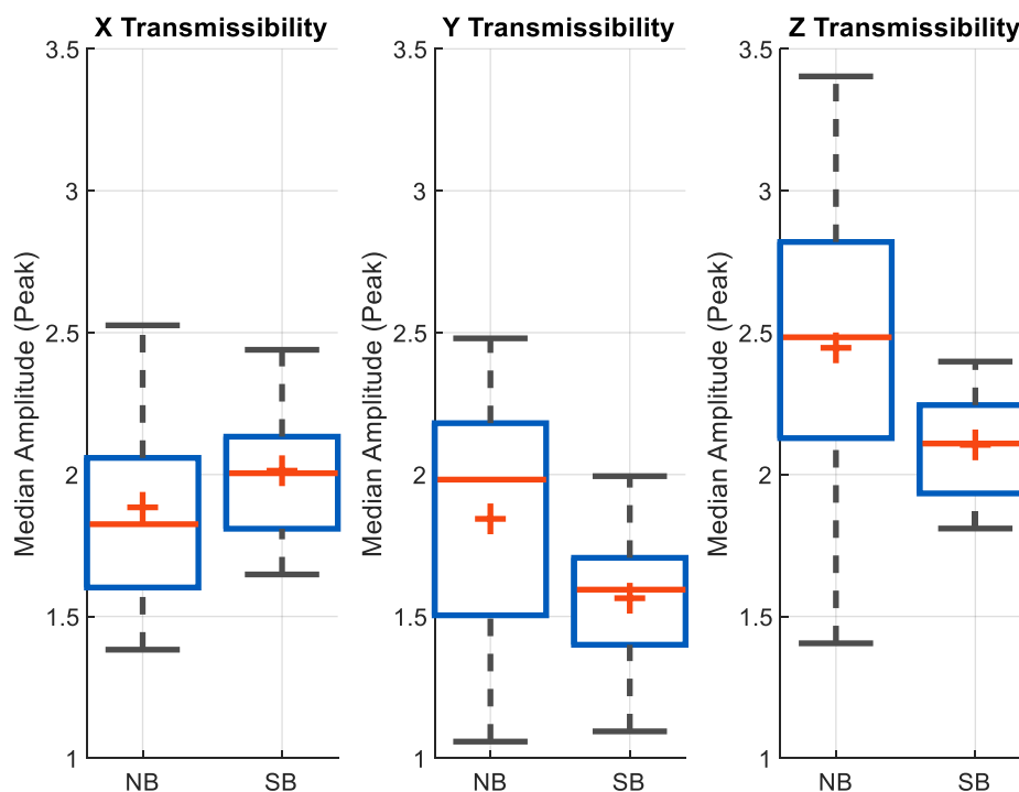
NB and SB boxplots (Head)
