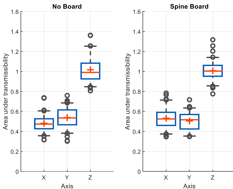
Figure 38: Boxplots representing the area underneath the transmissibility curve, measured at the chest and dependent on immobilization condition.
