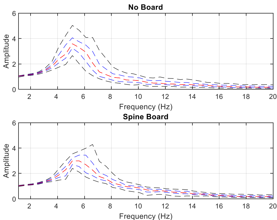
Figure 29: An overlaid transmissibility plot for the chest comparing the immobilized and non-immobilized conditions. The red line represents the subject median transmissibility, the blue line represents the 25th to 75th percentile, and the black line represents the 5 th to 95 th percentile.
