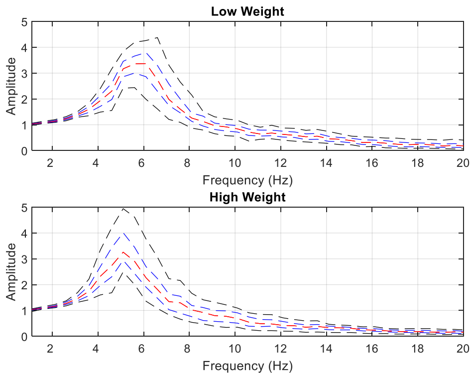
Figure 26: An overlaid transmissibility plot for the chest comparing the LW and HW groups. The red line represents the subject median transmissibility, the blue line represents the 25 th to 75 th percentile, and the black line represents the 5 th to 95 th percentile.
