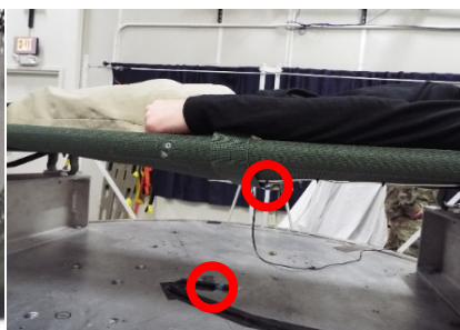
Figure 14. Test setup showing sensor positions.
