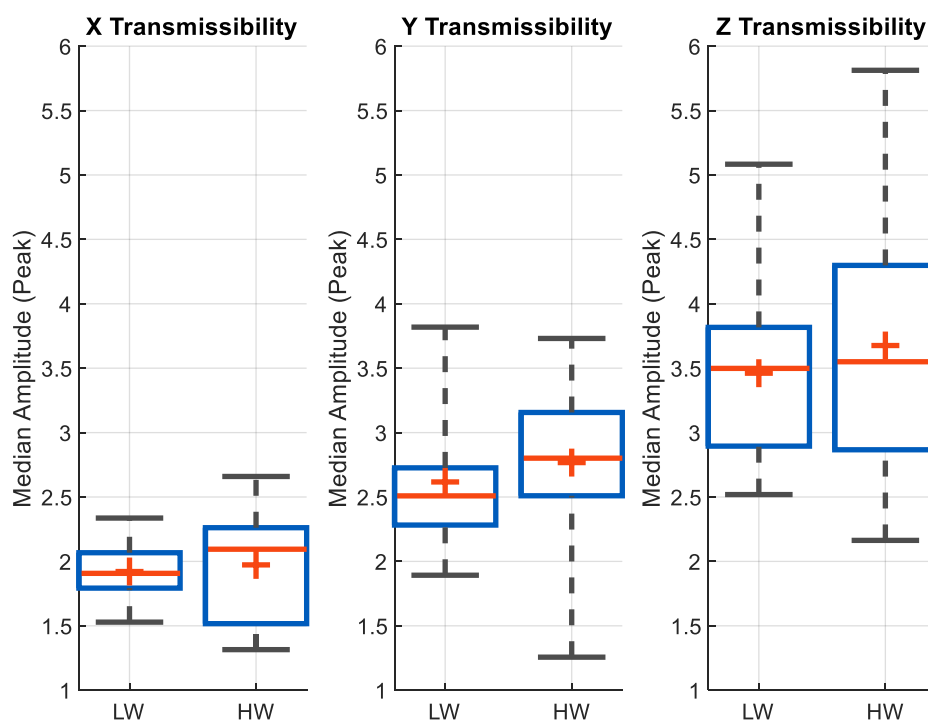
LW and HW boxplots (Hip)
