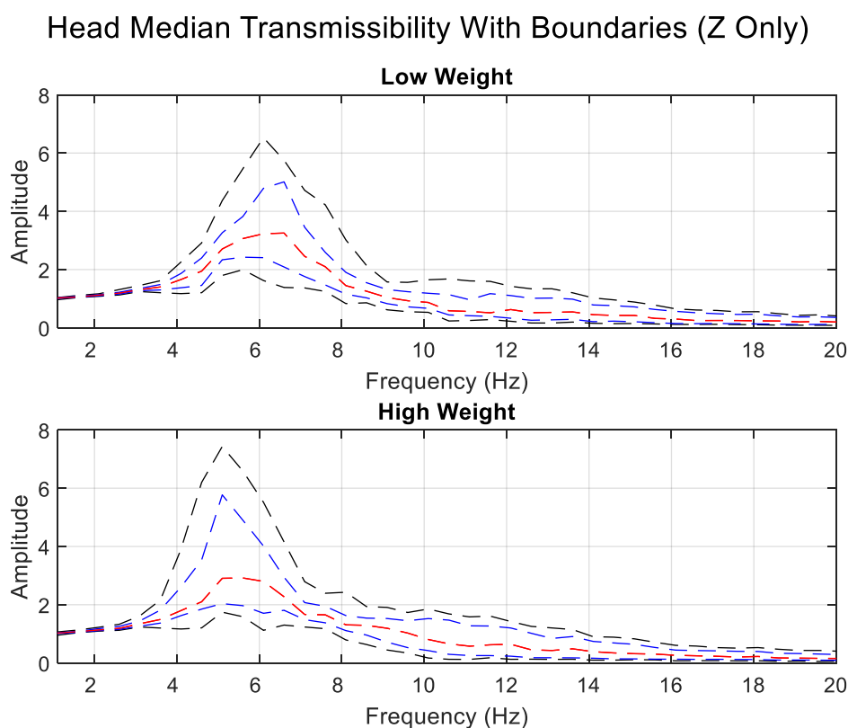
Figure 25: An overlaid transmissibility plot for the head comparing the LW and HW groups. The red line represents the subject median transmissibility, the blue line represents the 25th to 75th percentile, and the black line represents the 5th to 95th percentile
