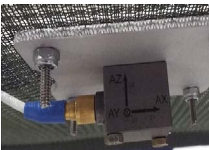
Figure 13. Decon Litter sensor.
