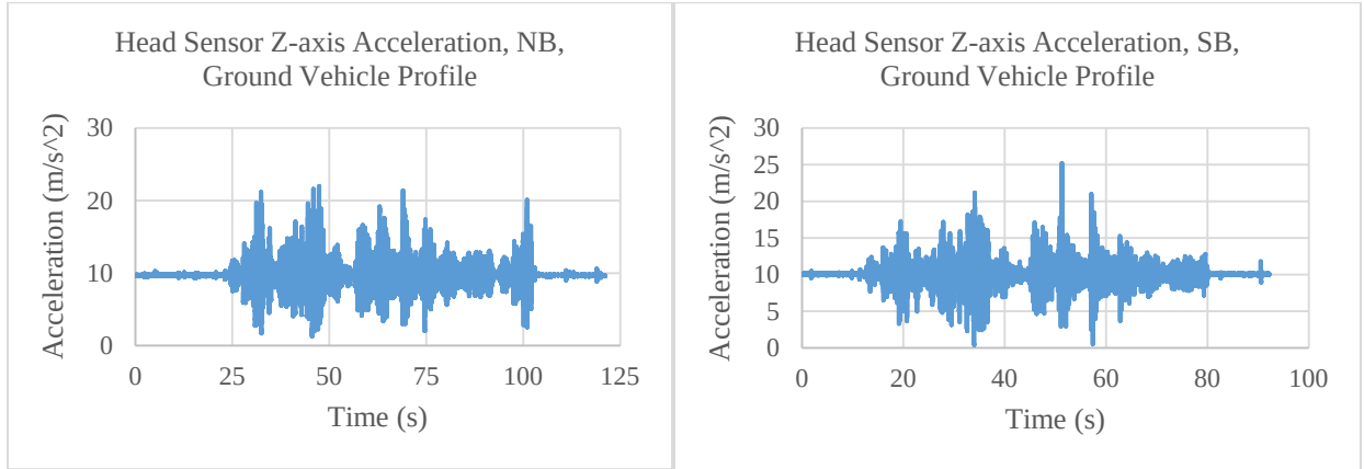
Figure 18. Example z-axis acceleration data for both test configurations.
