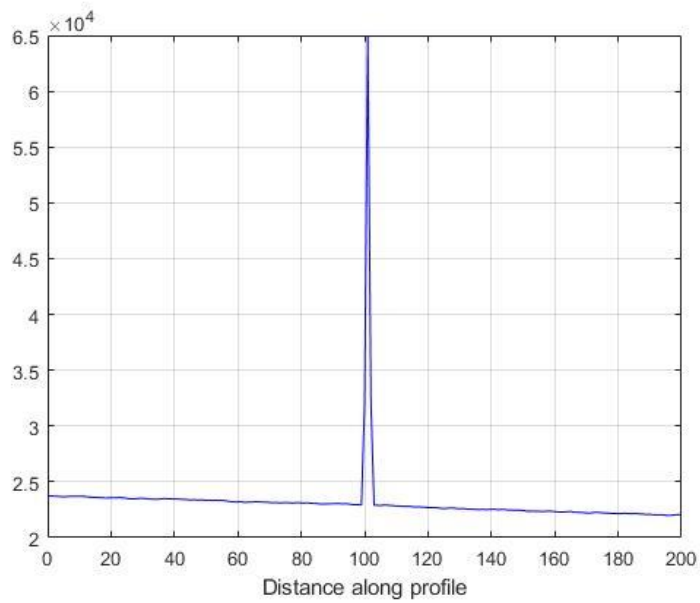
Figure (7A) Line Profile of synthetic crack of width 2, off grid configuration.
