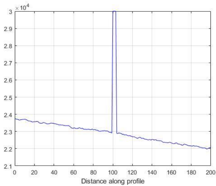
Figure (10A) Line Profile of synthetic crack of width 4, on grid configuration
