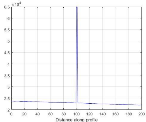
Figure [6] Line Profile of synthetic crack of width 2, in the "on grid" configuration. Gray value is plotted as a function of distance along the line profile.
