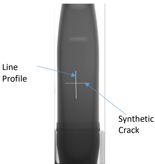
Figure [5] Synthetic Crack of Width 2 in the on grid configuration. A Line profile is shown perpendicular to the synthetic crack.
