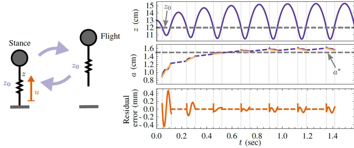
Fig. 4: Averaging the effect of within-step morphological feedback over many steps [DeBu+18]. (left) In this model for vertical hopping, a spring-mass moves vertically in a gravitational field. When the limb extends beyond length z_0 , the model transitions from stance to flight . In stance , the limb exerts viscoelastic and actuator forces on the mass; in flight , the only force is gravity. (right) The cumulative effect of stance forces can be averaged over many steps to obtain a simple proportional-derivative feedback law controlling hopping height. This smooth “averaged” system (in gold) provides a good approximation for the behavior of the original hybrid system (in blue): the trajectories differ by less than 5% of hopping height (top and bottom subfigures), and actuator inputs agree to even greater precision (middle subfigure).
