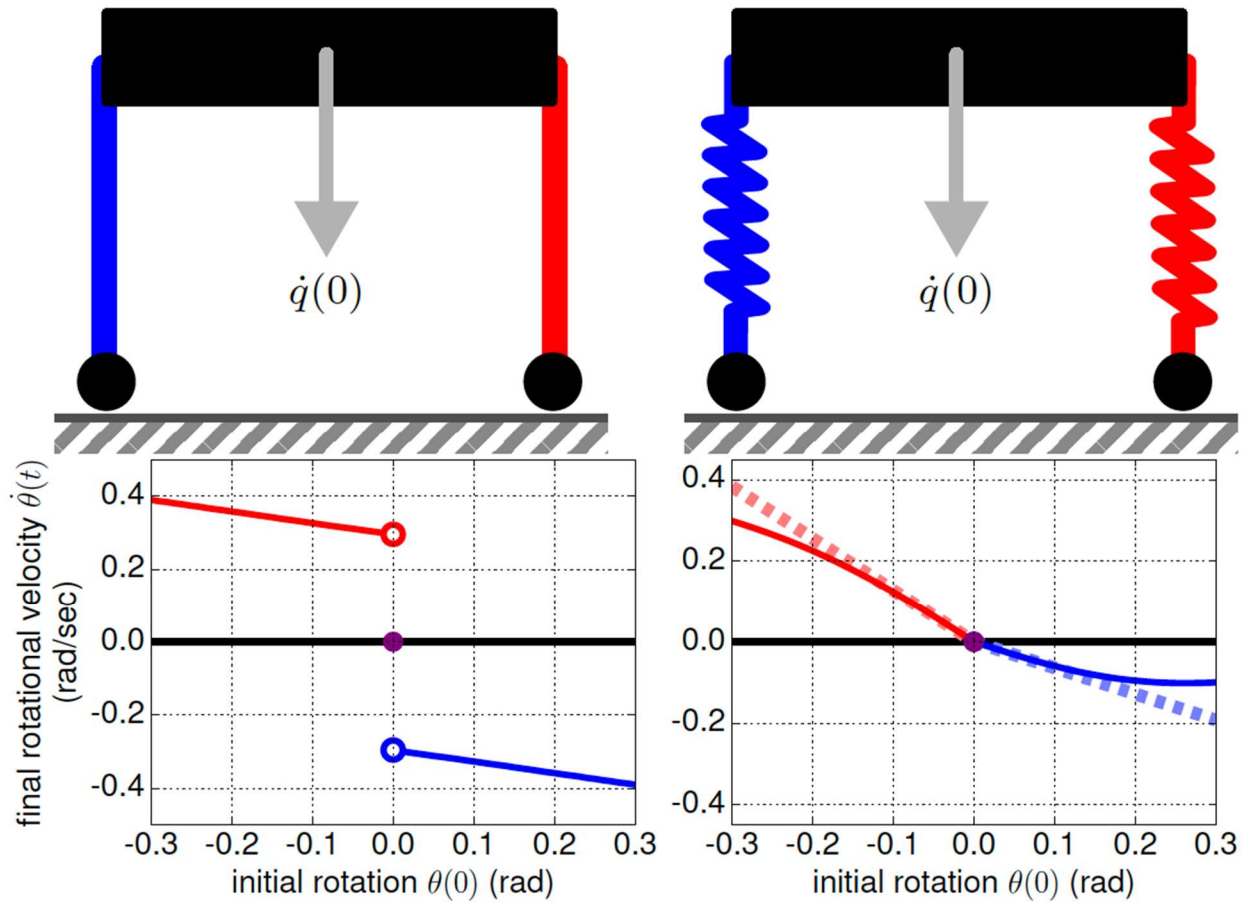
Fig. 3: Trajectory outcomes in mechanical systems subject to unilateral constraints.
