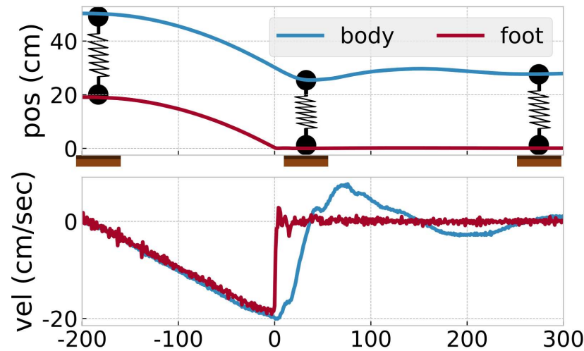
Fig. 1: Schematic, photograph, and impact data from haptic robot testbed constructed in our lab. ( top left ) A single robot leg (from Ghost Robotics' Minitaur) is constrained to move vertically in a gravitational field using a linear rail. A treadmill underfoot presents the robot with variable terrain. A Cable-driven perturbation system enables application of force profiles ranging \pm 2\times robot weight at 80% maximum testbed speed. Onboard motor encoders and accelerometers record data at 1kHz; a high-speed motion capture camera records data at 1kHz. ( top right ) Photograph of testbed prototype. ( bottom ) Sample data collected on testbed showing position and velocity traces in 500msec window around impact.
