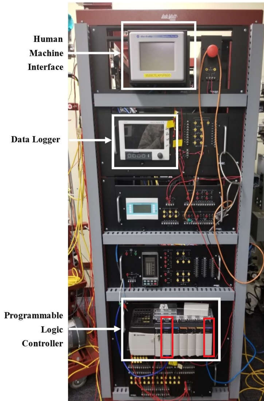
Figure 18. Lab-Volt 3531's Computing Cart.
