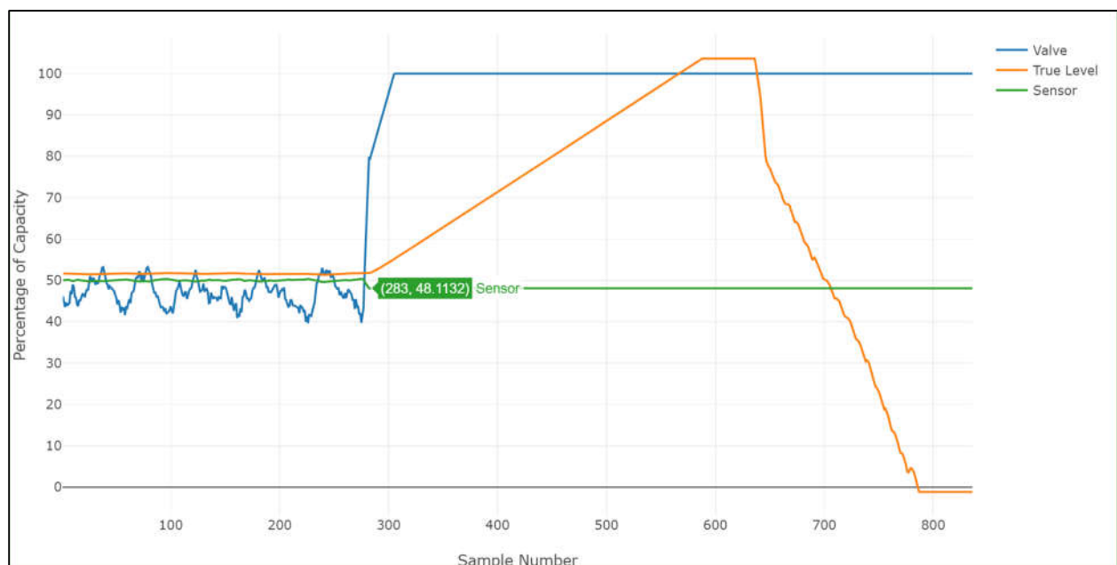
Figure 35. Overpressure Outcome.
