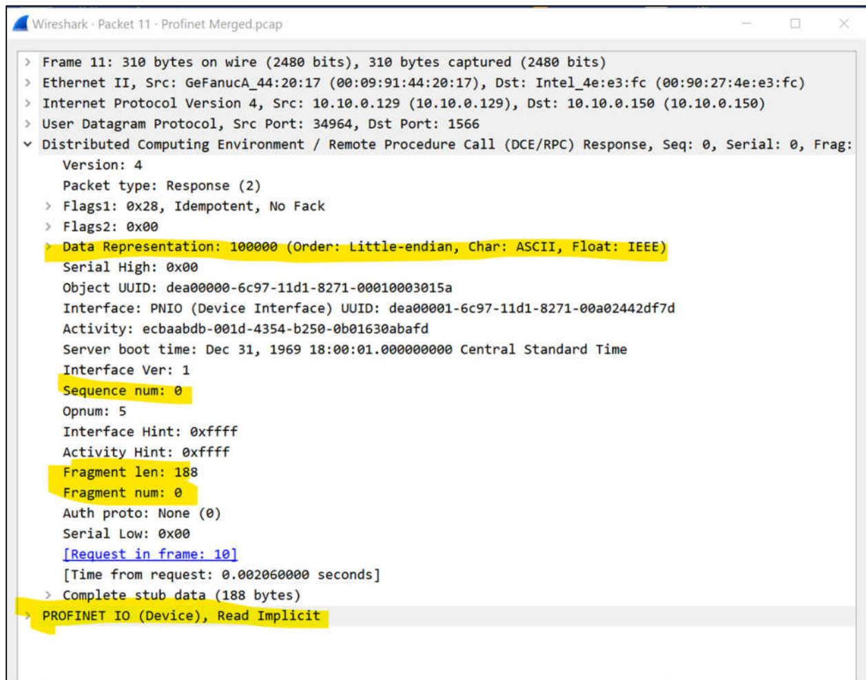
Figure 12. Distributed Computing Environment Protocol Example [21].
