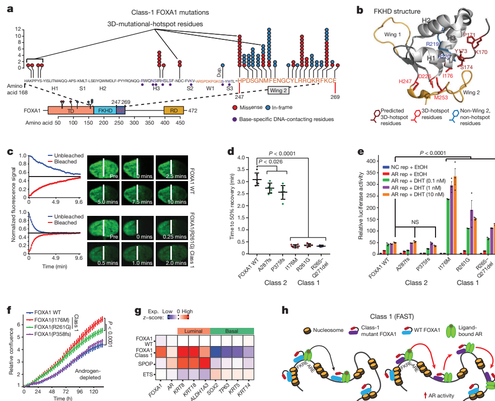
Fig. 2 | Functional characterization of class-1 mutations of FOXA1.
