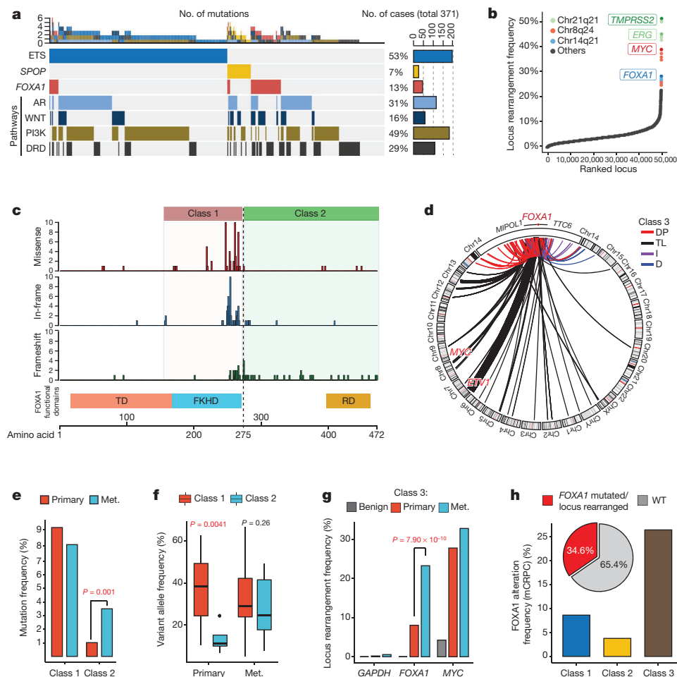
Fig. 1 | Structural classes of FOXA1 alterations. a , FOXA1 mutations and key alterations in mCRPC. Alterations in ETS, AR, WNT, PI3K and DNA repair (DRD) were aggregated at the pathway or group level. b , Locus-level recurrence of RNA-seq structural variations. c , Structural classification of FOXA1 mutations. TD, transactivation domain; RD, regulatory domain. d , Structural classification of FOXA1 locus rearrangements. DP, tandem duplications; TL, translocations; I, inversions; D, deletions. e , Frequency of FOXA1 mutational classes by prostate cancer stage ( n = 888 primary,
