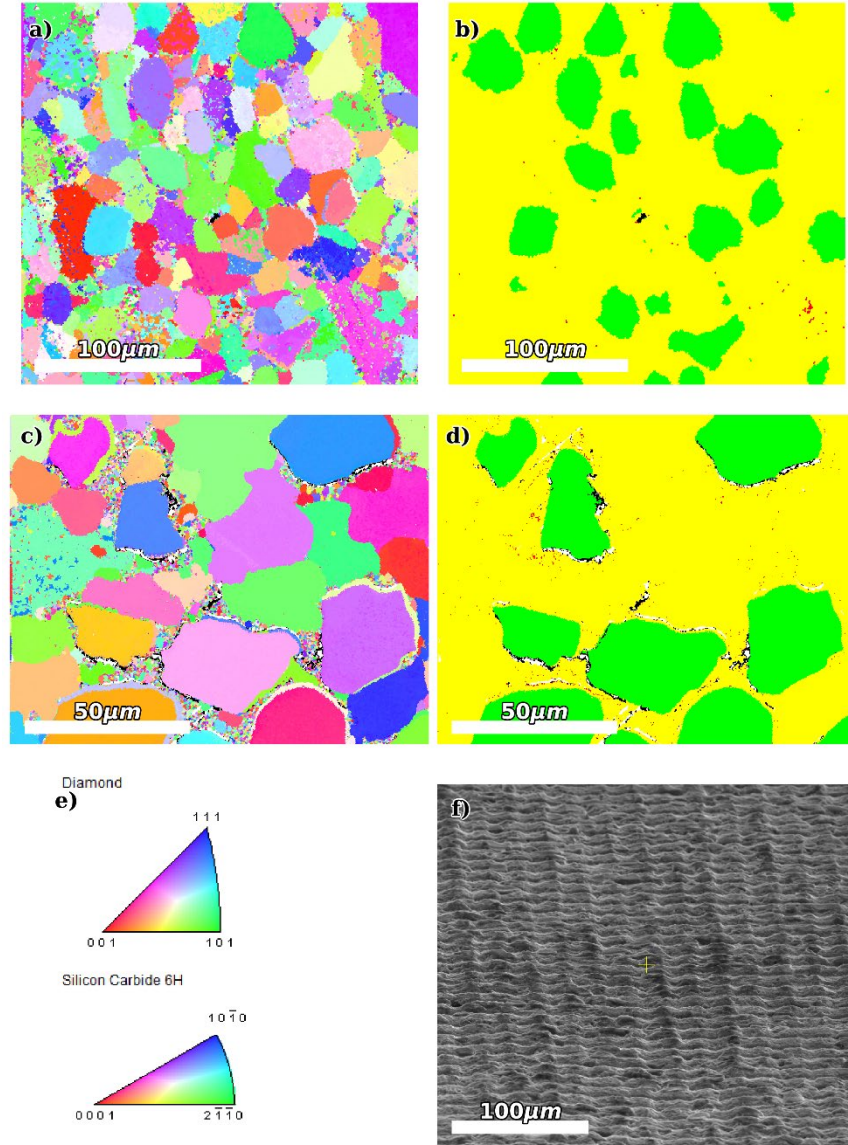
Fig. 4 EBSD results for the polishing methods, (a–e). Only the mechanical polish and ion polished surfaces were capable of providing EBSD data. The laser polished surface (f) is too rough, which blocks any diffracted beam from the camera.
