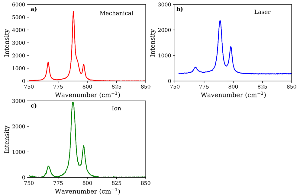
Fig. 3 Raman spectra in the range of 750–850 \text{cm}^{-1} for all three polishing methods: a) mechanical, b) laser, and c) ion. All show the expected SiC peaks without any major shifts in peak position.
