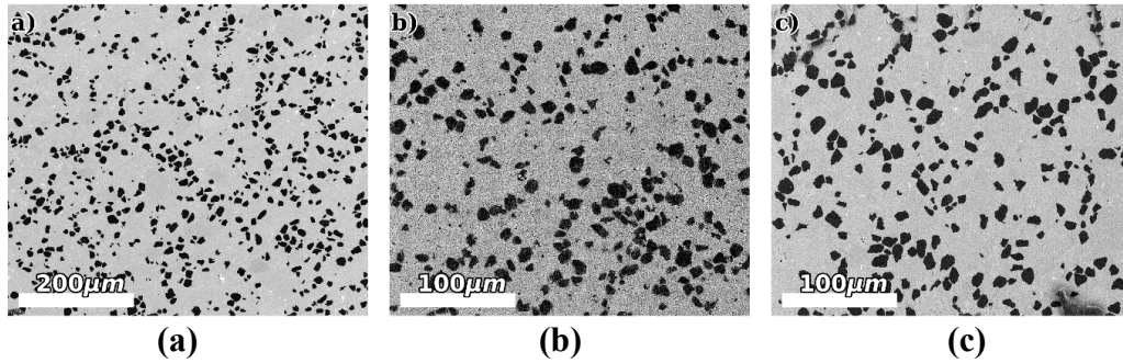
Fig. 1 Backscatter SEM images from surfaces polished using the a) scaife process, b) femtosecond laser, and c) broad-beam ion polisher. The darker phases are the diamond particles.
