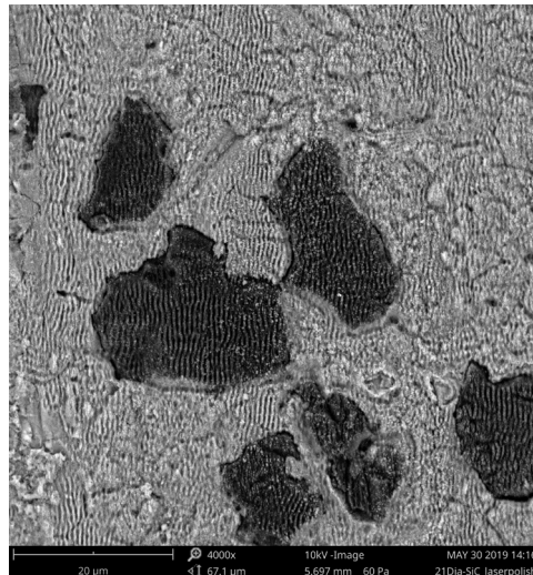
Fig. 2 Backscatter SEM image from the femtosecond laser-polished sample showing the presence of LIPSSs in both phases
