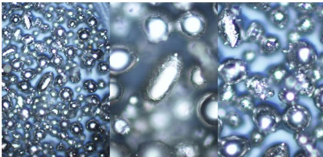
Figure 4 Optical Microscopic Images of the Inconel Powder with different magnification
