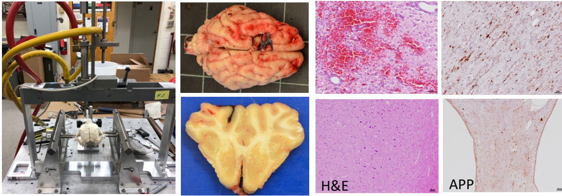
Fig.2 New CCI injury at 72 hours post injury. More appropriate biomechanics of the contusion injury lead to subdural, subarachnoid, and intraparenchymal hemorrhage. Compression of the cortical gyrus is visible, as well as a partial midline shift at this level. H&E demonstrates intraparenchymal hemorrhage as well as pyknotic neurons in adjacent gyri. Axonal pathology extends beyond the level of the blood brain barrier breakdown, suggesting primary biomechanical injury of the white matter. This extends into the collosum and fimbria fornix, suggesting that this injury may be primarily focal but with a diffuse component, replicating important aspects of human injury/contusion. An animal with this injury has now been implanted with both a surface grid and a hippocampal depth.
