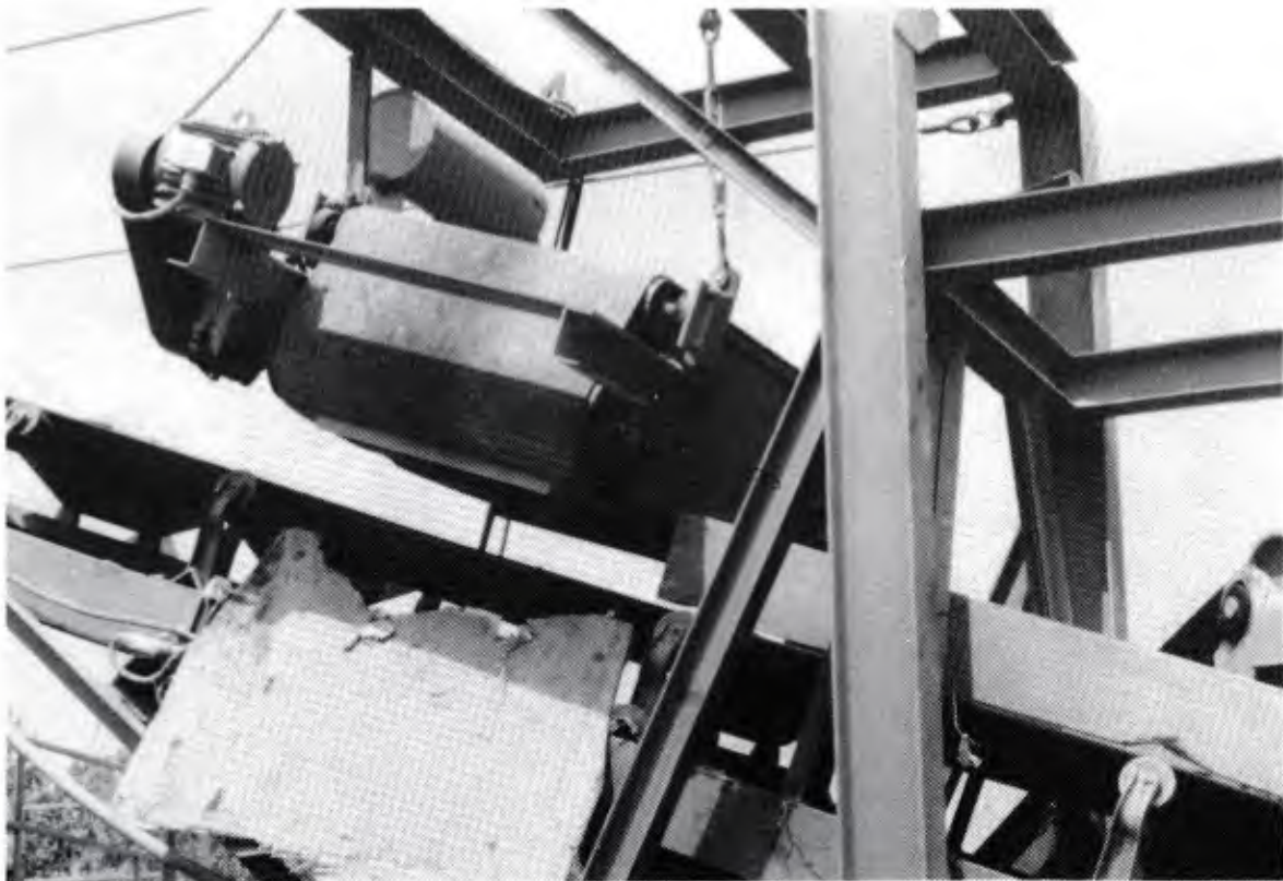
FIGURE 7. ELECTROMAGNET USED TO REMOVE REINFORCING STEEL FROM THE CONVEYOR BELT.
