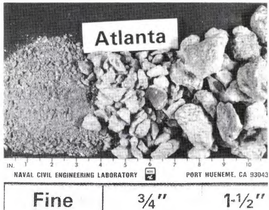
FIGURE 10. PRODUCTS FROM THE CRUSHING OF THE PCC SAMPLE FROM ATLANTA.
