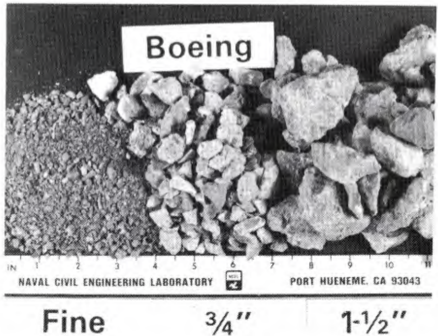
FIGURE 11. PRODUCTS FROM THE CRUSHING OF THE PCC SAMPLE FOR BOEING FIELD.
