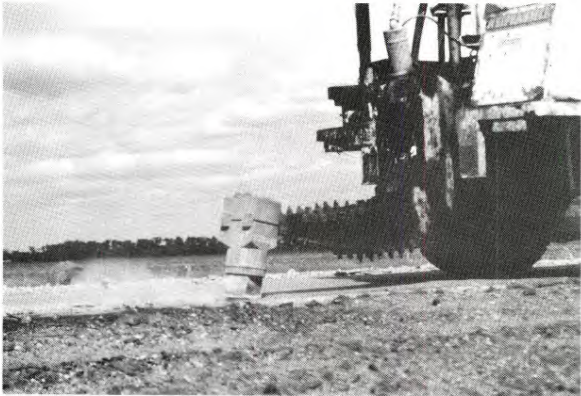
FIGURE 5. CLOSEUP OF THE IMPACT HEAD OF THE LEAF-SPRING WHIPARM HAMMER PAVEMENT BREAKER.
