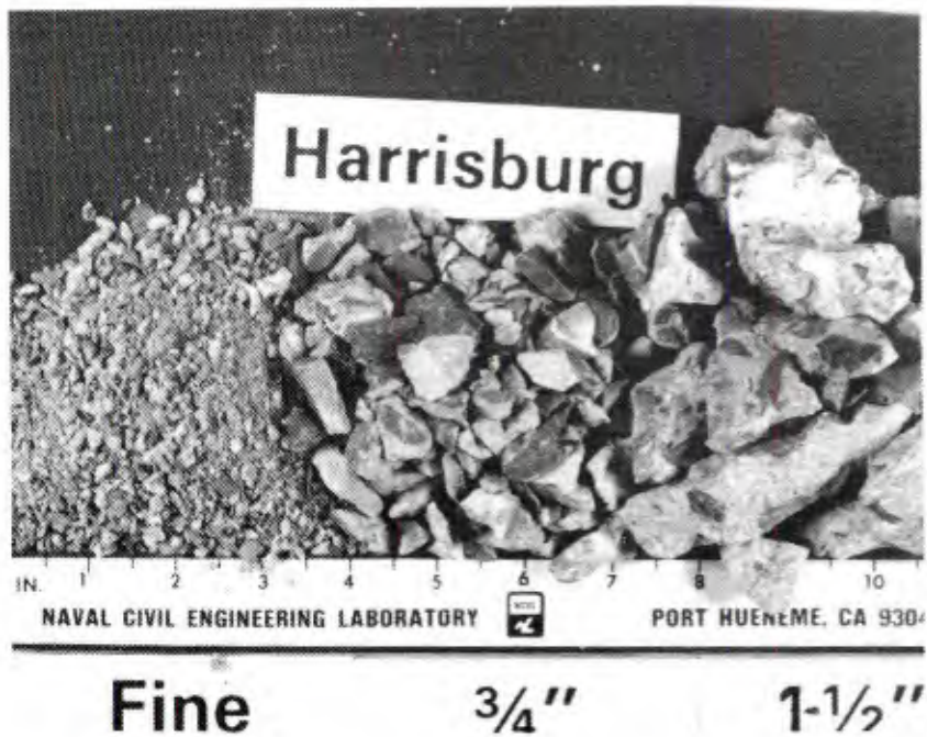
FIGURE 13. PRODUCTS FROM THE CRUSHING OF THE PCC SAMPLE FROM HARRISBURG.
