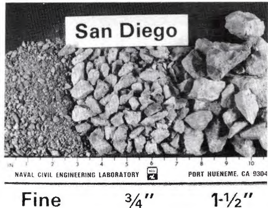
FIGURE 15. PRODUCTS FROM THE CRUSHING OF THE PCC SAMPLE FROM SAN DIEGO.
