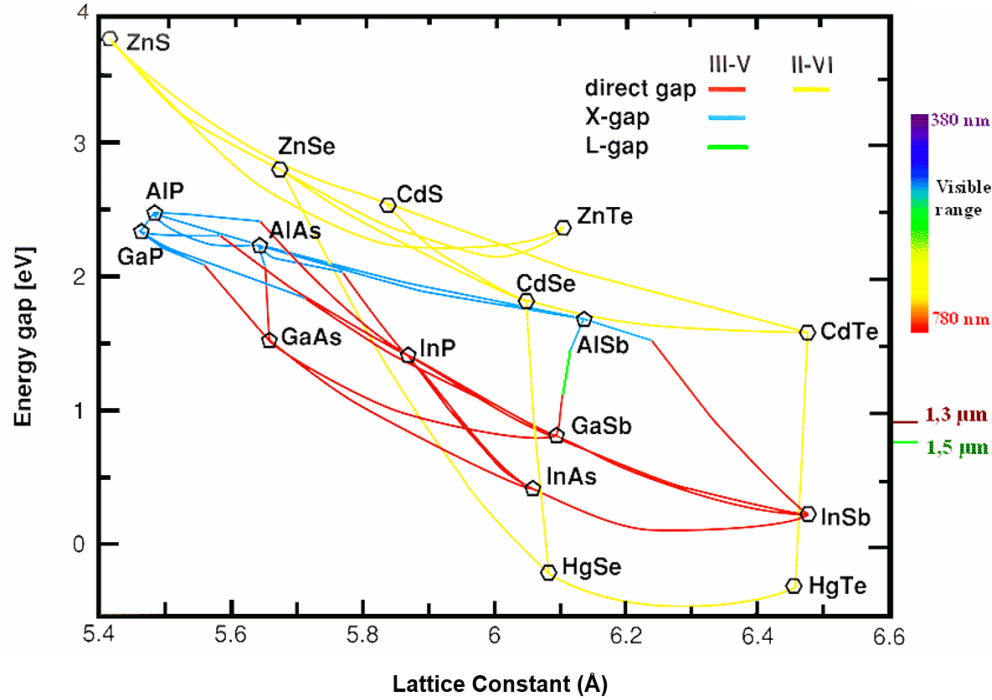
Figure 2-8: Graph of energy gap (eV) as a function of lattice constant (Å) for III-V and II-VI binary semiconductors. Wavelengths corresponding to energy gaps are displayed on the right axis [13].
