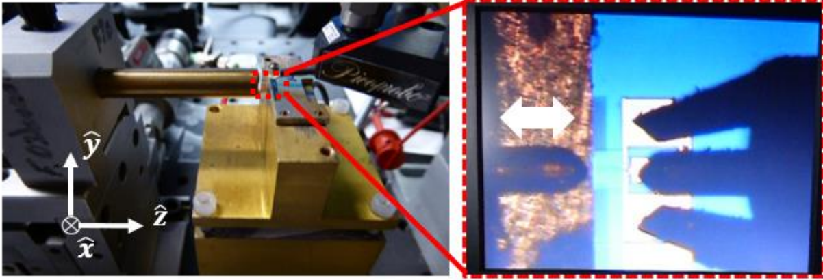
Figure 4-9: (Insert) The optical fiber up against a 25- \mu\text{m} device, and the cavity of air between them (not visible).
