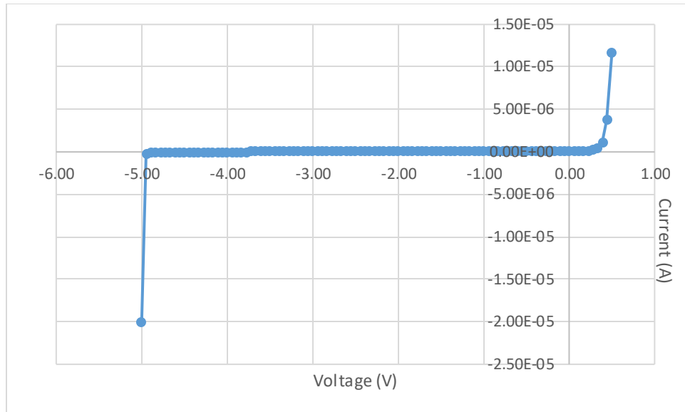
Figure 4-2: An example of the IV response of a 25- \mu\text{m}^2 device.
