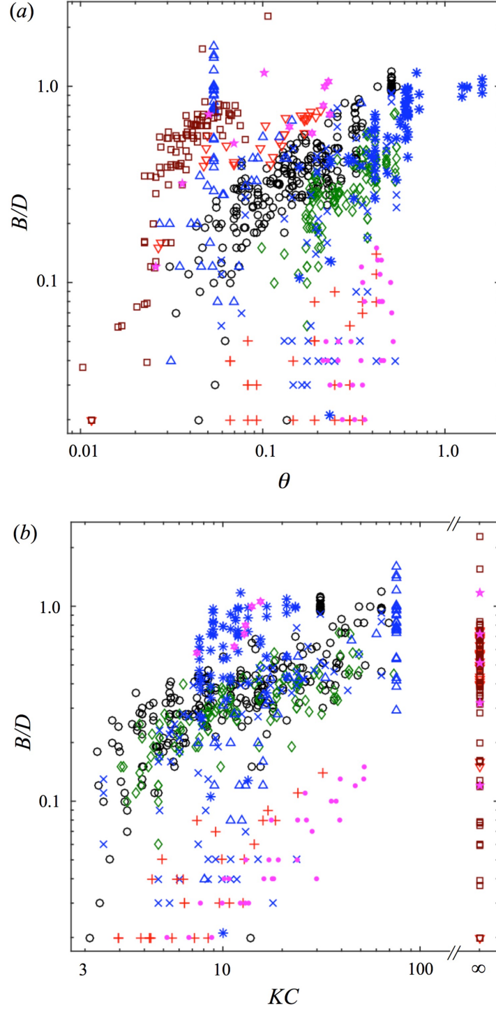
Figure 3. All observations of B/D plotted as a function of (a) \theta and (b) KC . Cylinders with waves plus currents in the field = * (all others are lab measurements); cylinders with \alpha < 60^\circ = \times (all others have \alpha \geq 60^\circ ); cylinders with D < 2.6 cm for waves only = \triangle and for currents only = \square (all other objects have D \geq 3.0 cm); other cylinders and spheres with currents only = \nabla ; cylinders with waves plus currents = \diamond ; cylinders and spheres with waves only = \circ ; conical frustums with waves only = + ; conical frustums with waves plus currents = \bullet ; tapered cylinders with waves only = \star ; tapered cylinders with currents only = \star .
