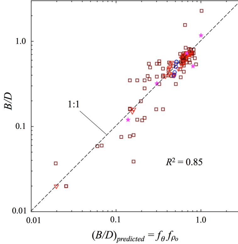
Figure 6. All available observations of B/D for currents in the absence of waves, plotted as a function the final parameterized model for B/D under steady flow, (B/D)_{\text{predicted}} = f_{\theta} f_{\rho_0} . Symbols are as in Fig. 4. The formulations and coefficients for f_{\theta} and f_{\rho_0} are provided in Fig. 4 and Fig. 5. To calculate f_{\theta} for \star , the coefficients for \nabla and \square were used for \theta less than and greater than 0.04, respectively. (Cases with U_w > 0 , e.g., the field cases in Tables 1 and 2, are not included in Figs. 4, 5 or 6.)
