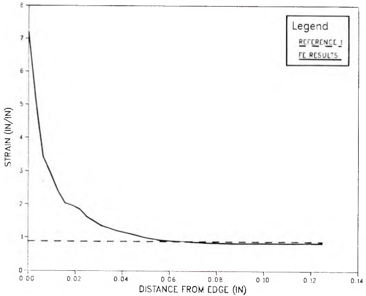
Figure 24. Strains on free surface of a 1/2-inch deep by 1/4-inch wide pavement seal subjected to 50% extension.
