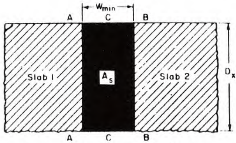
Sealed Joint of Minimum Width
