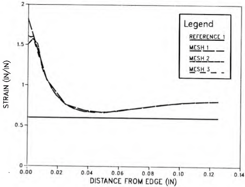
Figure 16. Strains at 0.00625 inches below the surface for various finite element meshes of a 1/4- by 1/4-inch seal subjected to a 50% extension.
