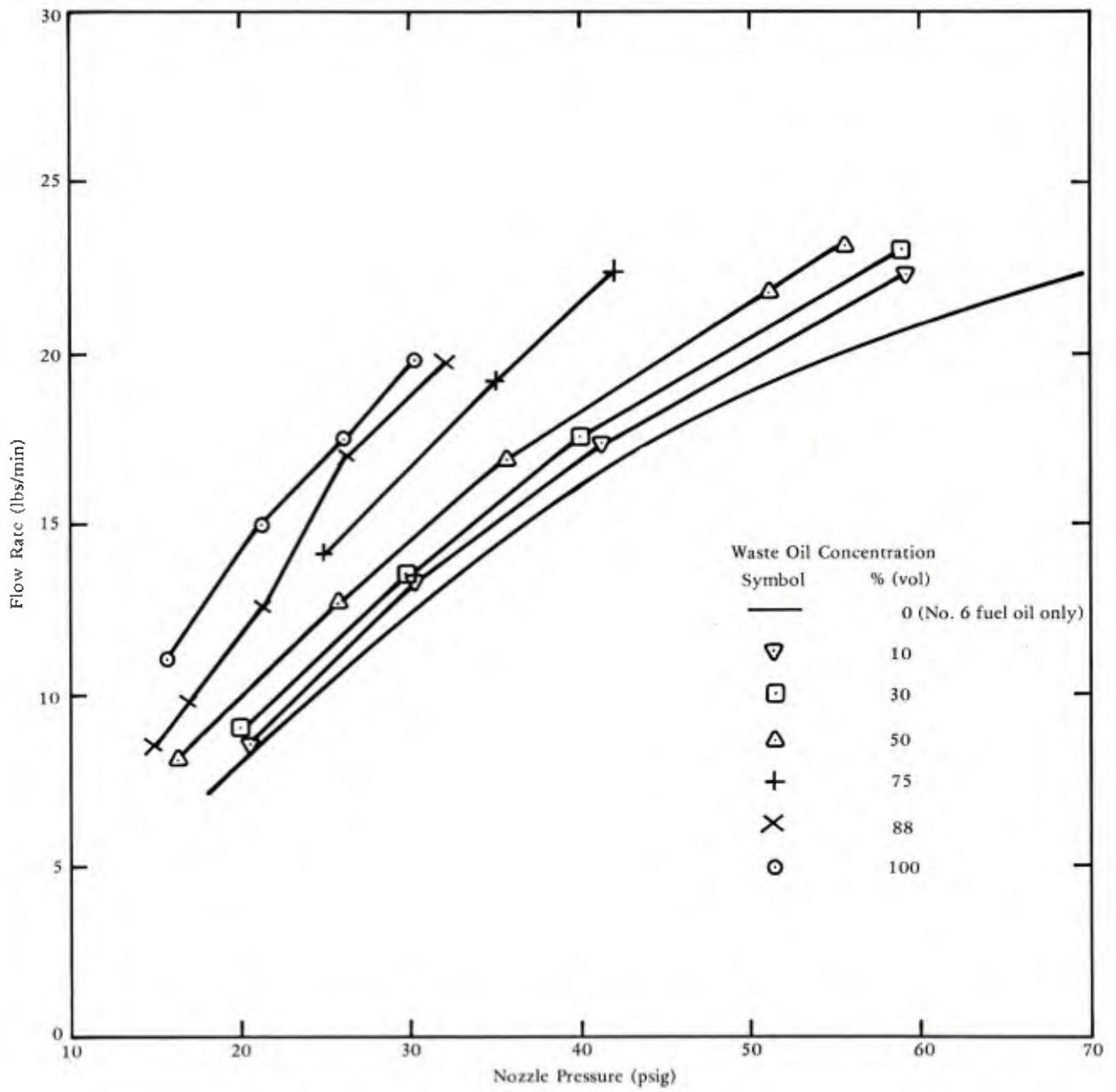
Figure 3. Fuel flow rate.
