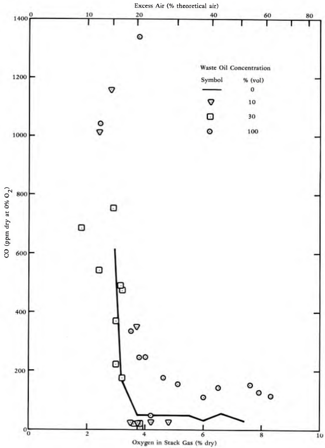
Figure 6. Carbon monoxide emissions.
