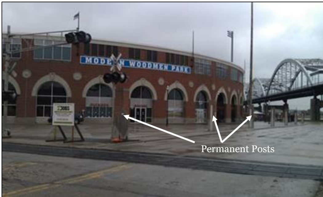
Figure 7. Combination wall in Davenport, IA, before deployment.
