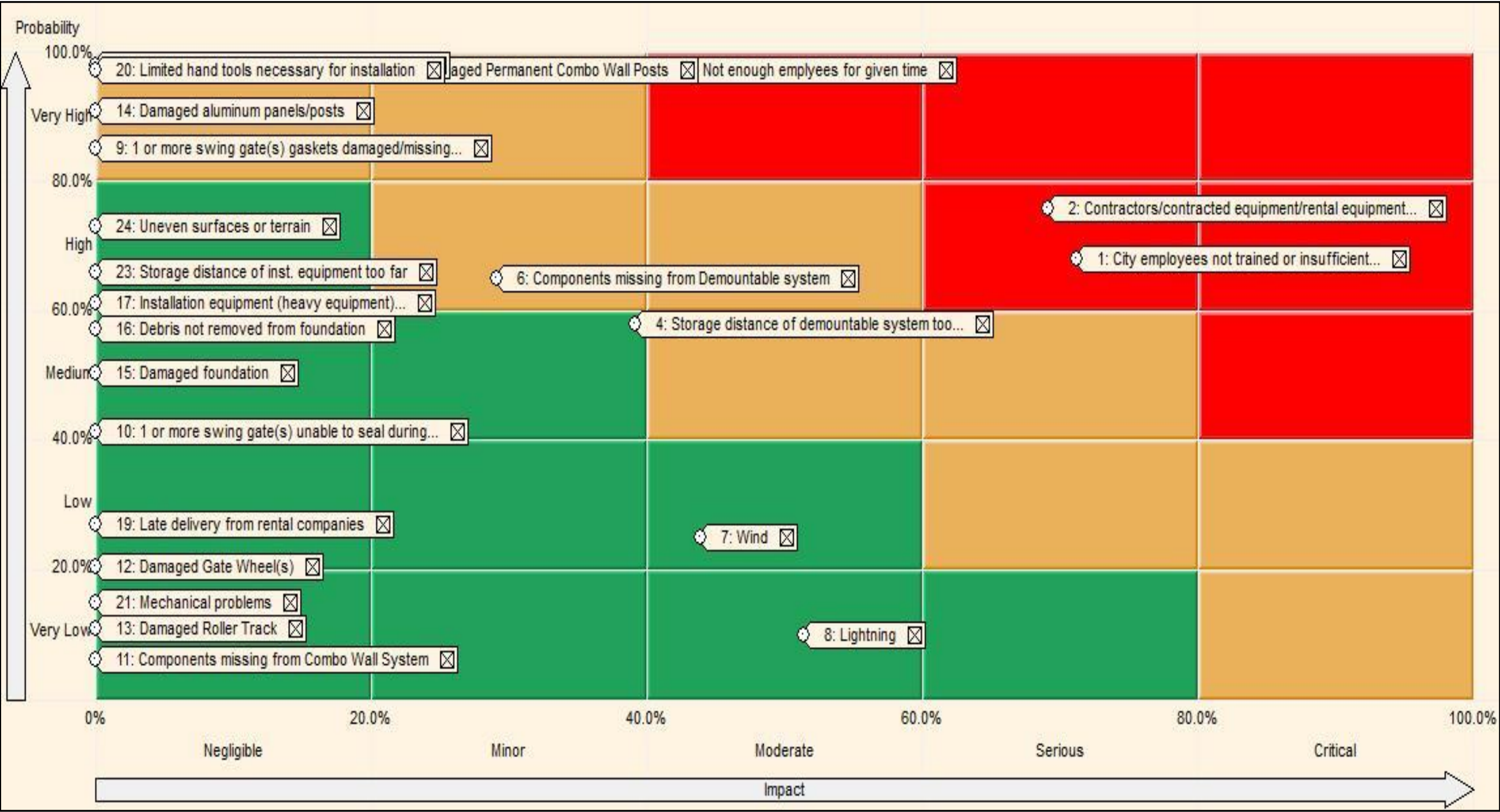
Figure E-5. Phase 1, Master Plan Minus 400 ft risk matrix.
