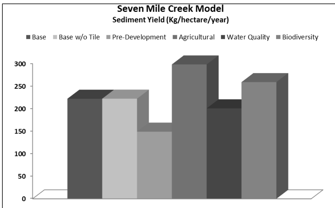
Figure 42. Annual sediment yields associated with the various land uses.
