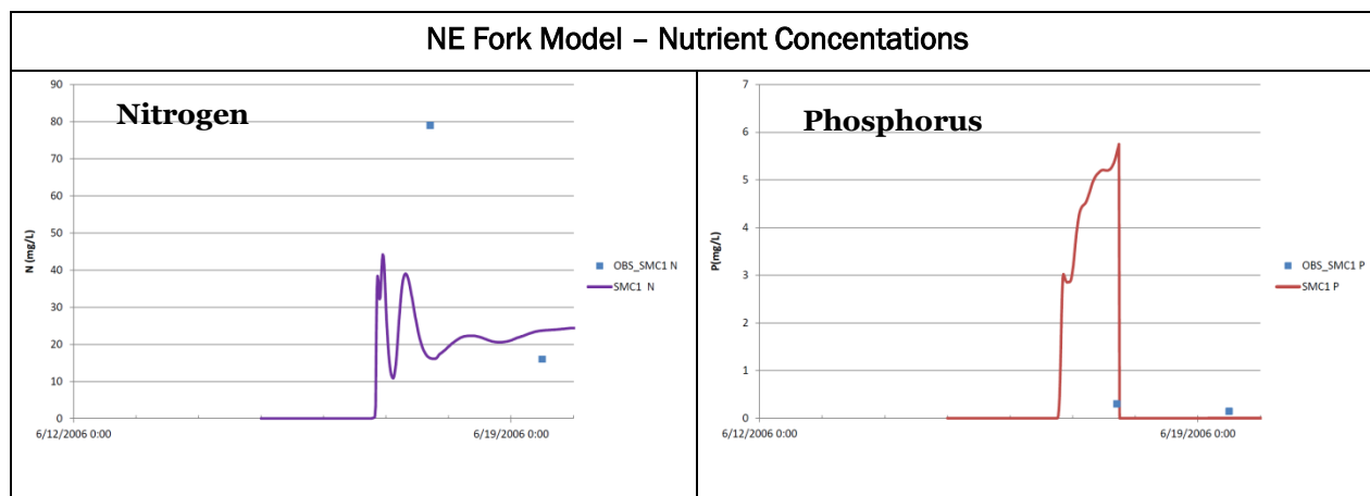
Figure 28. Nutrient concentrations at the outlet of the NE Fork for June 2006 event.
