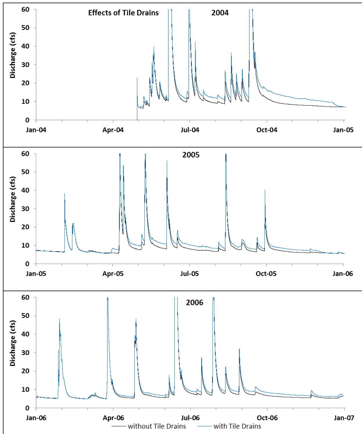
Figure 43. Comparison of outflow at Seven Mile Creek between simulated flow with and without tile drains.
