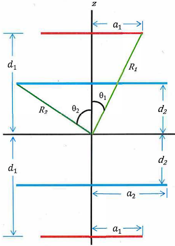
Figure 11. Fanselau coil geometry diagram
