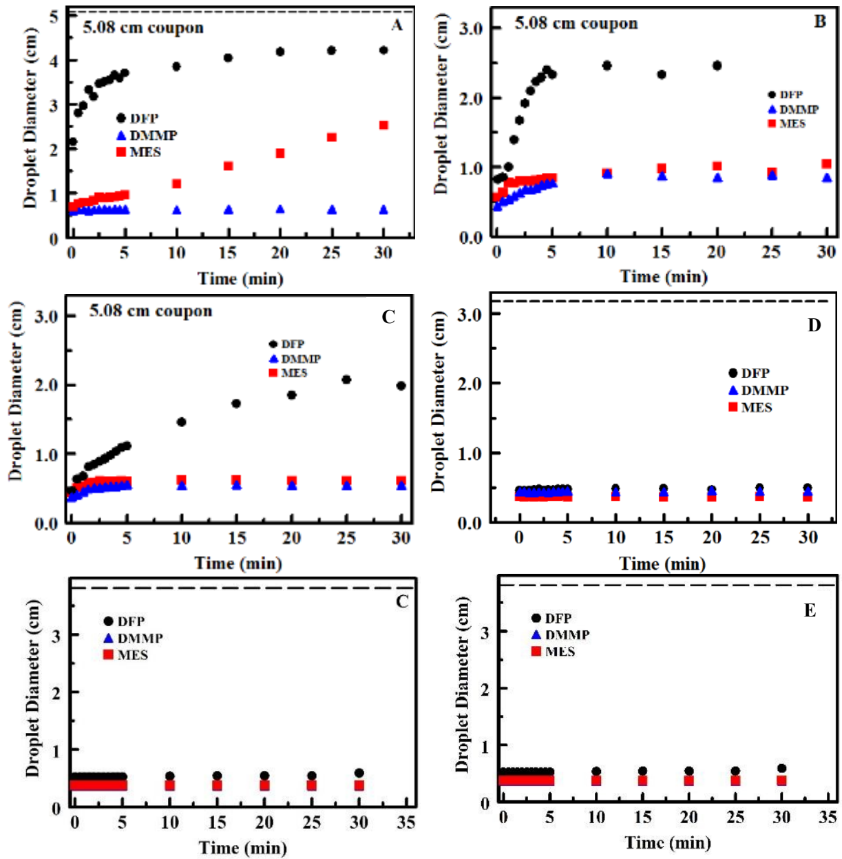
Fig. 4 — Droplet diameters over time following exposure to DFP (black), MES (red), and DMMP (blue) for a painted coupon (A), a painted coupon oiled with Fomblin Y (B), a painted coupon with a smooth fluoropolymer coating (C), and a painted coupon with the thick AVIRAL coating (D) and a painted coupon with the INVESIL coating (E).
