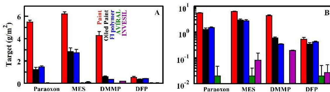
Fig. 5 — Target retention by coupons following treatment with an air stream and rinsing with soapy water: paint (red), oiled paint (black), smooth fluorinated polymer (blue), the AVIRAL coating (green), and the INVESIL coating (purple) plotted on a linear (A) and a log scale (B).
