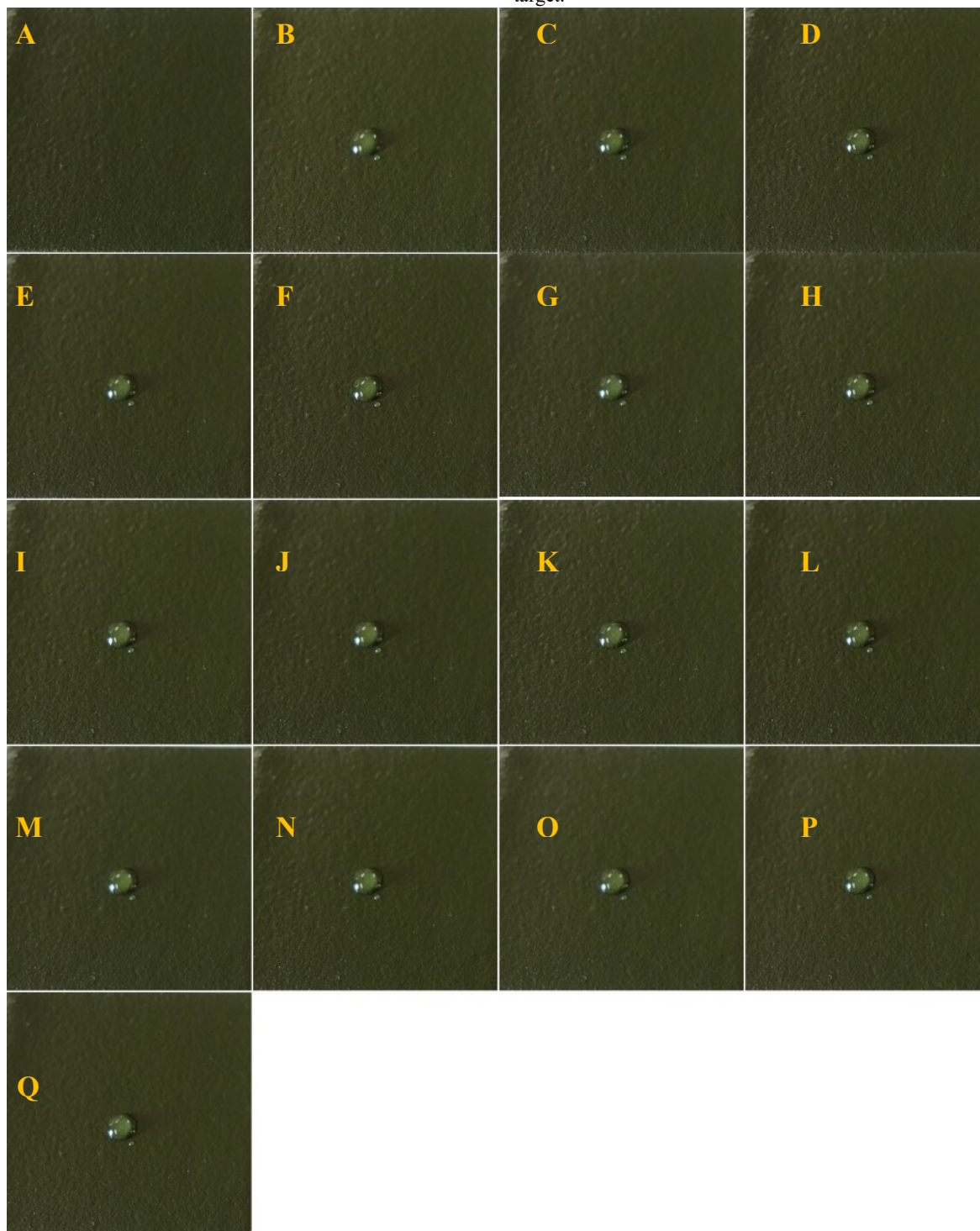
Fig. E3 — DMMP on thin INVESIL coating. Images of a coupon before application (A) and at 0 (B), 0.5 (C), 1 (D), 1.5 (E), 2 (F), 2.5 (G), 3 (H), 3.5 (I), 4 (J), 4.5 (K), 5 (L), 10 (M), 15 (N), 20 (O), 25 (P), and 30 (Q) min following application of the target.
