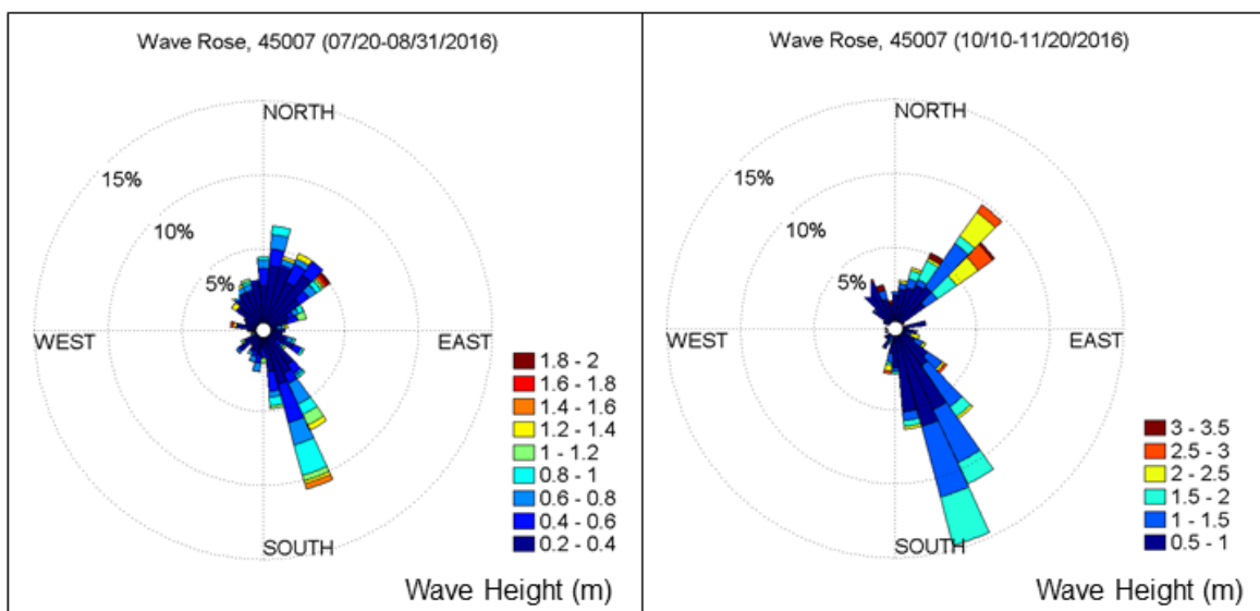
Figure 23. Wave roses for 7/20/2016 to 8/31/2016, and 10/10/2016 to 11/20/2016, at NDBC Buoy 45007.
