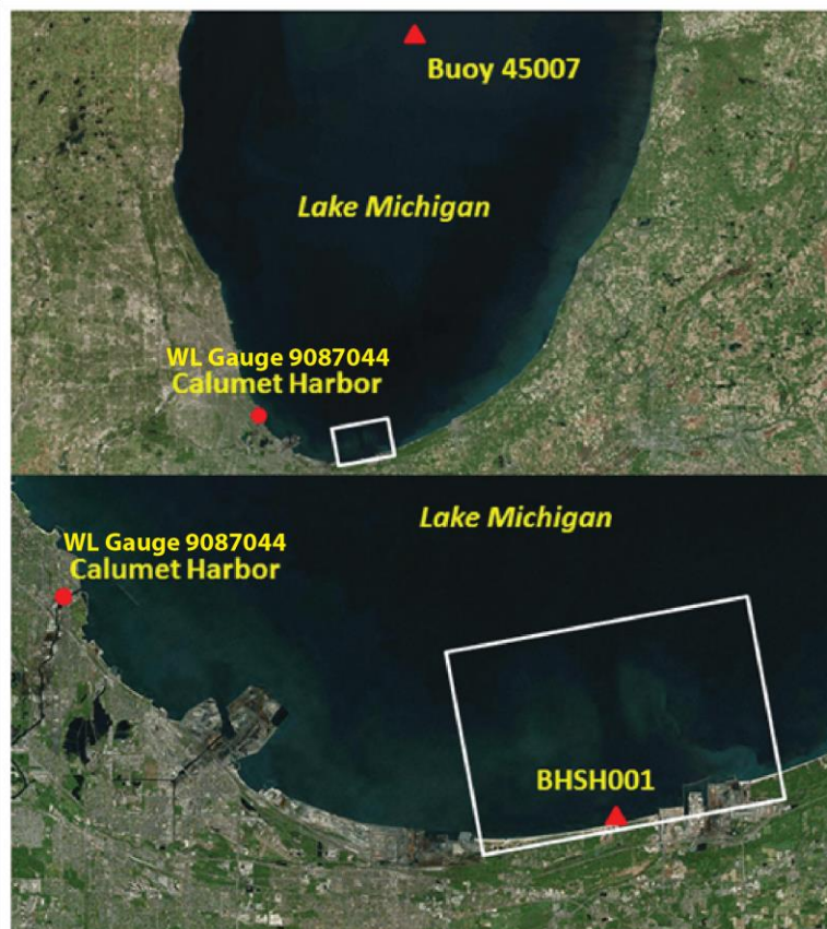
Figure 19. Locations of Lake Michigan water level gauge 9087044 (Calumet Harbor, Illinois), NOAA buoy 45007 and the up-looking ADCP (BHSH001) site. The white rectangle designates the CMS domain.
