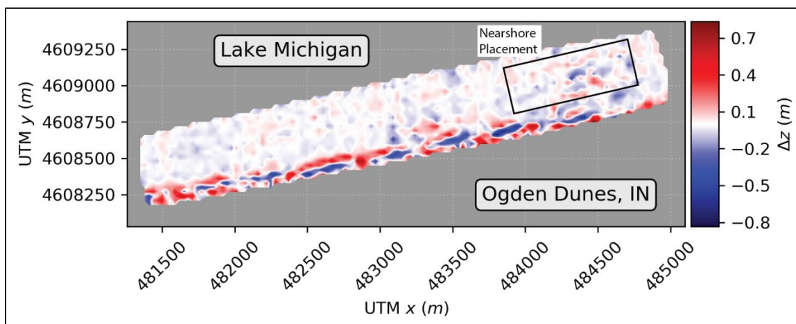
Figure 54. Elevation difference between the adjusted 11/15/2016 ADCP survey DEM and the 10/11/2016 ADCP survey DEM ( \Delta z = \text{adjusted } 11/15/2016 \text{ } z - 10/11/2016 \text{ } z ).
