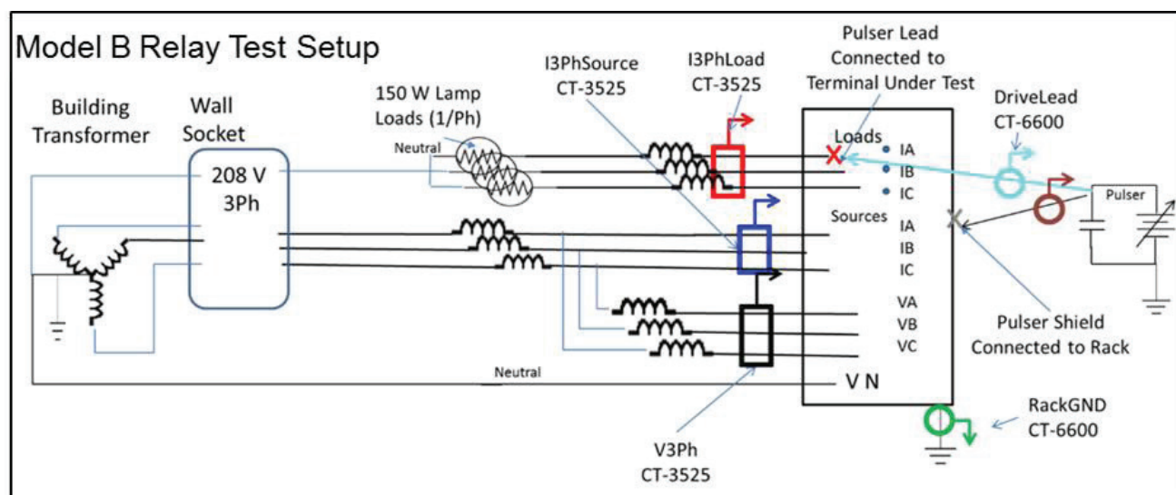
Figure 11. Typical PCI measurement points and injection connection for an unhardened DCS protective relay. (Note the inductive isolation.)
