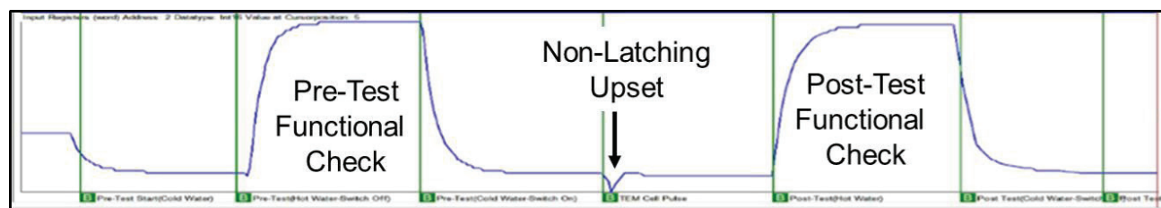
Figure 15. The non-latching upset observed during TEM BWTL testing.
