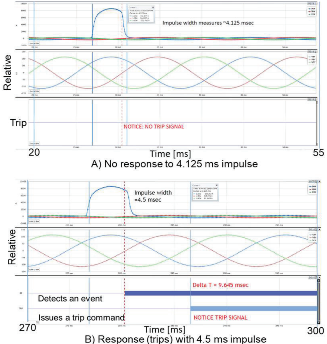
Figure 12. Model-A response to short impulses.
