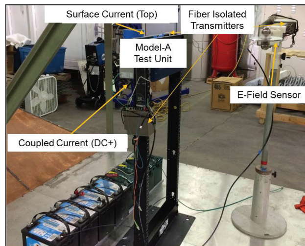
Figure 7. Unprotected-open-rack, protective relay test configuration.
