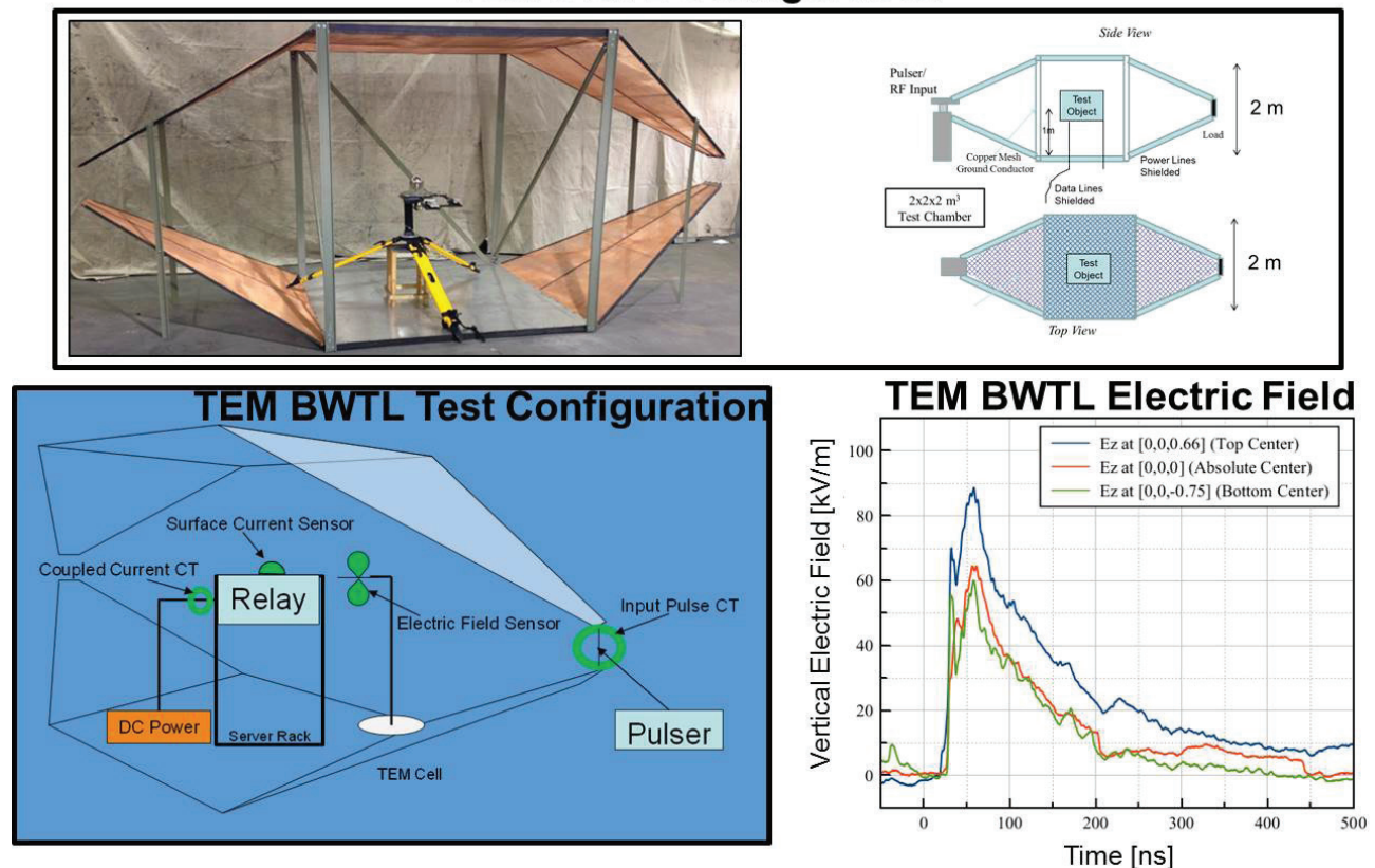
Figure 2. TEM BWTL for DCS protective relay testing.
