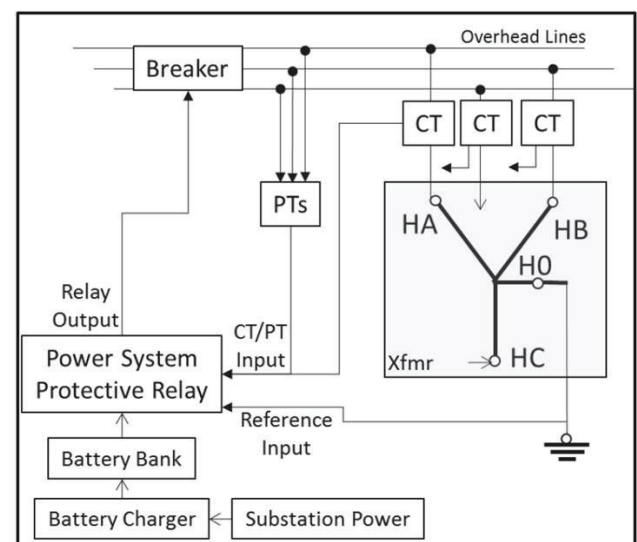
Figure 10. How protective relays are used typically in the power grid.
