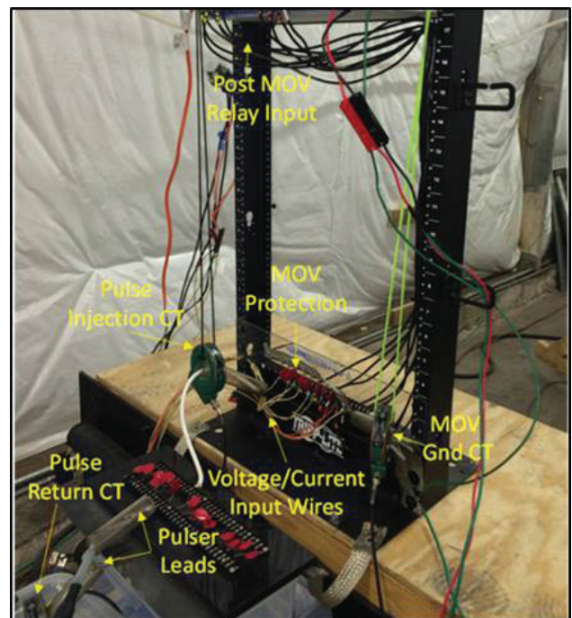
Figure 4. The EMP, open-rack-protected configuration for protective relays seen during PCI testing.
