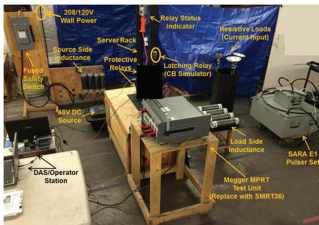
Figure 8. PCI test configuration.
