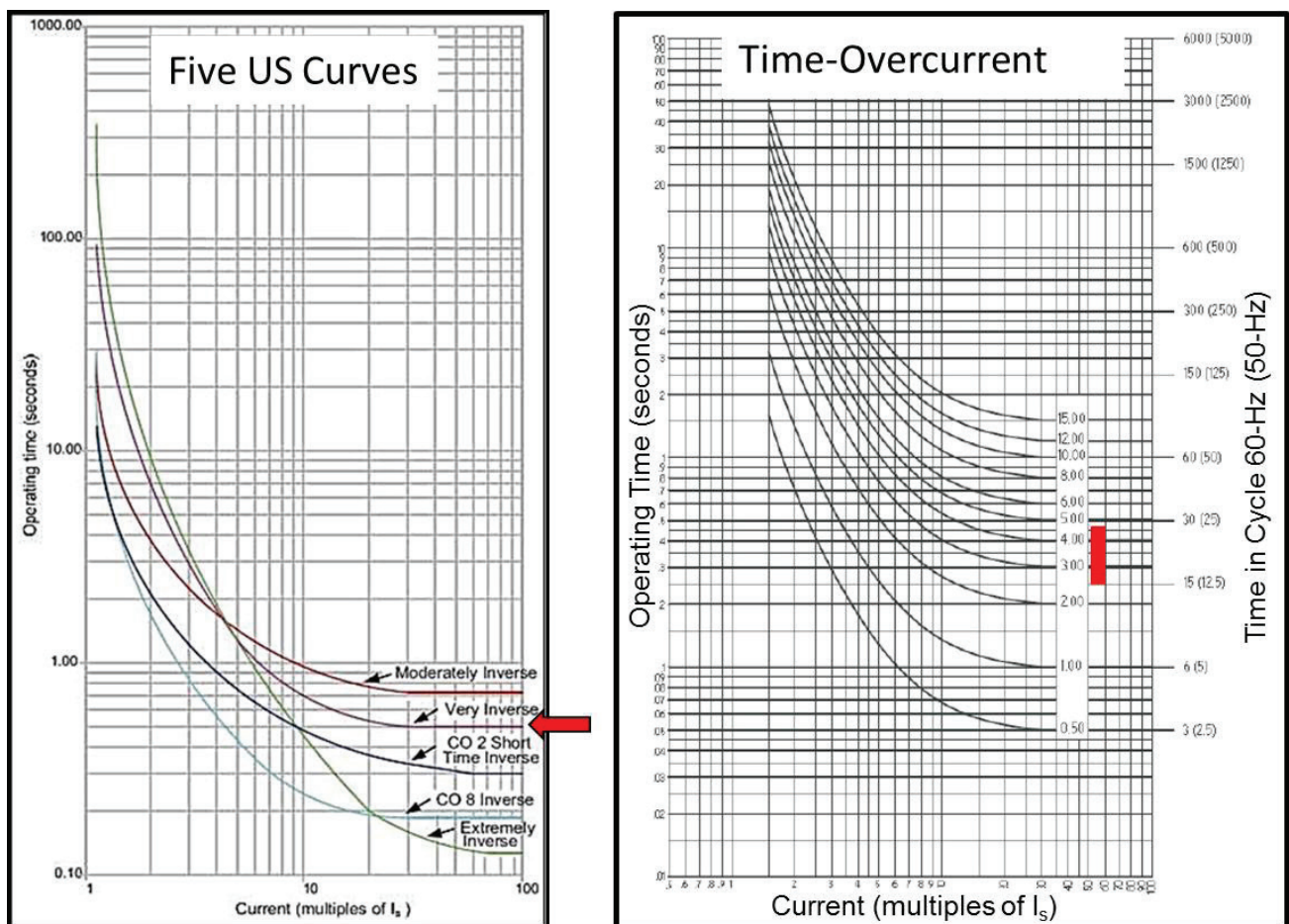
Figure 6. Time overcurrent curves.
