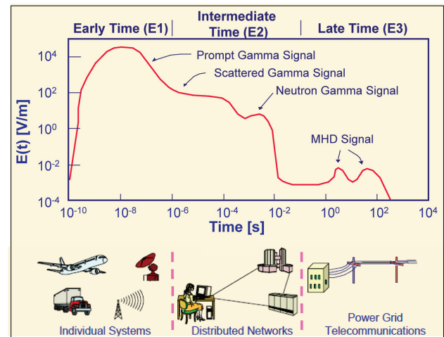
Figure 1. HEMP generic waveform.
