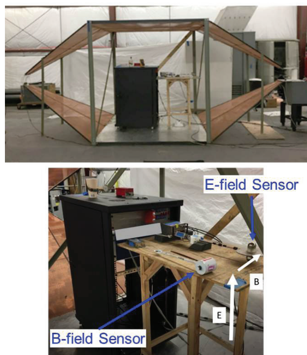
Figure 14. TEM BWTL test of the Model-PGP-A in the front orientation.
