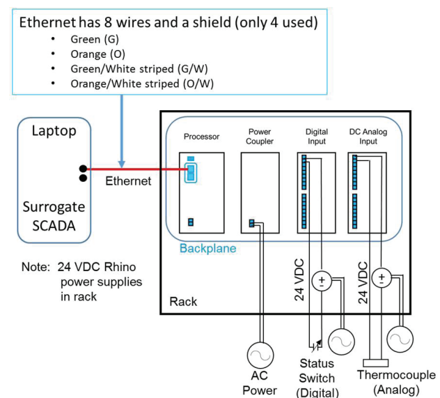
Figure 13. Model-PGP-A unprotected test configuration.
