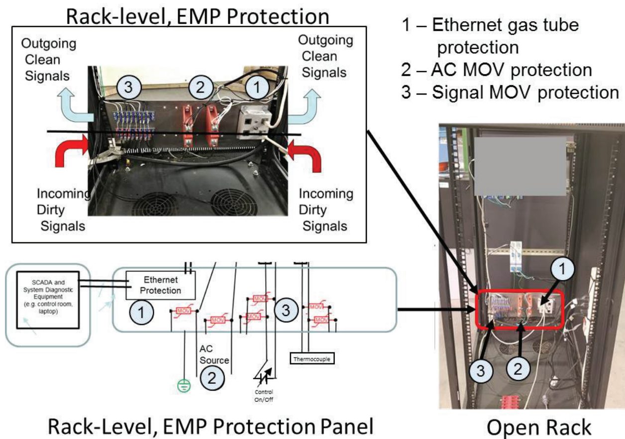
Figure 5. The EMP, open-rack-protected configuration for PGP.
