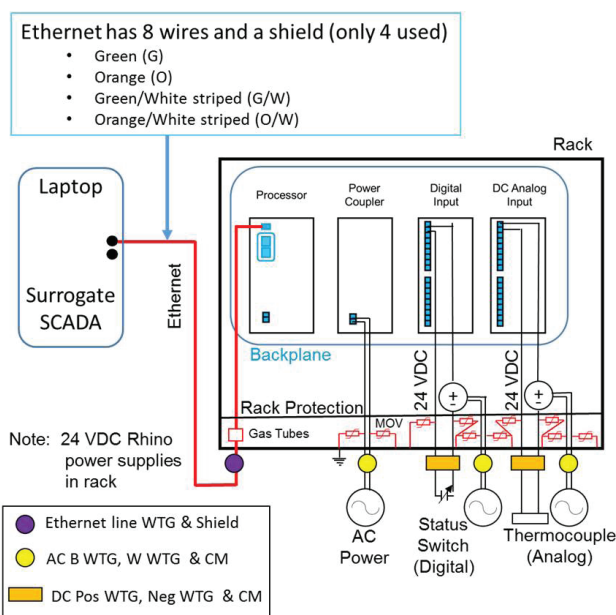
Figure 16. Protected rack Model-PGP-A PCI test point configuration.
