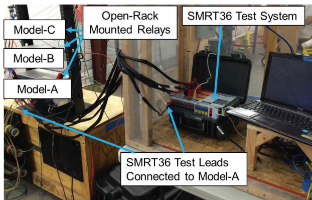
Figure 9. Close-up of the PCI test configuration showing the Megger SMRT36 protective relay test equipment.
