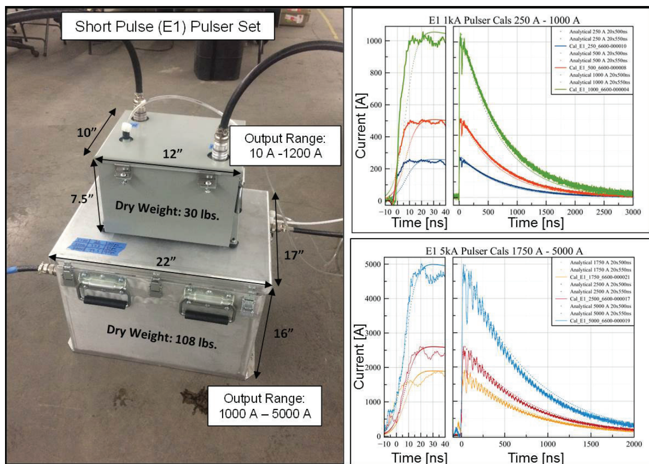
Figure 3. PCI HEMP E1 threat exposure using MIL-STD-188-125-1 App. B waveforms.
