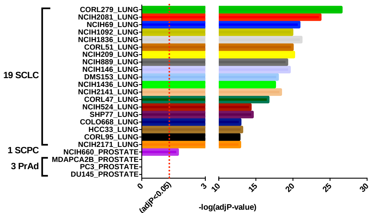
Fig. S8. PARCB cell lines have a strong transcriptional similarity to SCLC as well as SCPC cell lines. Computational analysis tool (DESeq2) identified 1232 up-regulated genes ( >2 log fold change, adjusted P < 0.01 , described in materials and methods, and table S2) in PARCB cell lines compared to patient-derived PrAd lines (LNCaP, 22RV1, and VCaP). Using the gene list, gene list enrichment analysis (Enrichr, http://amp.pharm.mssm.edu/Enrichr ) identified that the top 19 cancer cell lines which were all SCLC cell lines and 1 SCPC (NCI-H660) cell line were significantly shared genes in the list with PARCB cell lines (table S4).
