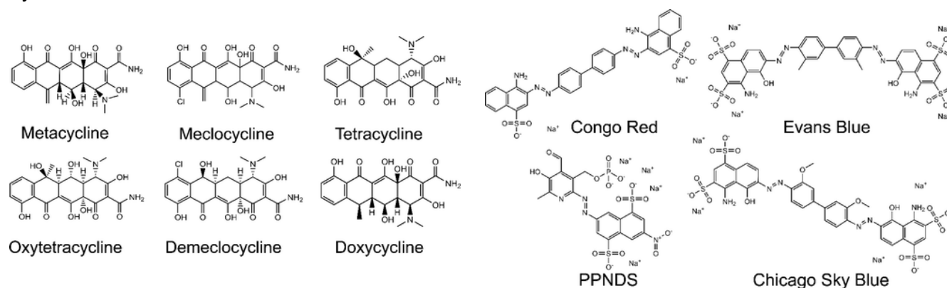
Figure 3. Some of the tetracycline and azo dye derivatives with IC 50 values < 10 \mu M identified in the high-throughput screen.
