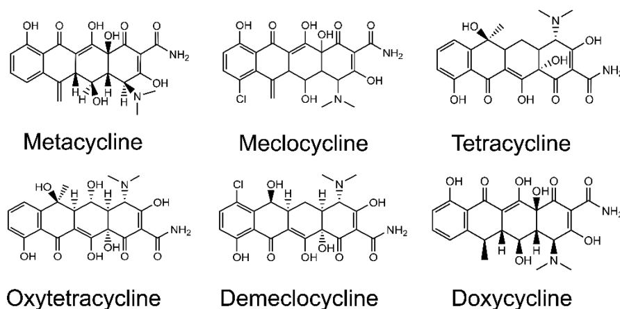
Figure 3. Tetracycline derivatives identified in the screen. Shown are the structures and names of the top tetracycline active compounds (IC 50 < 10 μM) selected in the screening campaign.
