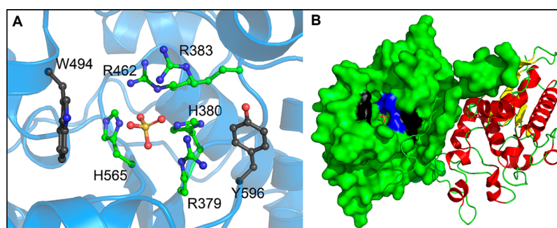
Figure 6. Active site of the histidine phosphatase domain of Sts-1. In addition to the catalytic histidine residues (H379 and H565 shown in ball-and-stick representations with green carbon atoms and blue nitrogen atoms) and conserved arginine residues (R379, R383, and R462 shown in ball-and-stick representations with green carbon atoms and blue nitrogen atoms), two aromatic residues (W494 and Y596 shown in ball-and-stick representations with black carbon atoms, blue nitrogen atoms, and red oxygen atoms) occupy the phosphatase active site of Sts-1 (A). A sulfate molecule (shown with a ball-and-stick representation with the sulfate atom shown in orange and oxygen atoms shown in red) in the structure acts as a phosphate surrogate and marks the site where catalysis occurs. Overall view of the Sts-1 HP dimer (B); the left protomer shows a surface representation where the conserved His and Arg residues are colored blue, while W494 and Y596 are colored black, illustrating how Trp494 and Tyr596 are at the periphery of the active site and could serve a role in positioning planar aromatic inhibitors to block access to the active site.
