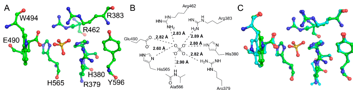
Figure 2. Active site of human Sts-1 HP . A ball-and-stick diagram (A, carbon atoms colored green, nitrogen atoms colored blue, oxygen atoms colored red, and the sulfur atom colored yellow) shows the active site residues of Sts-1 HP around the phosphate binding pocket (marked by the sulfate in this structure). In addition to the conserved histidine residues and arginine residues, additional hydrogen bonding contacts are made to the sulfate by an additional arginine residue and a glutamate residue (B). The superposition of the human and murine Sts-1 HP (C, overall root-mean-square deviation of 0.35 Å) illustrates that the architecture of the active site is highly structurally conserved. The only observed difference is a slight change in the orientation of the tryptophan (W494 in the human protein) at the edge of the active site.
