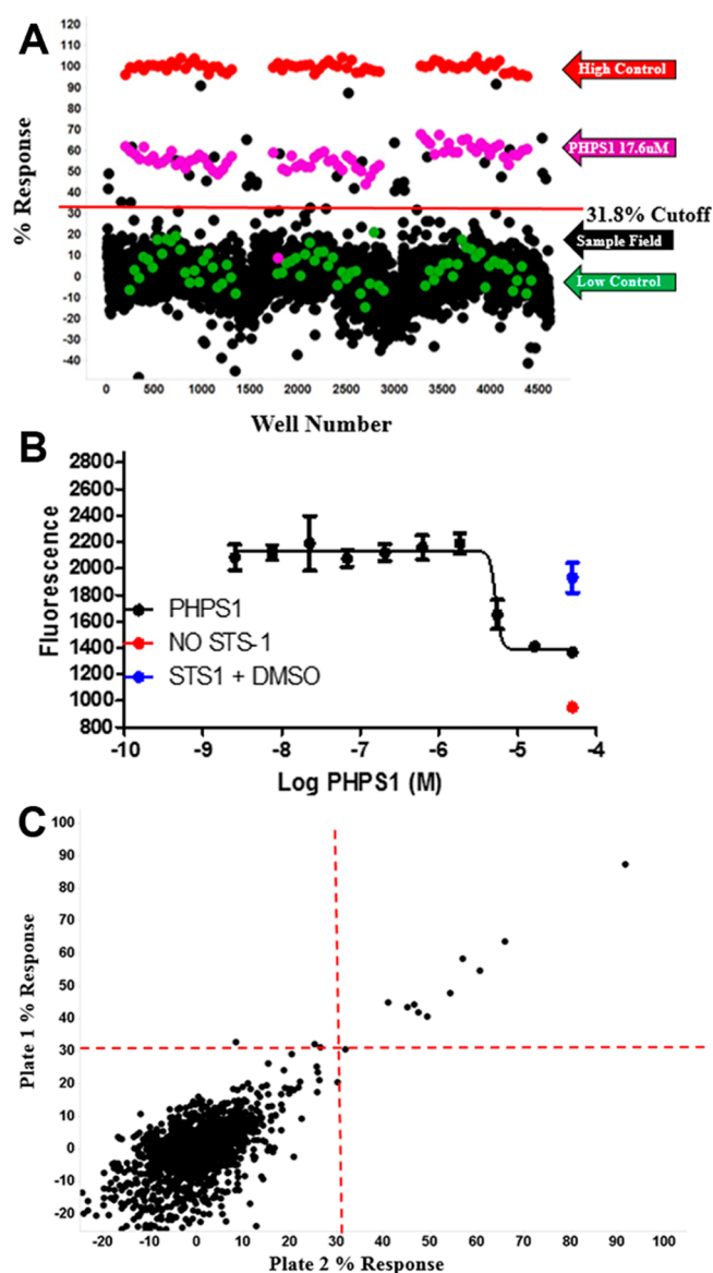
Figure 1. Pilot screen. The % response (A) for the 1280 LOPAC library compounds, conducted in triplicate, is shown. The high control is plotted in red, the low control is plotted in green, the PHPS1 standard is plotted in magenta, and the samples are plotted in black. Compounds that had a response greater than 3 times the standard deviation (a 31.8% response in this case) were selected as active. The potent Sts-1 inhibitor, PHPS1, which has an IC_{50} of 17.6 \mu M (B), was used as a positive control. A correlation plot (C) of the compounds screened in duplicate plates is shown ( R^2 = 0.933 ). The hit cutoffs are designated by red lines.
