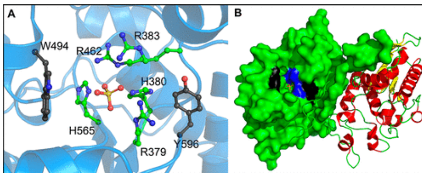
Figure 4. Active site (A) of the histidine phosphatase domain of Sts-1, showing conserved residues and two aromatic residues that likely play a role in how the inhibitors that we identified bind to the active site. The overall dimeric structure (B) is shown and the positions of the conserved residues (blue) and these aromatic residues (black) are highlighted.
