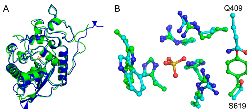
Figure 3. Structure of human Sts-2 HP . The overall fold of human Sts-2 HP is nearly identical to that of Sts-1 HP . A superposition of the Sts-2 HP protomer with the equivalent Sts-1 HP protomer (A, Sts-1 colored green and Sts-2 colored blue, RMSD of 1.02 Å) shows only subtle differences in peripheral loop regions. Similarly, the active sites of the two proteins align well (in panel B, Sts-1 has green carbon atoms and Sts-2 has cyan carbon atoms; in both structures, the nitrogen atoms are colored blue, oxygen atoms are colored red, and the sulfur atom is colored yellow) but do show some subtle yet distinct differences. Whereas the conserved histidine and arginine residues line up well, a tyrosine and a valine in Sts-1 (Y596 and V386, respectively) are replaced with a glutamine and a serine, respectively, in Sts-2 (Q409 and S619, respectively). It is these differences that likely account for the substrate selectivity of the Sts proteins.
