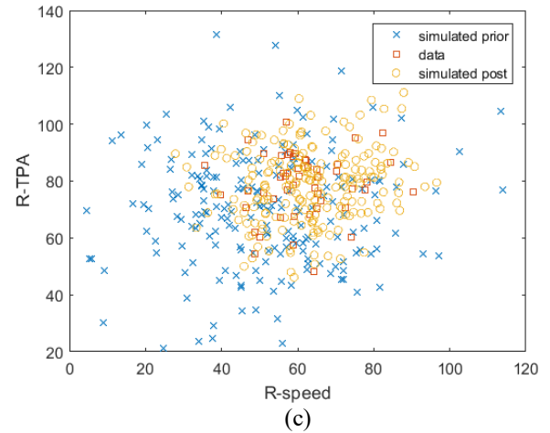
Figure 4. Scatter plots of the prior and posterior distributions and the incoming data for the three random variables.
