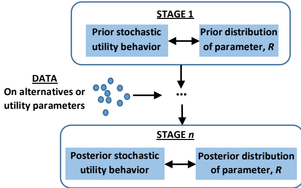
Figure 2. Summary of the proposed approach. Posterior from a stage acts as the prior for the next cycle of updating.
