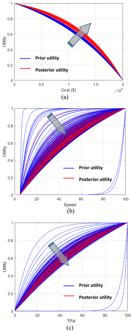
Figure 5. Plots of the prior and posterior utility functions for the three attributes.
