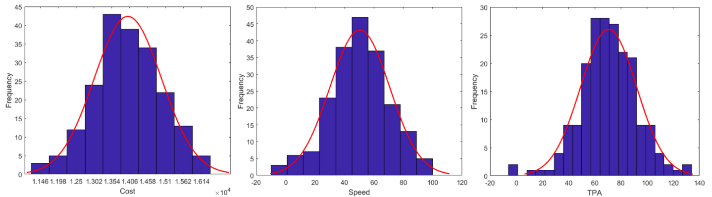
Figure 3. Histograms of risk tolerances associated with the three attributes.
