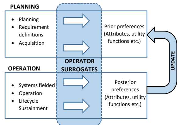
Figure 1. Prior utility function in planning and posterior utility function in operation.
