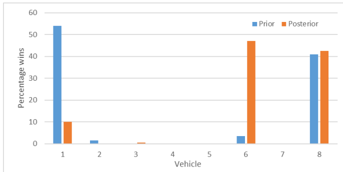
Figure 7. Percentage of decision makers preferring each vehicle.
