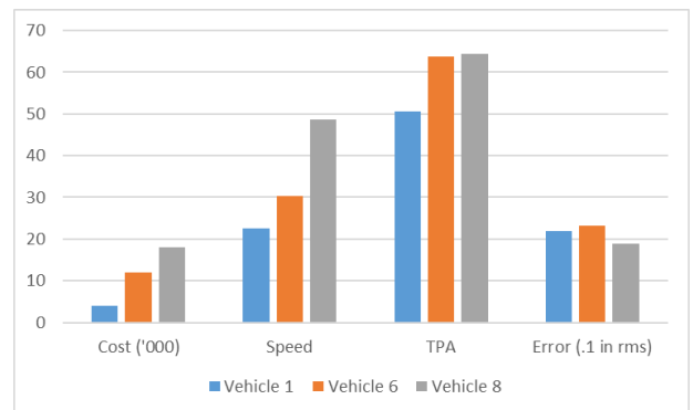
Figure 6. Relative attribute levels achieved by vehicles 1, 6 and 8.
