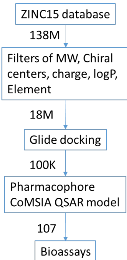
Figure 3. Virtual screening pipeline.
