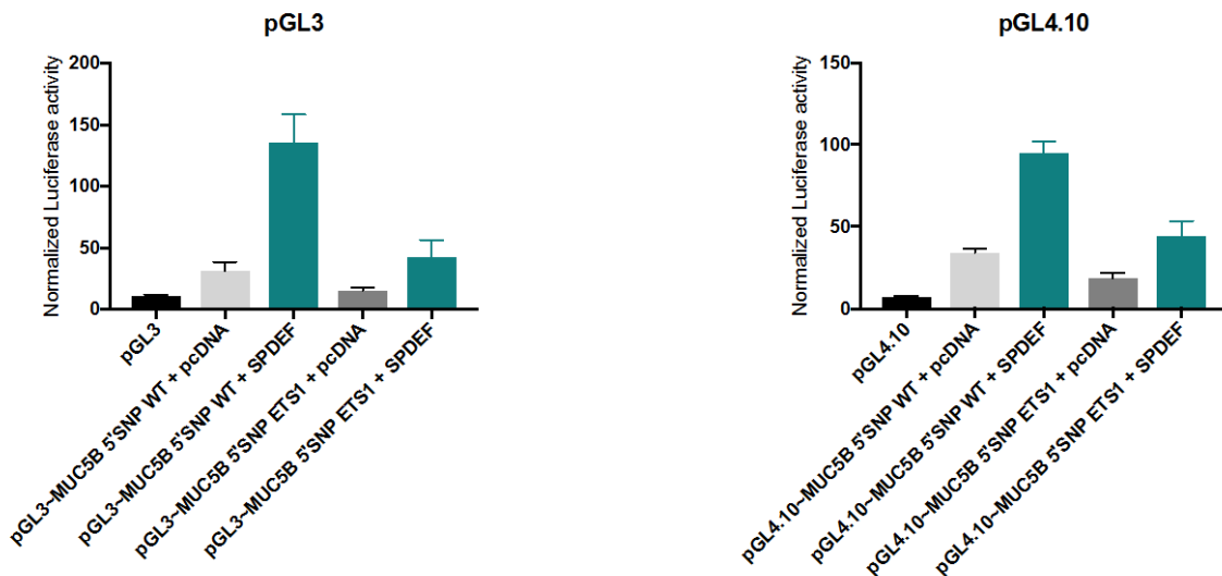
Figure 2. SPDEF regulates the MUC5B -3kB enhancer through a conserved ETS-family binding site.
