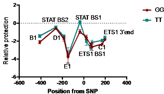
Figure 1: MNase Access assay
