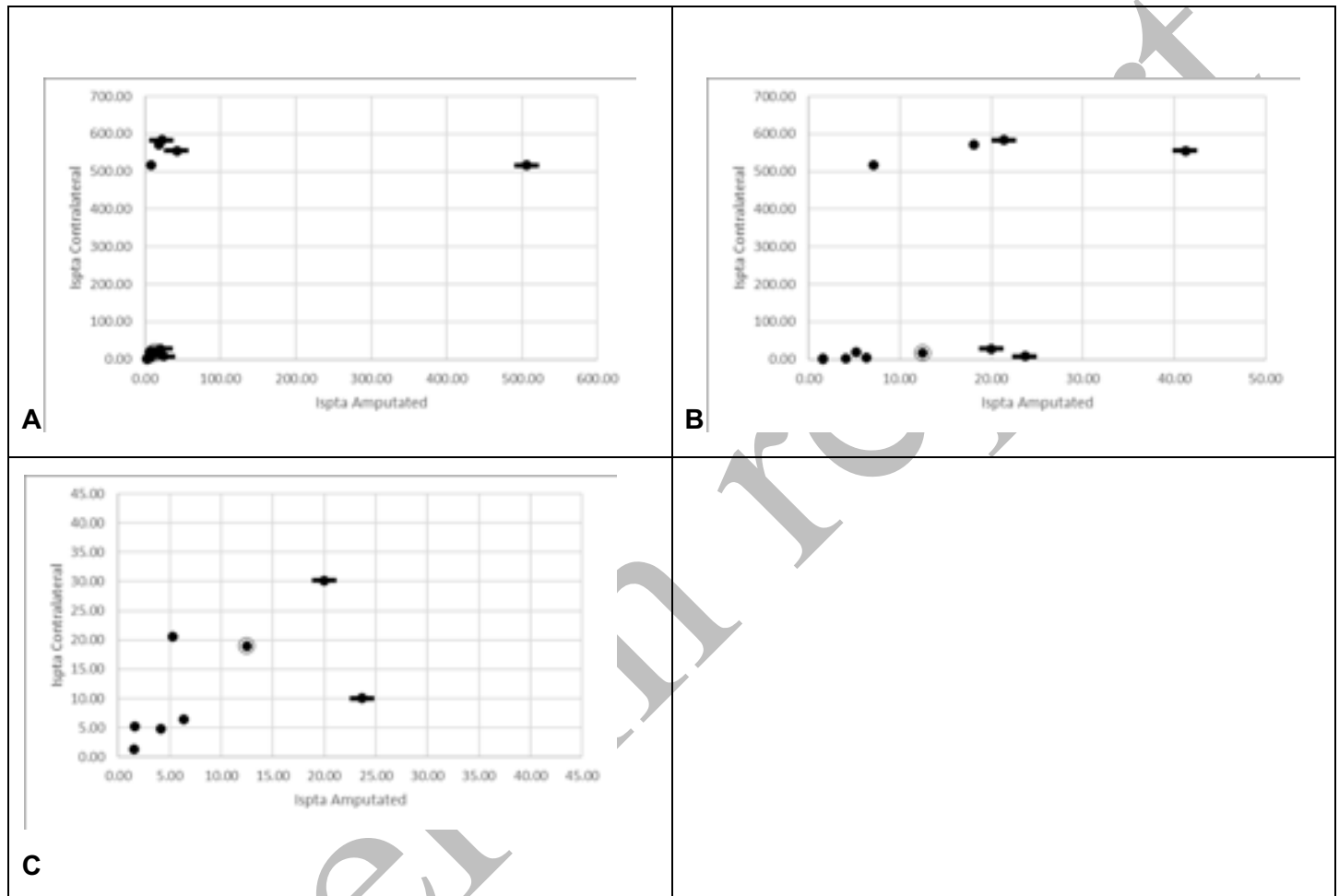
Figure 7. For standard amputee test subjects, paired intensity values necessary to generate a discernable sensation (or maximum of the device) in transected (ipsilateral) and intact (contralateral) nerves, (A) for all test subjects, (B) for all data points save one, and (C) a close up of the data associated with the standard amputees most sensitive to ultrasound stimulation. There was a significant difference in the intensity necessary to create a sensation for the intact versus paired transected nerve across all test subjects (Wilcoxon matched pairs signed-rank test, z=2.587 p<0.01 N=13 ). Removing the outlier, the paired comparison of ipsilateral and contralateral remain did not change these results. There exist a sub-set (C) of standard amputees that have comparable levels of sensitivity to iFU stimulation between their ipsilateral and contralateral limb (Wilcoxon matched pairs signed-rank test, z=1.187 , p>0.25 , N=8 ). Data points with a line through them indicate test subjects deemed neuropathic via the LANNS pain score. Data point with a circle denotes data from a test subject with a neuroma. Note the large difference in range of the ipsilateral versus contralateral data points in Figure 7B.
