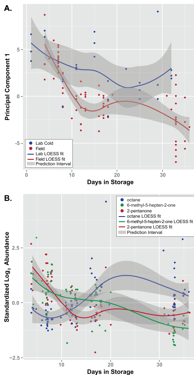
Figure 4. Exhaled breath compound stability in field conditions: (A) A LOESS fit of the first principal component scores (given 54 VOC abundances) and days in storage for the field sampled data (red). The cold laboratory data set was included for comparison. (B) Time courses of relative chemical abundances (normalized, transformed, and standardized) ( p = \pm 0.6, p < 0.01 ). X-axis values were randomly shifted \pm 0.5 d to avoid over plotting. Prediction interval depicts the 95% confidence intervals for LOESS fitted values. These data shows 19% of the variation in the field sampled data can be attributed to the first principal component. Additionally, the results suggest field sampling and transport causes a reduced stability of compounds over time but at a rate consistent with the laboratory controlled sampling.
