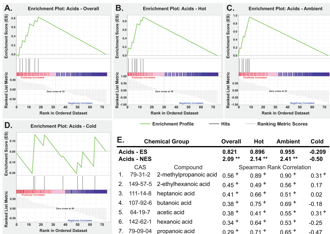
Figure 3. Gene set enrichment analysis for acids: enrichment plots for (A) acid—overall, (B) acid—hot, (C) acid—ambient, (D) acid—cold. Enrichment profile: green line, number of compound hits: black vertical bars, and the ranking metric scores: gray vertical bars. (E) Summary of the enrichment analysis for the acids classification featuring the enrichment score (ES), normalized enrichment score (NES) and the Spearman rank correlation values. The data illustrates the positive enrichment of acids in the overall, hot and ambient data sets. Additionally, Spearman rank correlation values highlight individual compound associations with the enrichment.
