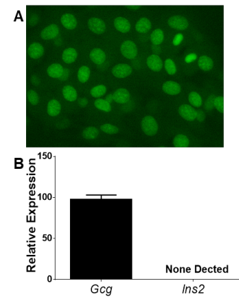
Figure 4. Primary isolated alpha cells in culture (A). Expression of Gcg and Ins2 mRNA (relative to 18S rRNA) in isolated primary alpha cells. Expression normalized to sort negative cells (B). n=3 .
