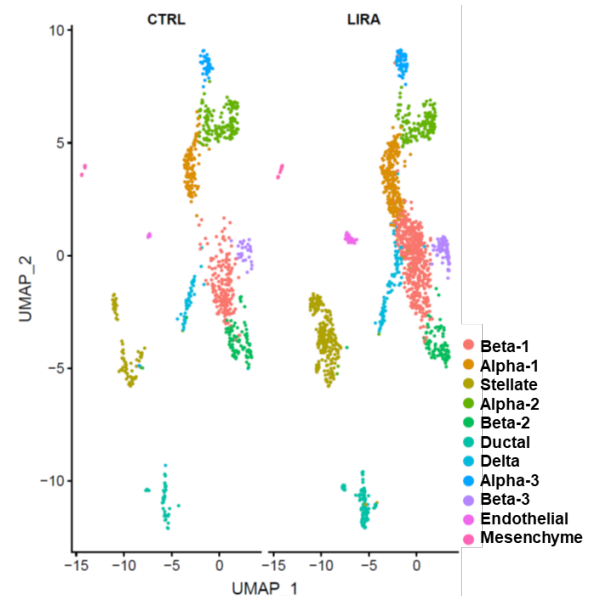
Figure 3. Unsupervised clustering of single cell transcriptomes by UMAP generated from non-diabetic human islets treated with saline (CTRL) or liraglutide (LIRA) (30nM for 12 hours) at 16.1 mM glucose. n = 2 per group.
