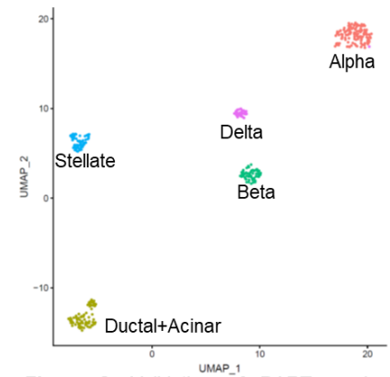
Figure 2. Validation of DART-seq in human islets. Unsupervised clustering of single cell transcriptomes by UMAP. Cell clusters were identified according to expression of known marker genes: insulin (beta), glucagon (alpha), somatostatin (delta), COL1A1 (stellate), KRT19 (ductal and acinar).
