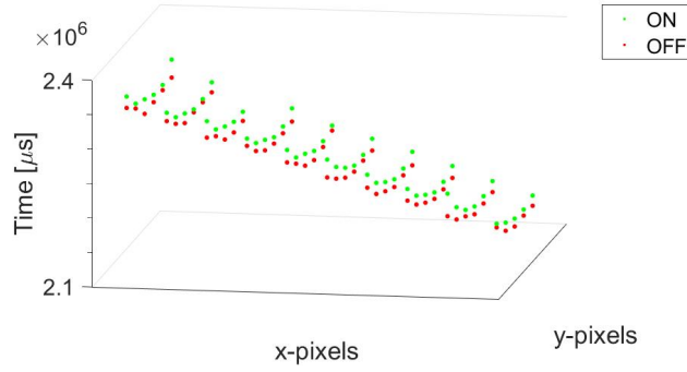
Figure 42: The output of the event pair filters can produce two almost identical layers of events with opposite polarity.
