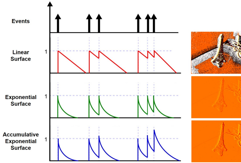
Figure 38: Example of adaptive time surfaces (modified from [71]).
