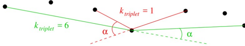
Figure 41: Schematic demonstration of the influence of k_{triplet} on the determination of \alpha [68].
