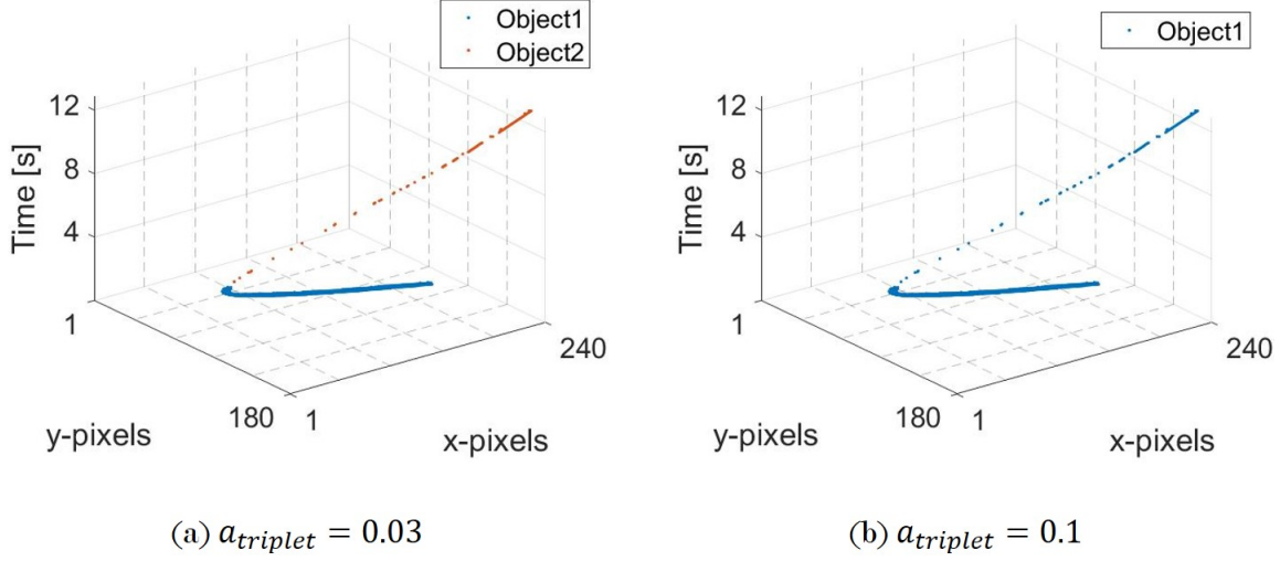
Figure 43: Output of TriplClust acting on banking drone event data. In (a) a_{triplet} is too low to handle the drones change in direction and so creates two separate tracks.
