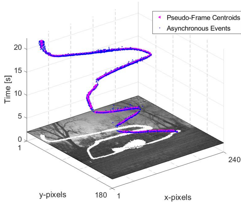
Figure 56: Comparison of tracking the SS40 quadcopter at night.
