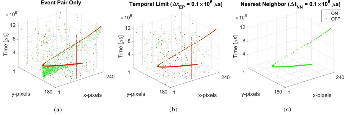
Figure 34: Example application of the event pair filter. For a looping drone, (a) draws out ON/OFF and OFF/ON pairs only while (b) enforces a maximum temporal separation between those event pairs. (c) then applies the nearest neighbor filter to produce a very clean result.
