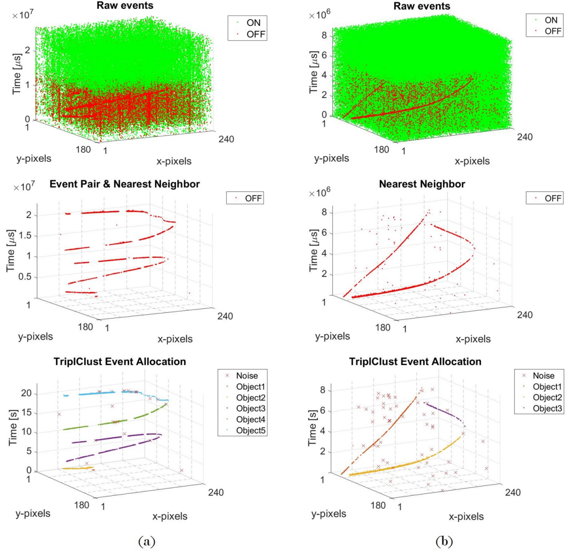
Figure 44: Example output of TriplClust acting on (a) an airborne quadcopter flying at night with a flashing LED and (b) an airborne drone flying during the day with a bird also flying through the FOV.
