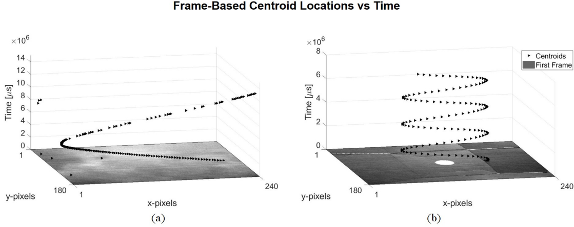
Figure 28: Frame-based centroids displayed as a function of time. (a) An airborne drone banking (b) A swinging pendulum.
