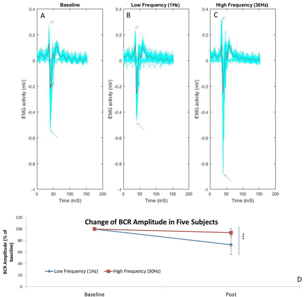
Figure 3: Change in bulbocavernosus reflex (BCR) amplitude, which is measured from the perineal muscle EMG, during low frequency (1 Hz) and high frequency (30 Hz) transcutaneous magnetic spinal cord stimulation. A, B & C. An example of measured the BCR from subject C at Baseline (A), after low frequency stimulation (B) and after high frequency stimulation (C) respectively; blue = individual electrical recordings; red = average. D = amplitude changes in all five subjects. Note a significantly higher degree of reduction of BCR amplitude after low frequency stimulation when compared to high frequency stimulation. Student's t-test: *** = p < 0.0001 .
