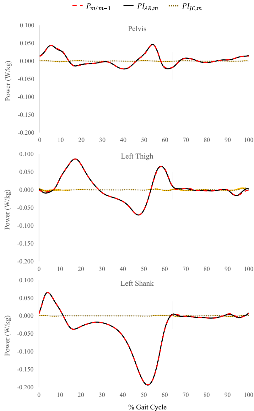
Fig. 3. Average power imbalance between the segmental rate of energy change and the anatomically relevant kinetic method ( P_{I_{AR,m}} ) is almost completely explained by the average power due to the relative segment endpoint displacement ( P_{m/m-1} ), as seen graphed over 100% of the gait cycle (where m represents the pelvis, left thigh, or left shank). Average ( \pm 1 standard deviation in yellow) power imbalance between the segmental rate of energy change and the joint center kinetic method ( P_{I_{JC,m}} ) is relatively small in comparison to P_{I_{AR,m}} . The range of P_{m/m-1} is smaller in swing phase (indicated to the right of the vertical black line at 63%) than in stance for all three segments, and largest in the left shank compared to the thigh and pelvis over stance phase. (For interpretation of the references to color in this figure legend, the reader is referred to the web version of this article.)
