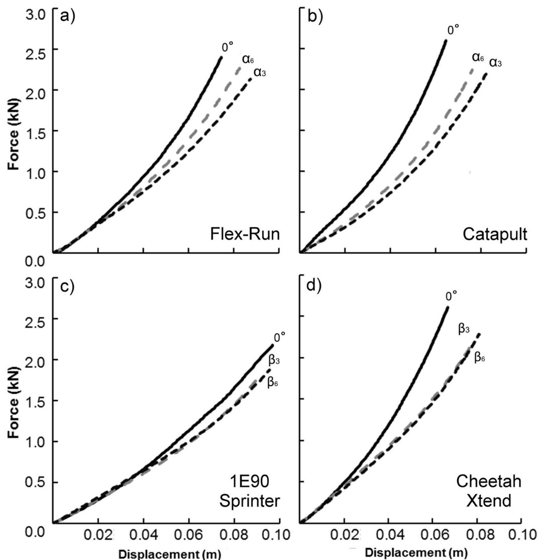
Fig 3. Representative force-displacement profiles for running-specific prosthetic models at each testing angle. Each running-specific prosthesis (RSP) is the manufacturer recommended stiffness category for a 70 kg distance runner. \alpha_3 and \beta_3 indicate the measured angle between the RSP and peak resultant ground reaction force (GRF) vector while running 3 m/s using the C-shaped RSPs (Flex-Run and Catapult) and J-shaped RSPs (1E90 Sprinter and Cheetah Xtend), respectively. \alpha_6 and \beta_6 indicate the measured angles between the RSP and peak resultant GRF vector while running 6 m/s using the C-shaped RSPs and J-shaped RSPs, respectively. a) The Flex-Run prosthesis at testing angles of 0^\circ , \alpha_3 , and \alpha_6 , b) the Catapult prosthesis at testing angles of 0^\circ , \alpha_3 , and \alpha_6 , c) the 1E90 Sprinter prosthesis at testing angles of 0^\circ , \beta_3 , and \beta_6 , and d) the Cheetah Xtend prosthesis at testing angles of 0^\circ , \beta_3 , and \beta_6 .
