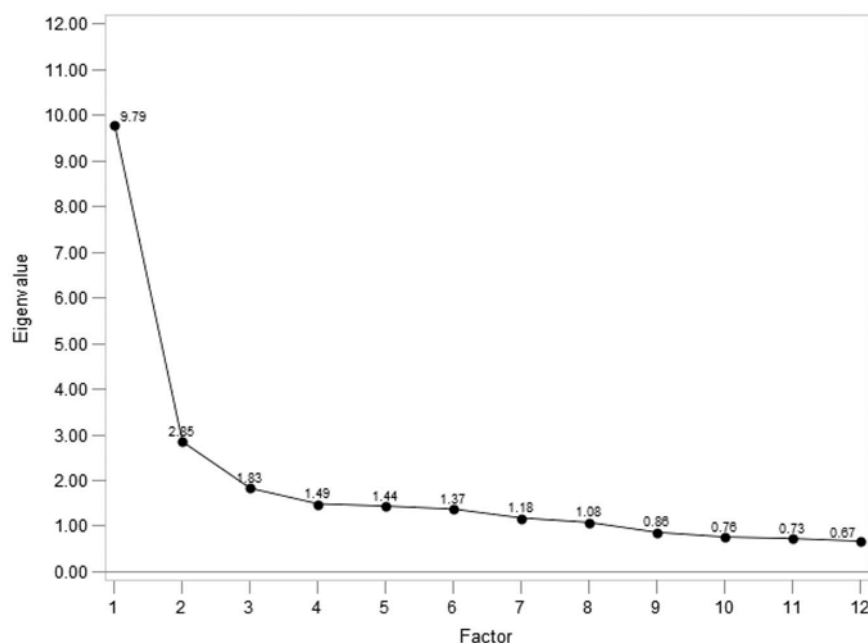
Figure 3. Exploratory factor model scree plot 1 .
