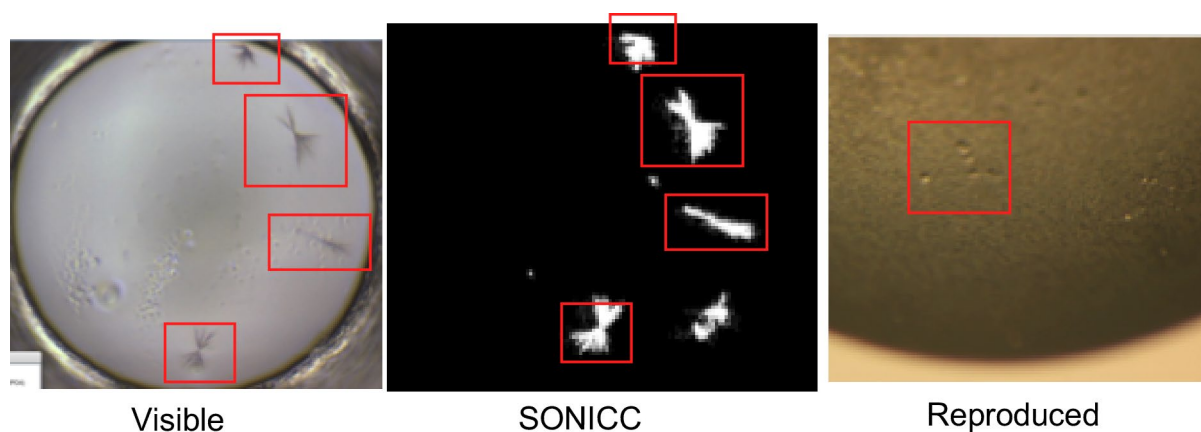
Figure KO3. Crystals of apo ARdbd. Visible and SONICC imaging photos are displayed in the first 2 panels. Crystal correspondences are indicated by red boxes.
