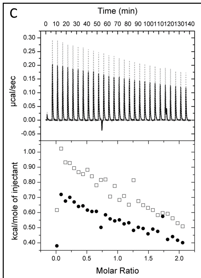
Figure KO1. Isothermal titration calorimetry of AR-DBD against VPC-14449 (dotted lines) is overlaid with the titration of the protein into buffer (heavy lines). ( Top ) The raw ITC data expressed as the change in thermal power with respect to time over the titration period. ( Bottom ) The lower panel shows the integrated heats. The AR-DBD C552A protein (1 mM) was in the syringe and the inhibitor VPC-14449 (100 µM) was in the cell.
