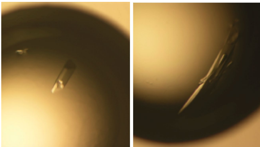
Figure KO2. Crystals of ARdbd + DNA. The crystals were subsequently soaked with 2 mM VP14449 compound. Evidence for the bound ligand was not seen in the electron density maps calculated from diffraction data from these soaked crystals.
