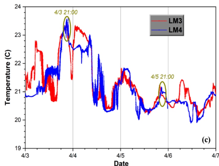
Figure 13. Model-mooring comparison. (a) Model temperature flux ( ^{\circ}\text{C m/s} ) at 21:00 UTC on 4/3; (b) Model temperature flux ( ^{\circ}\text{C m/s} ) at 21:00 UTC on 4/5; (c) Surface temperature ( ^{\circ}\text{C} ) at moorings LM3 and LM4 (times corresponding to model results in panels a and b are indicated).
