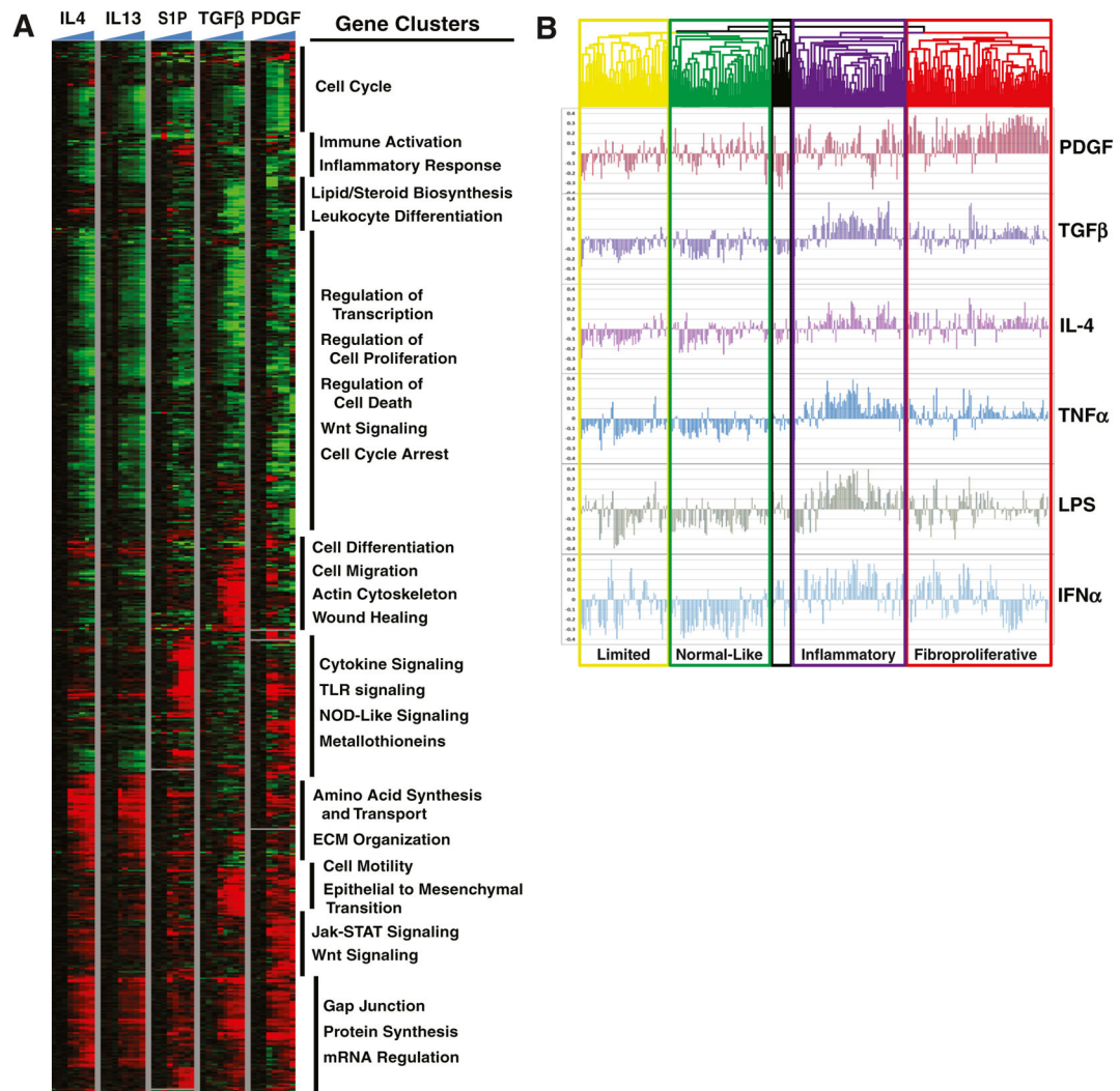
Fig. 1. Pathway activation signatures show differential expression across the intrinsic gene expression subsets. a Normal and SSc dermal fibroblasts were treated with different pro-fibrotic and immune mediators that have been implicated in SSc. A subset of pathways and fibroblast time courses is shown. b Hierarchical clustering was performed on 329 microarray hybridizations from 287 unique biopsies representing 111 patients: 70 dSSc, 10 lSSc, 26 healthy controls, 4 morphea, and 1 eosinophilic fasciitis from three independent data sets [1–3], as published in [24]. The array tree is color coded to indicate intrinsic subset designations (yellow = limited, green = normal-like, purple = inflammatory, red = fibroproliferative, and black = unassigned). Pearson correlation coefficients were calculated between each pathway and a sample and plotted. Adapted from Johnson et al. PLoS One (2015) with permission [24]
