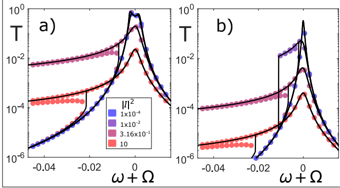
Fig. 4. Transmittance spectra of the system of Fig. 2a when the first resonator experiences a nonlinear detuning ( \chi = 10^{-4} ) and the coupling to the leads is asymmetric. We have used the same parameters as the one used in Fig. 3c. Various incident powers (see inset) are shown. (a) The control parameter is \alpha = \gamma/2\kappa = 0.4 . Notice that the transmittance for incident power |I|^2 = 10^{-2} remains unaffected while the corresponding case in Fig. 3c we observe a drop by \Delta T/T = 60\% . (b) The control parameter is \alpha = 3 . In this case the transmittance T = 34\% is already too low for low incident powers. One needs to compare with the corresponding case in Fig. 3c where T = 1 .
