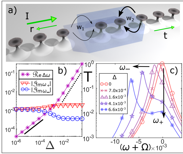
Fig. 2. a) Schematic of a two coupled cavity system (inside transparent box) connected to two transmission lines. The coupling is asymmetric i.e. |w_1| < |w_2| , enforcing differential radiative losses (and therefore Q -factors) between the first and the second resonator. The system is designed to support an EPD. b) Parametric evolution of the frequency difference \Delta\omega \equiv |\omega_{+} - \omega_{-}| and the corresponding imaginary parts of the two eigenmodes versus the linear detuning \Delta . The solid black line has slope 1/2 while the dashed black line has slope 1 and are drawn in order to guide the eye. Notice that \Delta\omega \leq \max\{|\text{Im}(\omega_{\pm})|\} in the domain where the frequency difference scales as \propto \sqrt{\Delta} . c) Transmission spectrum for various detuning strengths \Delta (see labels in the inset).
