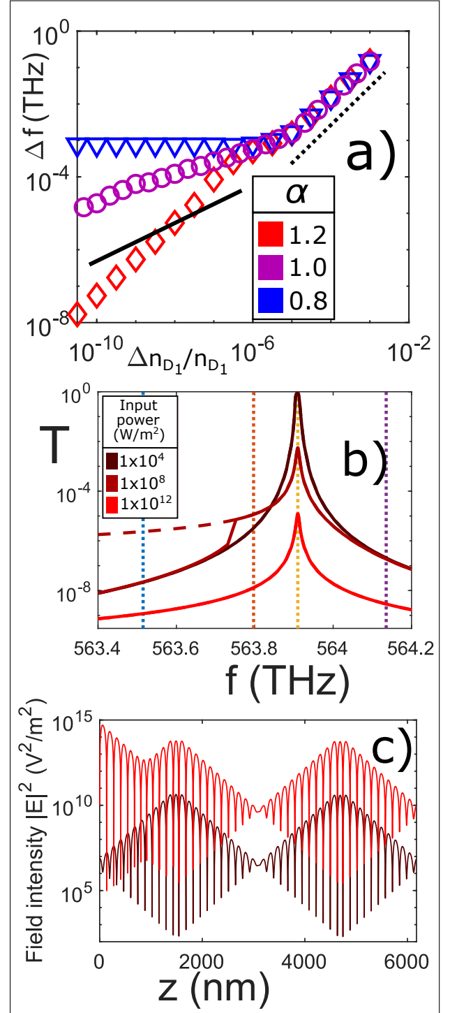
Fig. 5. (a) Resonant split \Delta f as a function of n_{D1} refractive index perturbation when loss is higher (red diamonds), lower (blue triangles) than losses at EPD and when the system is at EPD (purple circles). (b) Transmittance spectra of the free-space multilayer at different incident field intensities. (c) Spatial field intensity distribution within the multilayer at low incident field intensity 10^4 \text{ W/m}^2 (dark red line) and high incident field intensity 10^{12} \text{ W/m}^2 (bright red line).
