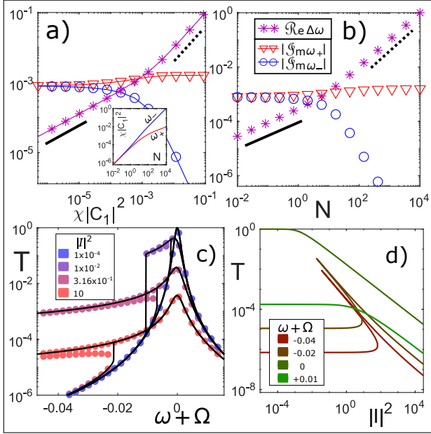
Fig. 3. Parametric evolution of the frequency difference \Delta\omega and of the imaginary parts \text{Im}(\omega_{\pm}) of the two nonlinear stationary modes of a non-linear dimer (see Eq. (9)) with \alpha = 1, \chi = 10^{-4}, \gamma_1 = 0, \gamma_2 = \gamma = 1.6 \times 10^{-3}, \Omega = 0 versus (a) the non-linear detuning \Delta = \chi|C_1|^2 and (b) normalized power N . The solid black line has slope 1/2 while the dashed black line has slope 1 and are drawn in order to guide the eye. Notice that \Delta\omega \leq \max\{|\text{Im}(\omega_{\pm})|\} in the domain where the frequency difference scales as \propto \sqrt{\Delta} . In the inset of (a) we plot the dependence of \chi|C_1|^2 versus N for each of the two modes \omega_{\pm} . (c) Transmission spectrum of the non-linear dimer for four representative values of incident power. (d) Transmission T versus incident power |I|^2 for four representative frequency detunings. Notice that the transmission T associated with the resonant frequency \omega = -\Omega defines the boundary for all other cases. It drops from unit value at small incident powers to (essentially) zero for high incident powers. In (c-d) the parameters of the dimer are the same ones used in Fig. 2c.
