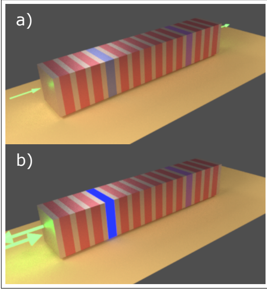
Fig. 1. Multilayer structure involving two optically identical coupled cavities with judiciously chosen differential Q -factors. (a) At low input intensity (in the linear regime), the photonic circuit supports an EPD and displays resonant transmittance. (b) If the input intensity exceeds the LT, the nonlinearity causes an abrupt lift of the EPD, rendering the photonic circuit highly reflective.
