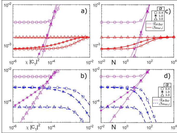
Fig. 7. (a) The \text{Re}(\Delta\omega) , \text{Im}(\omega_+) of the non-linear stationary modes \omega_{\pm} versus the non-linear detuning \Delta = \chi|C_1|^2 for three representative values of \alpha . (b) Same as in (a) but now we report the \text{Im}(\omega_-) ; (c) The same as in (a) but now versus N ; (d) The same as in (b) but now versus N .
