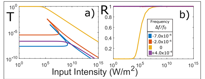
Fig. 6. (a) Transmittance and (b) reflectance of the non-linear multilayer photonic structure as functions of incident intensity at different frequencies in the vicinity of the resonant frequency of the multilayer f_0 . The colors indicate the frequency f of the incident wave and are "correlated" with the vertical lines of the same color from Fig. 5c. The photonic crystal is designed in a way that supports an EPD (i.e. \alpha = 1 ) for low incident powers.
