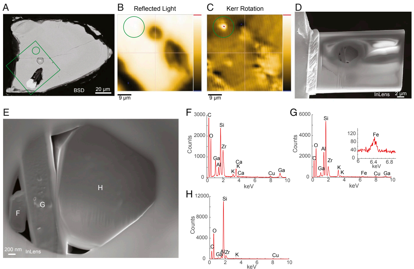
Fig. 5. Primary iron-bearing Jack Hills inclusions. (A) SEM image (backscatter detector [BSD] at 20 keV) of zircon. (B) NanoMOKE reflected-light image of zircon surface. Green circle highlights area of interest (see C). (C) NanoMOKE parallel image showing strong Kerr angle response (red inside green reference circle, note scale on right) from area without any surface features (compare with B). (D and E) SEM images (InLens, 20 keV) of focused ion beam lift-out of area (C) showing strong NanoMOKE response reveal a buried multicomponent silicate inclusion and voids. (F–H) Energy-dispersive analysis reveals the presence of quartz (H) and two different compositions of feldspars (F and G). One of the feldspars (G) bears iron that is a likely source of the magnetic signal. Cu and Ga peaks are related to TEM grid and FIB analyses, respectively.
