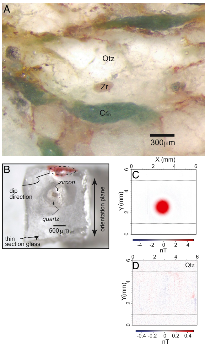
Fig. 1. Jack Hills Discovery Site zircon magnetization. (A) Photomicrograph of 300- \mu\text{m} -thick thin section used to isolate samples for microconglomerate test. \text{Cr}_m , chrome-mica fuchsite; Qtz, quartz; Zr, zircon. (B) Specimen of zircon and surrounding quartz extracted from thin section and used for paleomagnetic measurement with orientation information ( Materials and Methods ). (C) AIST SSM measurement of zircon and quartz after application of a pTRM at 575 ^{\circ}\text{C} in a 61- \mu\text{T} applied field. (D) AIST SSM measurement of quartz only after application of a pTRM at 575 ^{\circ}\text{C} in a 61- \mu\text{T} applied field. Note order-of-magnitude change in scale relative to C.
