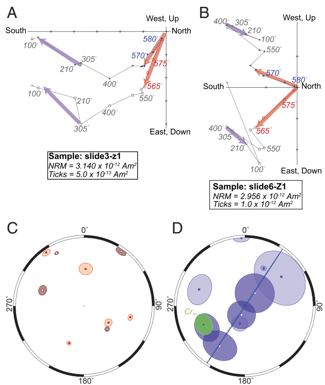
Fig. 2. Jack Hills microconglomerate test. (A and B) Example orthogonal vector plot of thermal demagnetization of microconglomerate specimens. Temperatures labeled are ^{\circ}\text{C} . Horizontal projection of the magnetization (declination) is shown with solid circles; vertical projection (inclination) is shown with open squares. Red arrows, high unblocking (characteristic) remanent magnetization. Purple arrows, low unblocking/intermediate temperature magnetization. (C) Equal area stereonet projection of high unblocking characteristic magnetizations. Uncertainties are maximum angular deviation values of principal component fits. Solid symbols, lower hemisphere (positive inclination); open symbols, upper hemisphere (negative inclination). (D) Equal area stereonet projection of low/intermediate unblocking magnetizations together with direction from the chrome-mica fuchsite (triangle, \text{Cr}_m ) from Cottrell et al. (21). Conventions are as in C. Also shown is great circle fit (solid/dashed line) to low/intermediate unblocking magnetizations.
