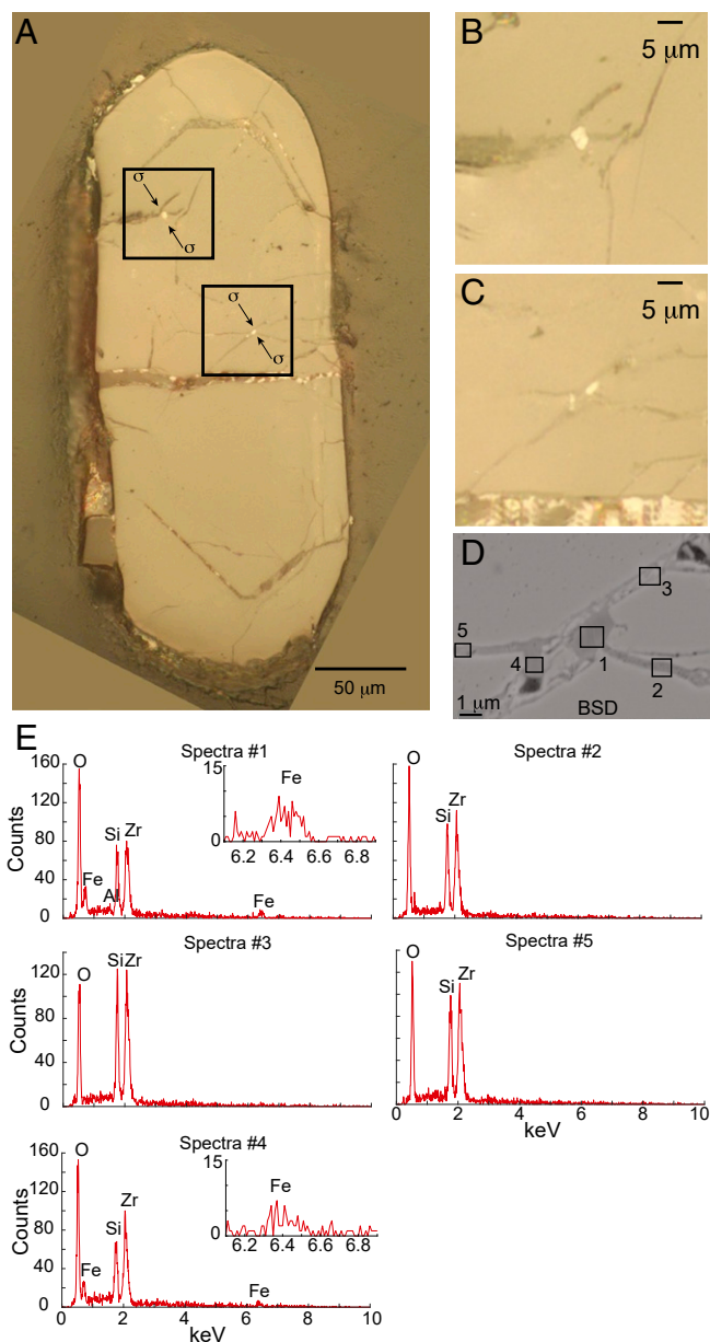
Fig. 3. Optical (reflected light) and SEM analyses of large (1 to 3 μm) magnetite inclusions in JH zircon. (A) Reflected light image (zircon RZ64). (B and C) Partially oxidized magnetite inclusions in crack. Other bright areas (at base) are other reflectors (i.e., not Fe). (D and E) SEM backscatter detector (BSD) image (D) of region C with EDS analysis spots (1–5) and corresponding spectra (E). Also shown is possible stress orientation ( \sigma ) in A, suggesting cracks emanating from inclusion in B and C were formed under the influence of the same stress field.
