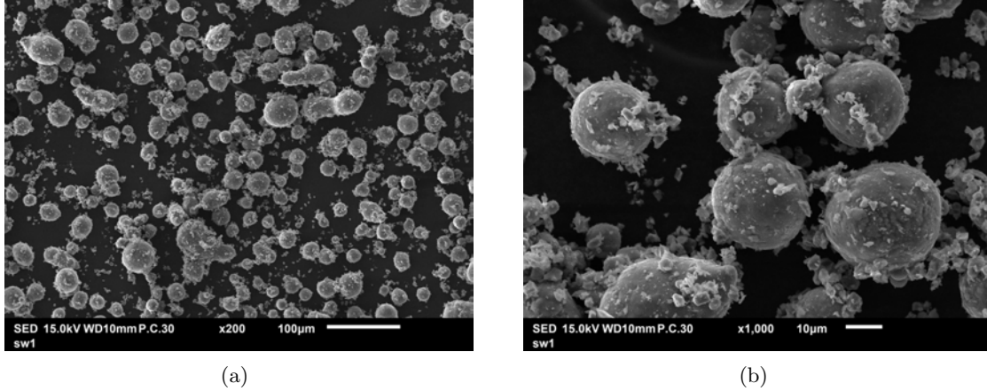
Figure 4. Composite powders fabricated by mechanical blending: Valimet Al-Si10-Mg standard powder mixed with H.C. Starck Grade F powder at 10 wt% ceramic: (a) 200 \times magnification; (b) 1000 \times magnification.
