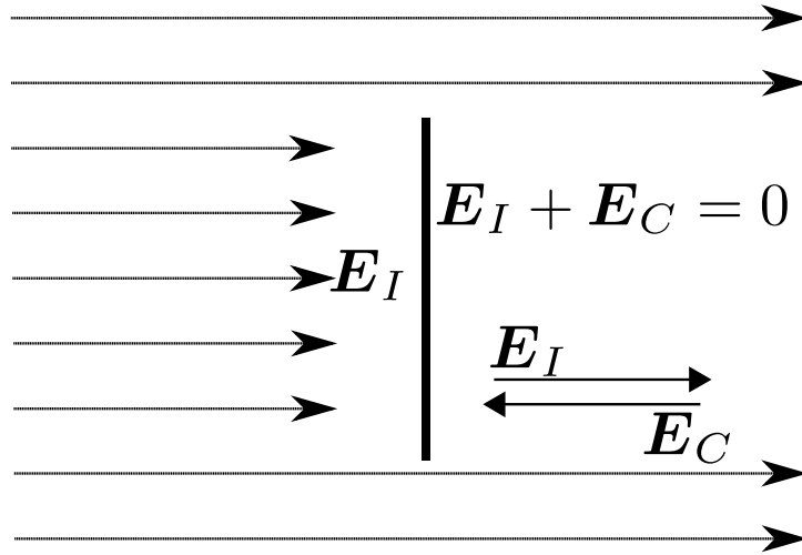
Figure 3. Shadow 'radiation'.
