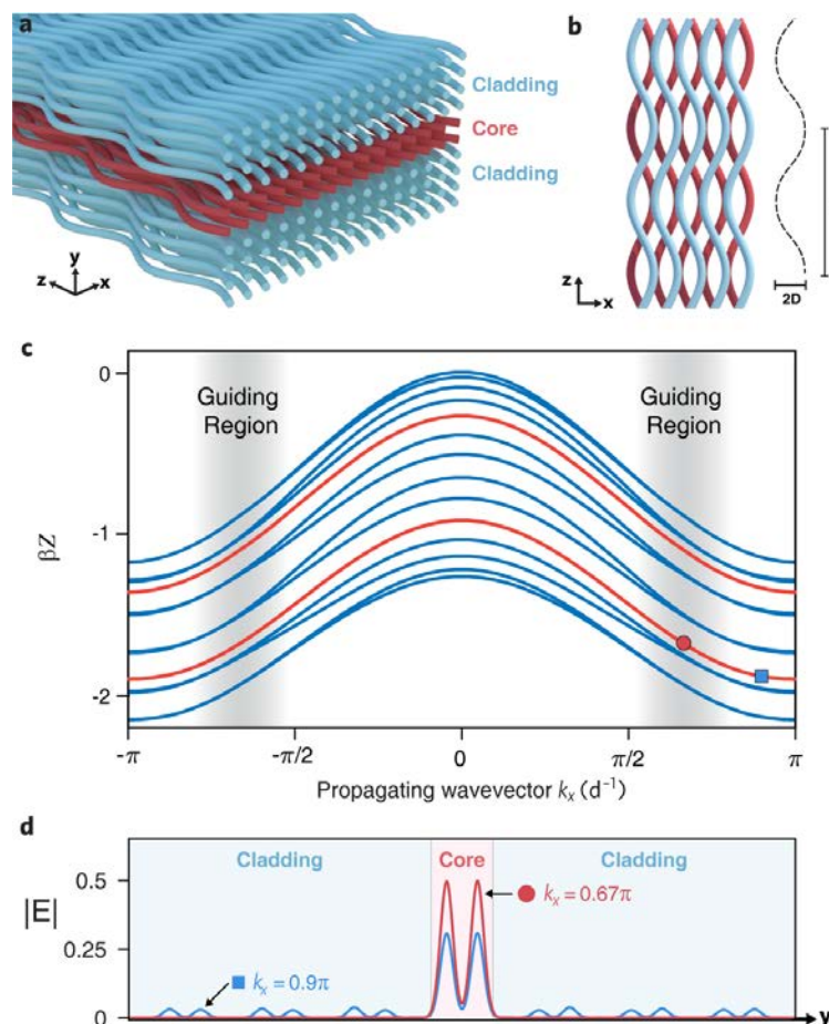
(a),(b) Schematic of the two dimensional waveguide array of sinusoidal trajectories displaying guiding by phase-shifted artificial gauge fields. All the waveguides have the same index profile and follow a sinusoidal trajectory with the same periodicity and amplitude (A), but the cladding (blue) and core (red) rows are shifted by a \pi phase. (c) Dispersion relation of the waveguide array depicted in (a). The z -periodicity of the structure gives rise to periodic dispersion relation (described by a Floquet spectrum). The blue lines represent the modes that are extended over the whole array, while the red lines
