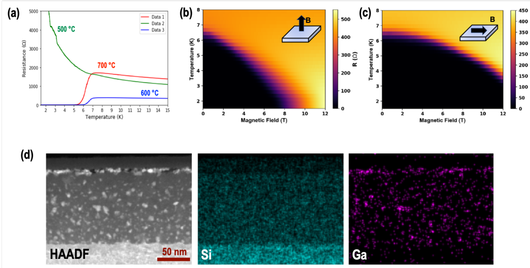
Figure 2: Data on the ion implanted Si superconductivity
