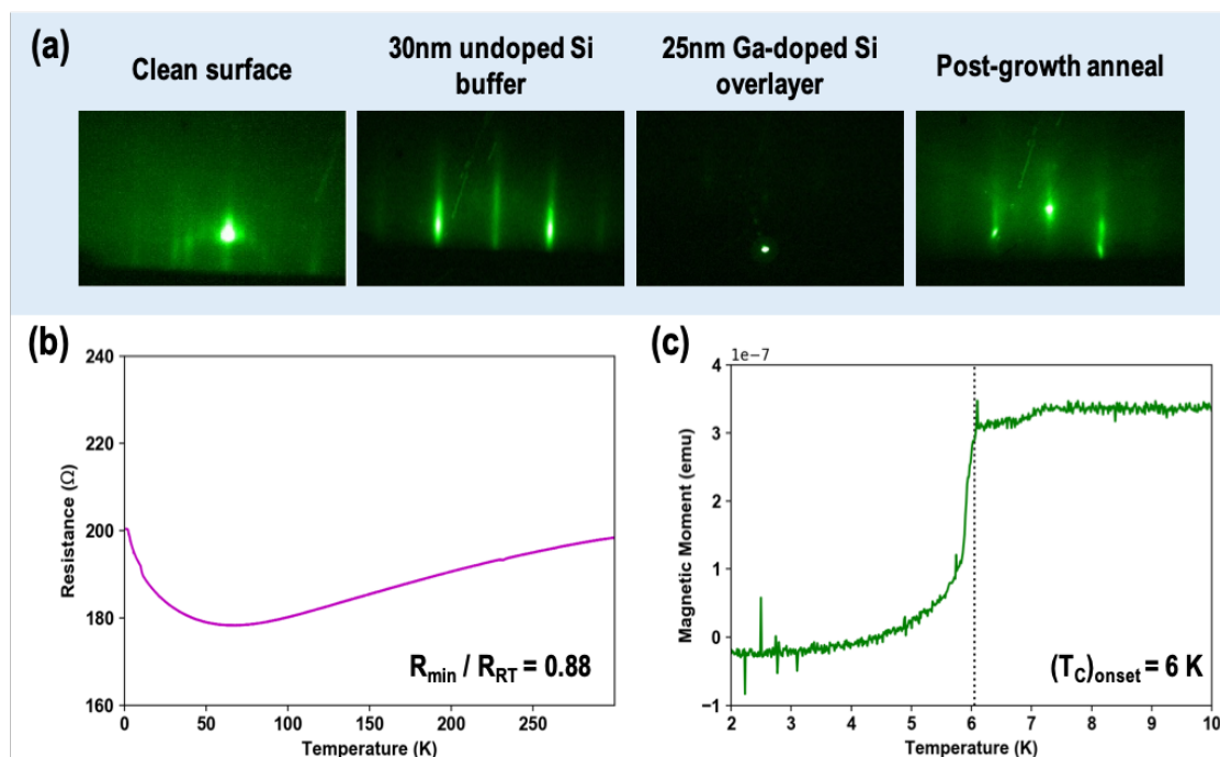
Figure 4: Silicon homoepitaxy results
