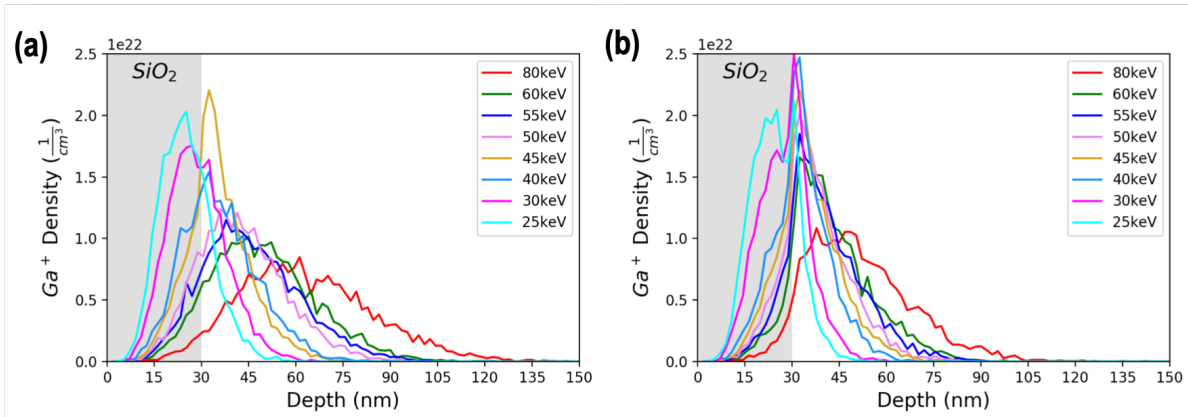
Figure 1: MC simulations of Ga implantation in Si and Ge
