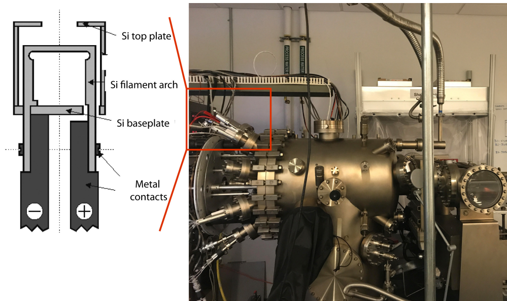
Figure 3: A photo of our molecular beam epitaxy machine and the schematic of our silicon source. The filament is made of Si that slowly evaporates. In this design it is possible to explore isotropically pure Silicon deposition as well.
