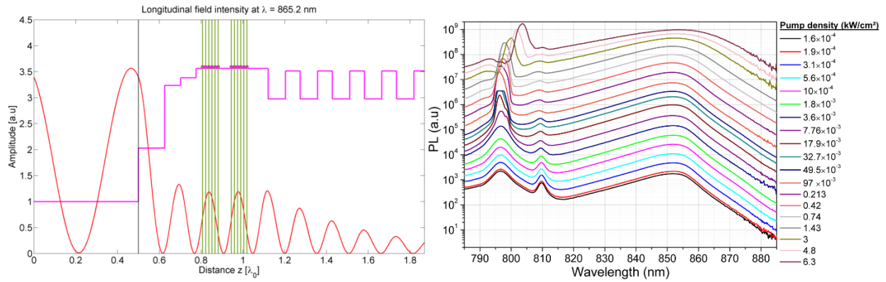
Figure 3. Structure layout of a MQW structure at 865nm and corresponding PL spectra at different excitation.
