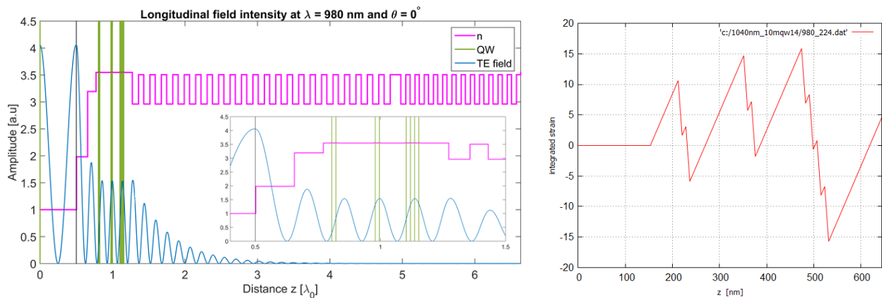
Figure 5. Structure layout of a 980nm MQW (2+2+4 QWs) VECSEL structure with a double DBR 23 (AlGa)As/GaAs pairs for signal + 13 pairs for pump (left) and its integrated strain profile (right).
