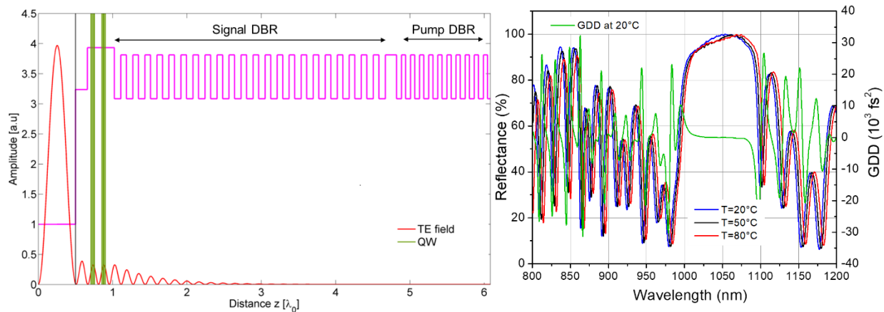
Figure 3. Structure layout of a 4+4QWs VECSEL at 1040nm with a double Signal+Pump DBR (left), and corresponding reflectivity and GDD spectrum (right).
