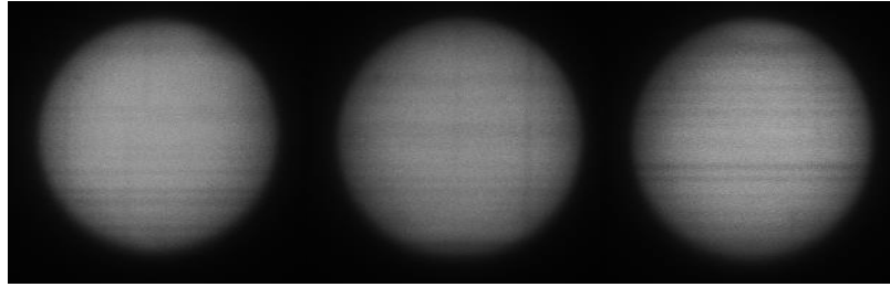
Figure 6. Surface photoluminescence images of a (2+2+4 QWs) VECSEL structure at 980nm.
