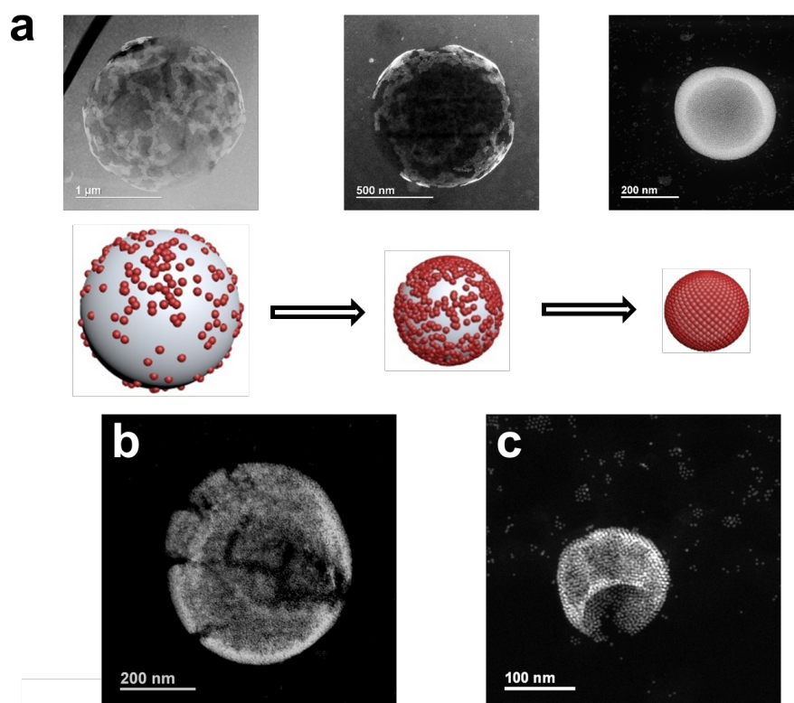
Figure 4 (a) Mechanism of forming intact NP shells at CLLIs from fractal-like patches. Top left and middle insets: cryo-STEM images of OLA-Au NPs absorbed at CLLIs; top right inset: HAADF-STEM image of Au NP HCS. HAADF-STEM images of Au NP HCS (b) annealed at 80 °C and (c) annealed at 58 °C, respectively.
