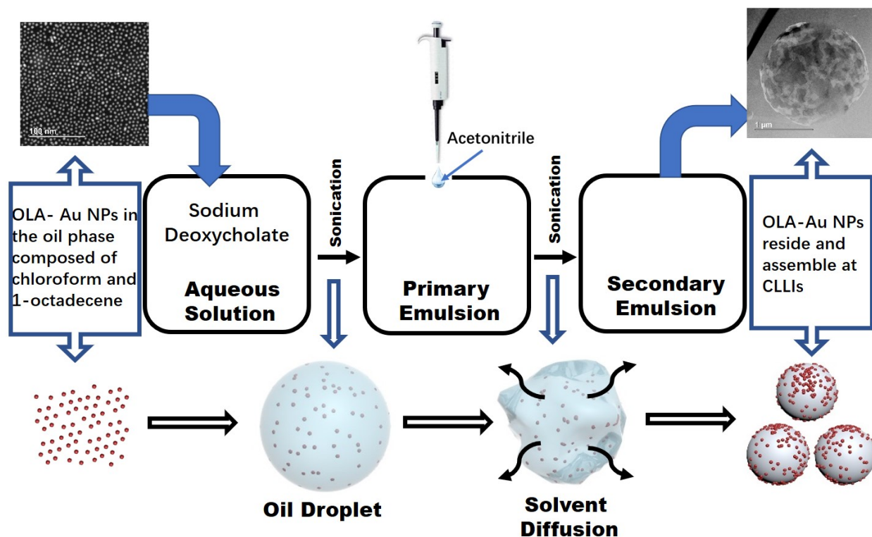
Figure 3 Entropic strategy to stably concentrate NPs assemblies at CLLIs using spontaneous emulsification induced by solvent diffusion. Top left inset: HAADF-STEM image of monodispersed OLA-Au NPs; top right inset: cryo-STEM image of OLA-Au NPs absorbed at CLLIs.
