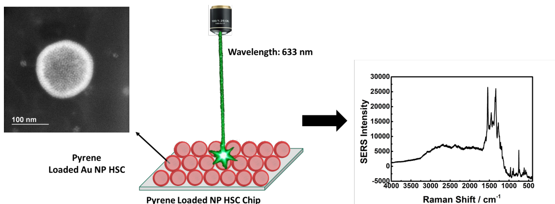
Figure 5 SERS spectrum of pyrene-loaded HCSs.
