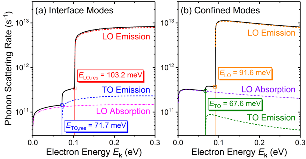
Fig. 5. (a) Interface and (b) confined mode phonon scattering rates are calculated and plotted as a function of electron energy. For both modes, the total interface phonon scattering rate combining all phonon modes (including the TO absorption scattering rate) is shown as the black solid line. The droplines with symbols are shown to indicate the threshold energies of TO emission and LO emission scattering. For interface mode scattering, these energies correspond to the TO and LO interface phonon resonant frequency energies \hbar\omega_{TO,res} = 71.7 meV and \hbar\omega_{LO,res} = 103.2 meV, respectively. For confined mode scattering, the threshold energies are at the vicinity (but not a complete match) of the TO and LO phonon energies of GaN, \hbar\omega_{1z} = 65.8 meV and \hbar\omega_{1Lt} = 91.9 meV, respectively.
