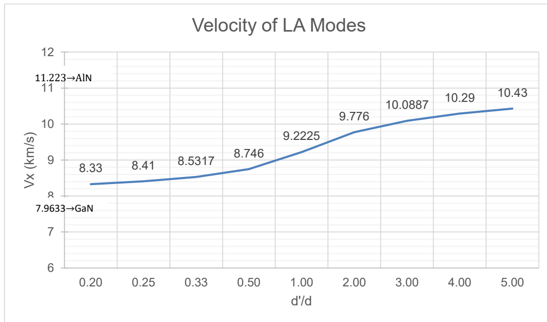
Fig. 3. Sound speed in an AlN-GaN superlattice as a function of the ratio, d'/d when piezoelectric stiffening is taken into account.
