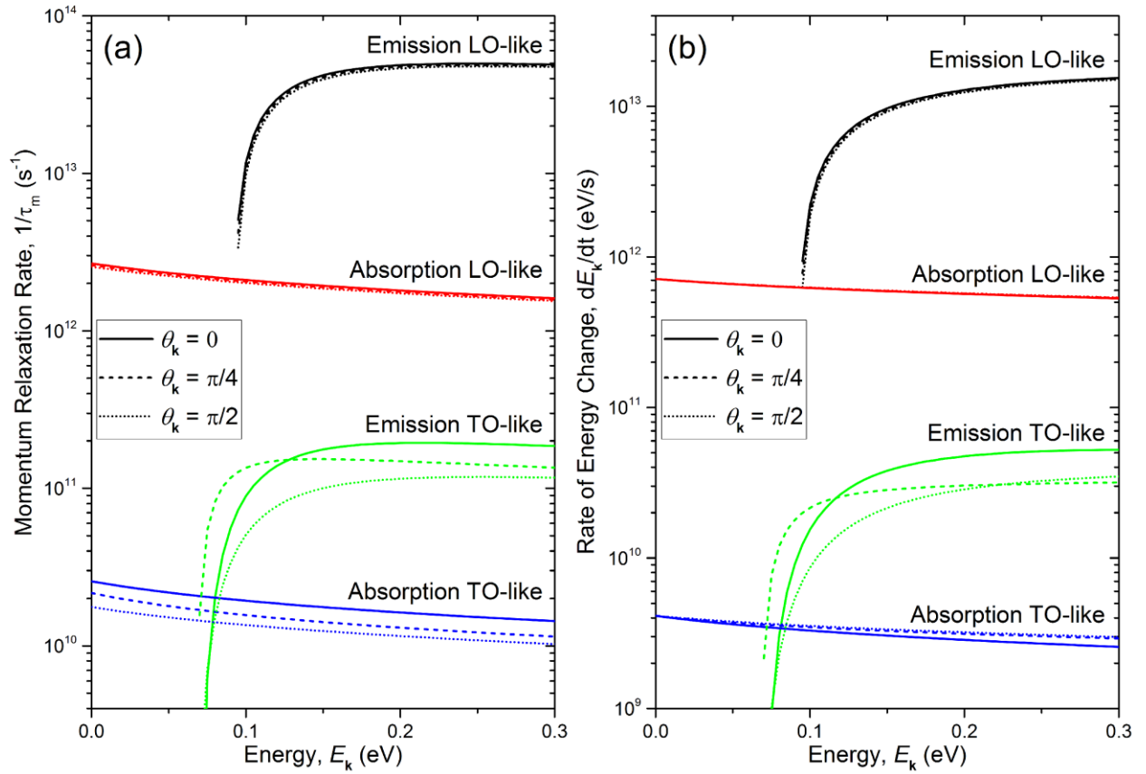
Fig. 1. (a) Absolute value of the momentum relaxation rates and (b) the rate of energy change due to emission and absorption of LO-like and TO-like phonons are plotted as a function of electron initial energy. The temperature is set to T = 300 K and the incident electron angles with respect to the c-axis are set to \theta_k = 0 (solid line), \pi/4 (dashed line), and \pi/2 (dotted line).
