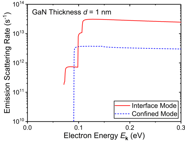
Fig. 6. Interface and confined mode phonon emission scattering rates of a AlN/GaN/AlN double heterostructure with GaN thickness of d = 1 nm is plotted. Compared to the d = 5 nm case, the interface mode scattering rate (red solid line) show a factor of 3 increase, whereas the confined mode scattering rate (blue dashed line) show a factor of 2.5 decrease. Overall, the interface phonon scattering rate is approximately 8 times larger than the confined mode scattering rate with GaN thickness of d = 1 nm.
