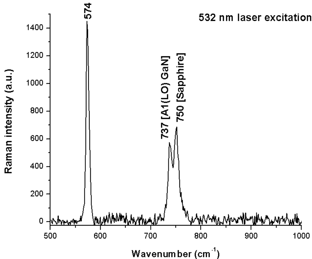
Figure 7. Raman spectra of AlN/GaN control wafer (Parameters: 20s exposure time, 1% Laser power.)
