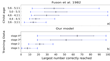
Figure 7: Our model compared with children’s counting data a) Data from Fuson et al. (1982). The x-axis shows the highest number correctly reached when children were asked to count starting at “one.” Boxes correspond to the standard deviation, central bands to the means, and whiskers to the range. b) Model performance, averaged over ten runs at four stages of increasing data quantity.
