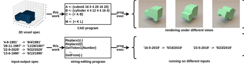
Figure 3: Examples of programs synthesized by our system. Top, graphics program from voxel specification. Bottom, string editing program from input-output specification.
