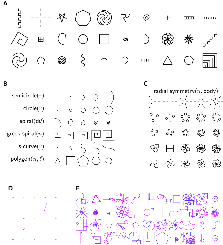
Figure 2: (A) : 30 (out of 160) LOGO graphics tasks. Agent writes a program controlling a ‘pen’ that draws the target picture. (B-C) : Example learned library routines. Agent learns interpretable parametric routines for drawing families of curves (B) as well as primitives that take entire programs as input (C) . Each row of images on the left is the same code executed with different parameters. Each image on the right is the same code executed with different parameters and with a different subprogram provided as input. (D-E) : dreams, or sampled programs, from library before (D) and after learning (E) , (most interesting dreams selected from 5 different runs), showing how dreams become more complex with acquired expertise. Blue: where the agent started drawing. Pink: where the agent ended drawing.
