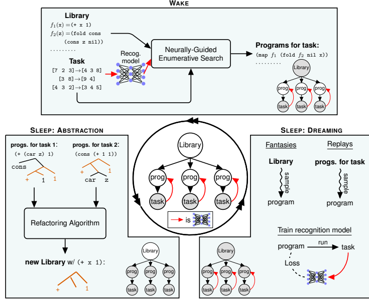
Figure 1: The Bayesian model underlying our model and its basic algorithmic cycle. Middle: DreamCoder as a graphical model. Agent observes programming tasks (e.g., input/outputs for list processing or images for graphics programs), which it explains with latent programs, while jointly inferring a latent library capturing cross-program regularities. A neural network, called the recognition model (red arrows) is trained to quickly infer programs with high posterior probability. Top: Wake phase infers programs while holding the library and recognition model fixed. Left: Sleep (Abstraction) phase updates library while holding the programs fixed by refactoring programs found during waking and abstracting out common components (highlighted in orange). Right: Sleep (Dreaming) phase trains recognition model to predict approximate posterior over programs conditioned on task. Trained on ‘Fantasies’ (programs sampled from library) & ‘Replays’ (programs found during waking).
