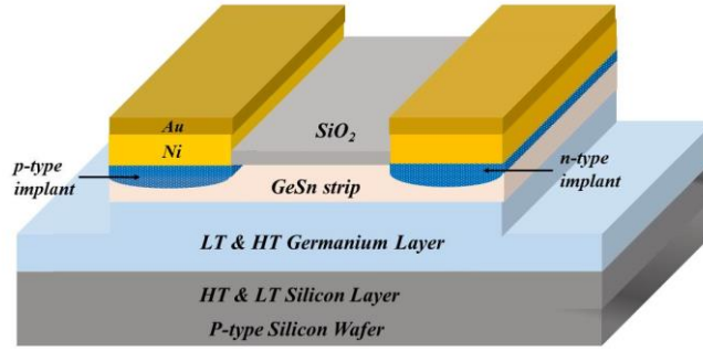
Figure 3. Schematic of the GeSn-based mesa diode that couples into an in-plane waveguide.
