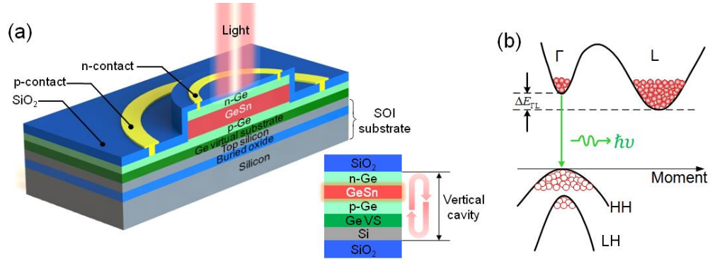
Figure 5. (a) Schematic of our GeSn p-i-n hetero-diode vertical-cavity surface emitter grown on silicon-on-insulator substrates. The buried oxide serves as the bottom reflector and the deposited SiO 2 layer serves as the top reflector, creating a vertical cavity for enhancing the light emitting efficient of the GeSn active layer. (b) Schematic band diagram of the Ge 0.969 Sn 0.031 active layer.
