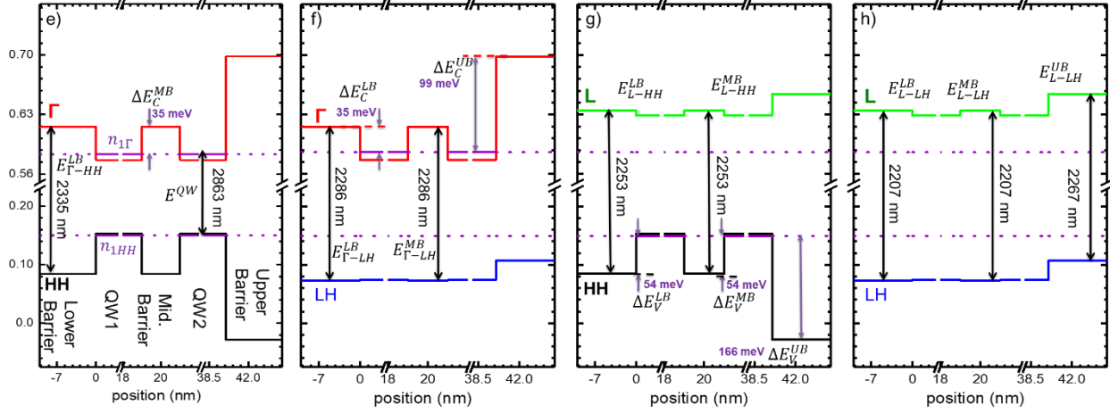
Figure 2. Top: for sample A. Band diagram calculated based on measured material data, showing the carrier confinement and the possible band-to-band optical transitions between (a) \Gamma -HH; (b) \Gamma -LH; (c) L-HH; and (d) L-LH. (Unit: meV). Bottom: for sample B. (e)-(h) The similar band diagram and optical transition calculations.
