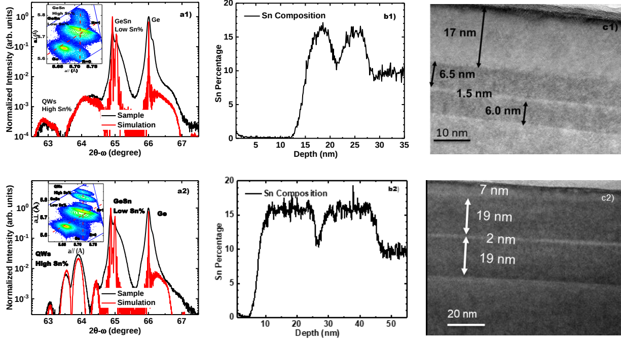
Figure 1. (a1) (a2) HRXRD 2\theta - \omega scan of samples A and B. The black and red curves are measured data and simulation results, respectively. Inset: The RSM contour plot; (b1) (b2) SIMS of samples A and B showing the Sn composition in each layer; (c1) (c2) TEM images of samples A and B.
