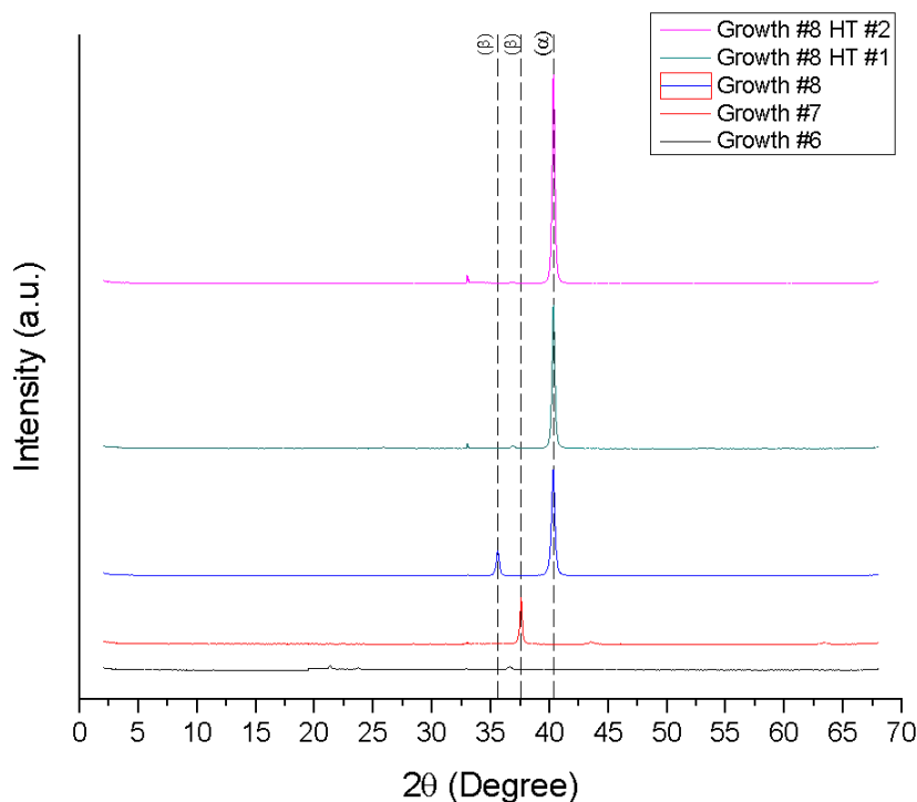
Figure 14. XRD results for three tungsten growth and post thermal annealing.
