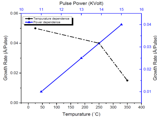
Figure 4. Growth rate dependence to applied power of PED and substrate temperature.
