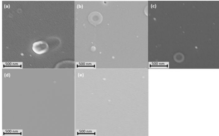
Figure 5. Top SEM view of GeTe thin films deposited by PED in various background pressure: (a) 7.5mTorr, (b) 6.8mTorr, (c) 5.5mTorr, (d) 5.5mTorr and (e) 4.5mTorr; and two target and substrate distances: (a-c) at shorter distance, and (d-e) at longer distance.
