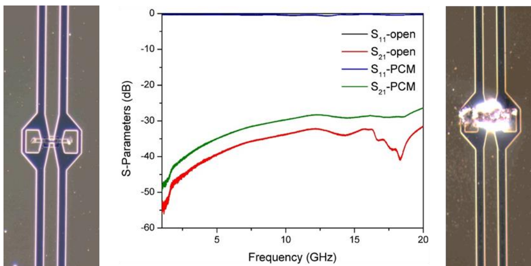
Figure 21. Measured Design 1 PCM sample compared to the open reference in the middle. Design 3 sample before and after direct biasing on the left and on the right, respectively.
