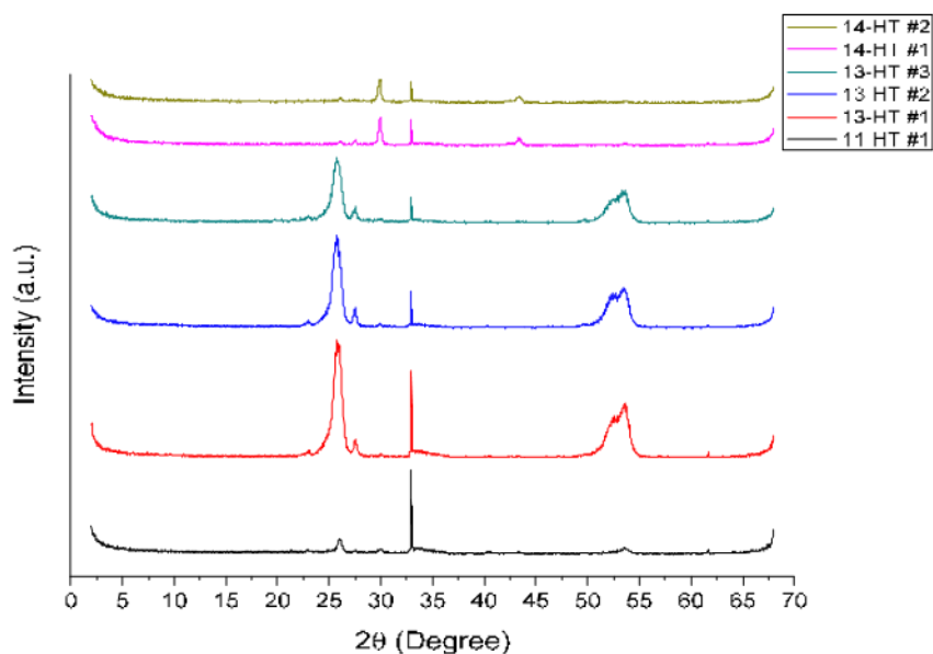
Figure 11. XRD results from different crystallization.
