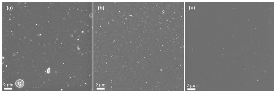
Figure 6. Top SEM view of GeTe thin films deposited at (a) 3 cm (b) 5 cm and (c) 8 cm target-to-substrate distances at pressure of 5.5 mTorr and PEBS of 15 kV.
