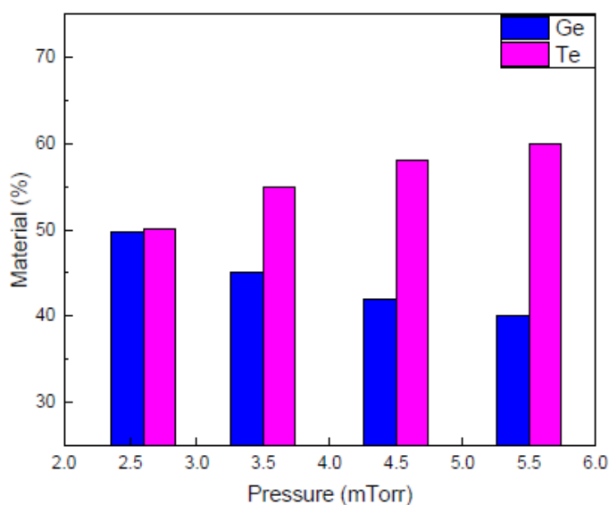
Figure 8. Germanium and Telluride ratio dependence on pressure.
