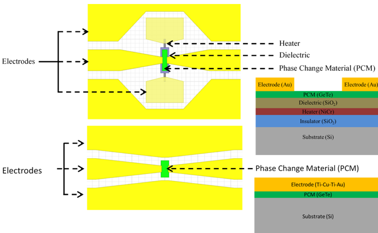
Figure 15. Layout of PCM-based RF switch. (a) Top-view of Design 1, (b) materials stack-up for Design 1, (c) top-view of Design 3, (d) material stack-up for Design 3.
