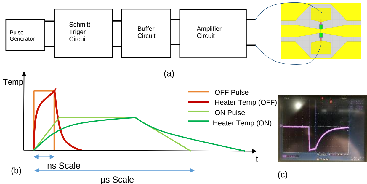
Figure 24. (a) The actuating circuit block diagram, (b) the set temperature profiles along with the actual profiles, and (c) the produced ON pulse.
