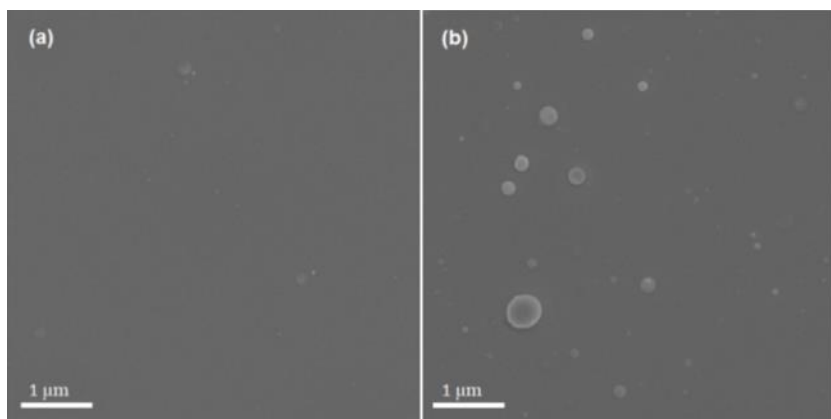
Figure 7. Top SEM view of GeTe thin films deposited at (a) 15 kV and (b) 17 kV PEBS potentials at pressure of 5 mTorr and target-to-substrate distance of 8 cm.
