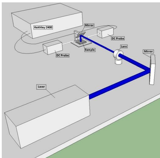
Figure 28. 3D schematic of the laser heating system.
