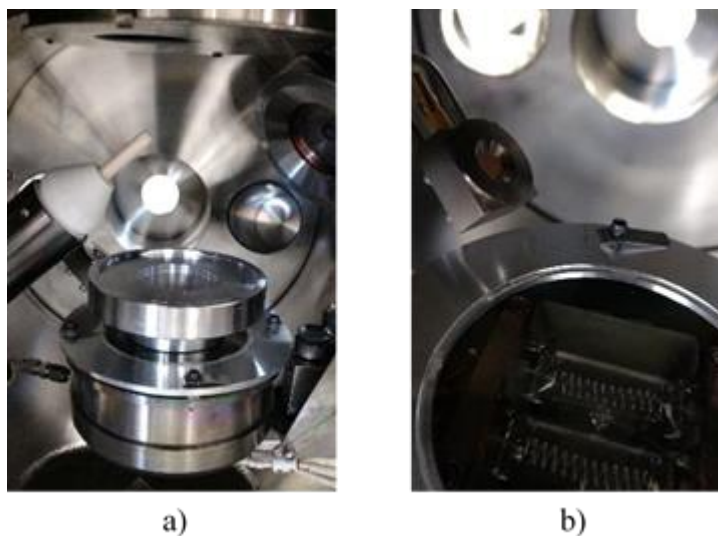
Figure 3. PED tool modifications. a) Extended sample holder for improving the material growth rate, and b) growth rate measurement system for improved film thickness control.
