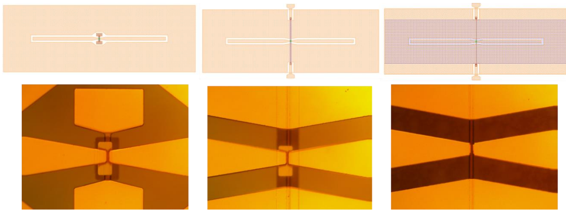
Figure 19. Three new designed switch structures on top and the fabricated results on the bottom.
