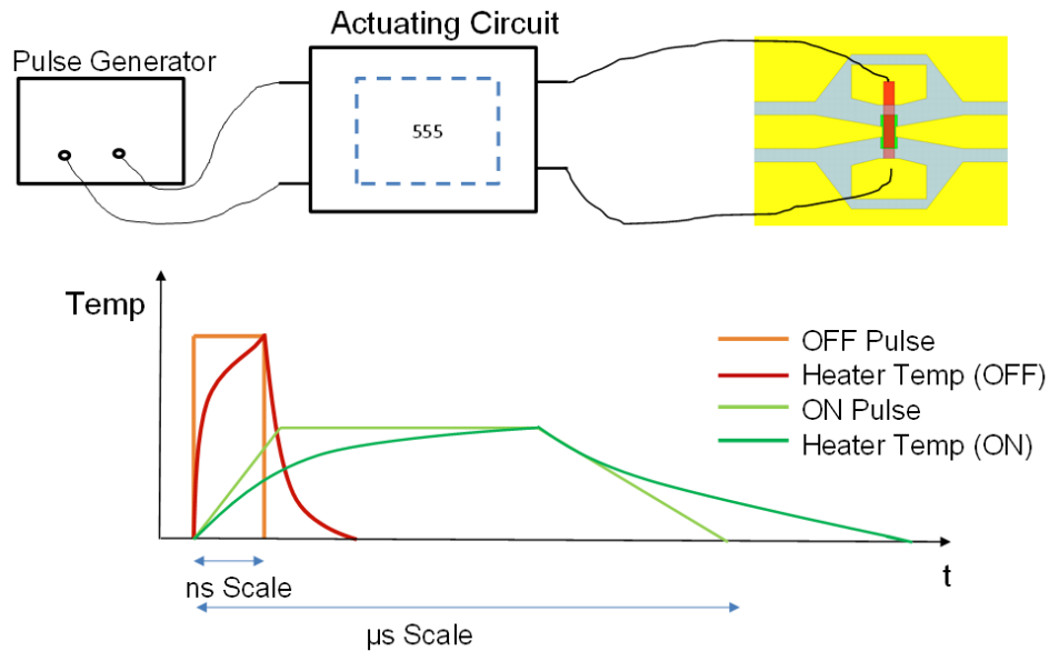
Figure 23. The biasing system concept for PCM switch actuation on top and the set temperature profiles along with the actual profiles are shown on the bottom.
