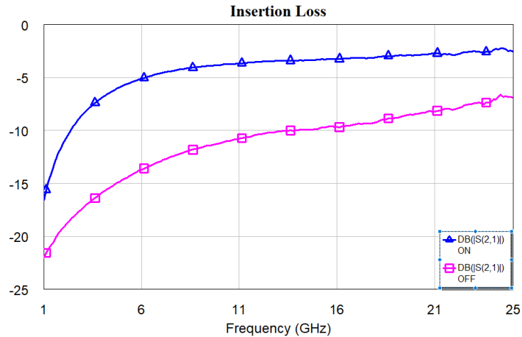
Figure 25. The measured insertion loss of the switch showing signs of phase-change as the switch was biased.
