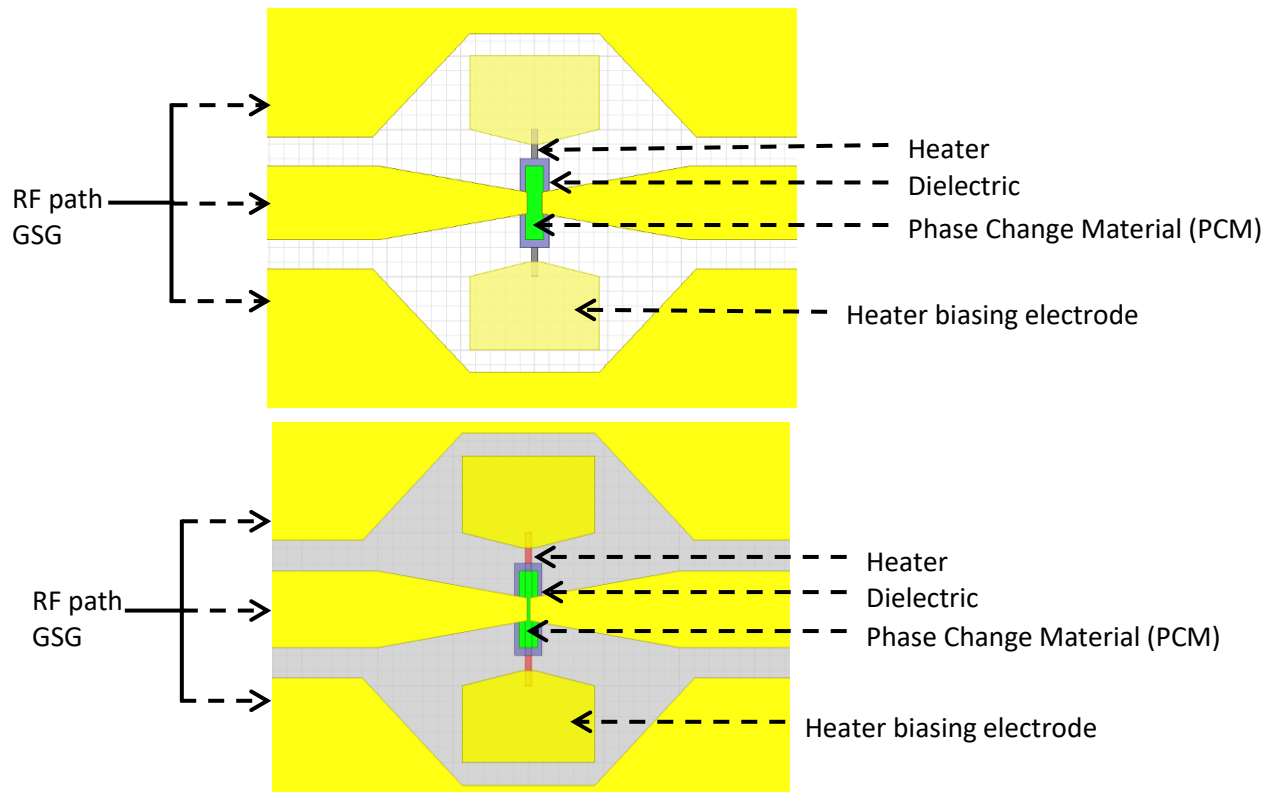
Figure 16. Layout of PCM-based RF switch, old structure on top and new design on bottom.
