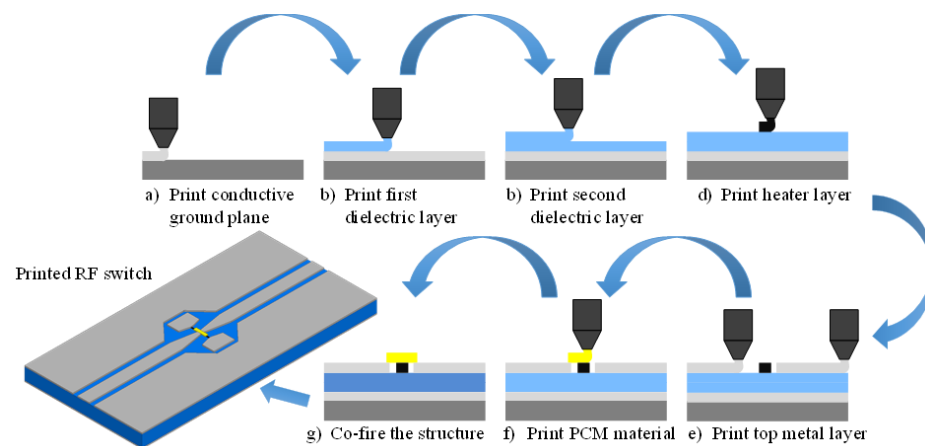
Figure 29. Conceptual example of multi-material printing. Four different materials are used to print a PCM-based RF switch (not drawn to scale).
