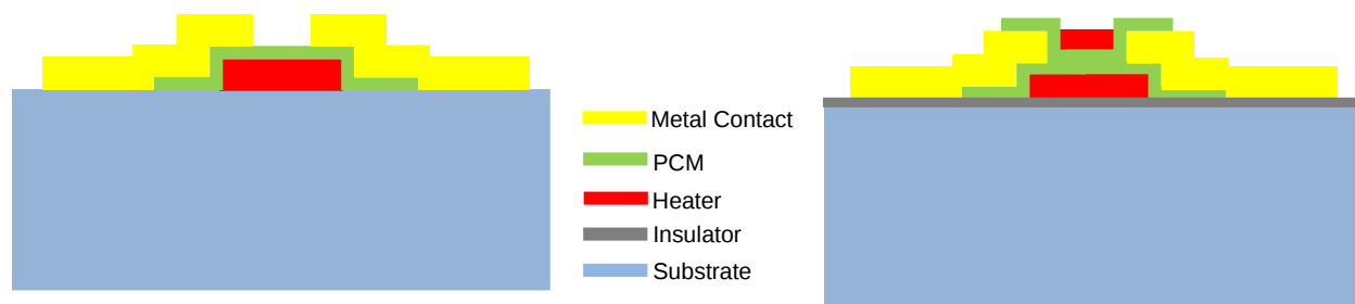
Figure 22. Direct heater cross-sectional views. Design with a bottom heater only on the left and a design with both a top and a bottom heater on the right.
