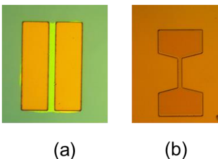
Figure 13. The etch results of W deposited by (a) E-beam and (b) Sputtering.
