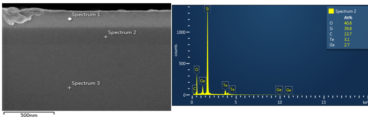
Figure 2. Cross section SEM view of GeTe thin film and Energy Dispersive X-ray spectra of germanium telluride
