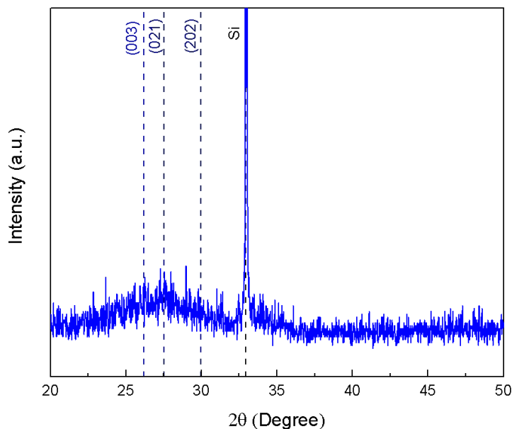
Figure 9. X RD pattern of the as-deposited GeTe film.
