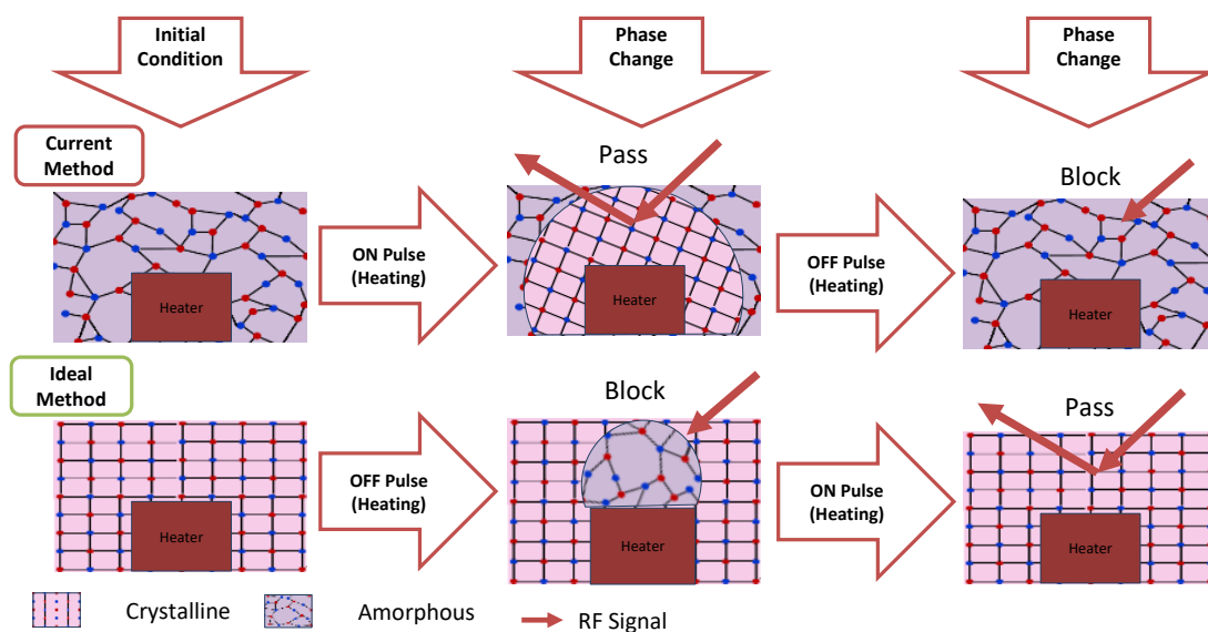
Figure 10. The configuration on the top represents the situation with the current samples, where the initial condition of the film is amorphous and only a small portion of the switch changes phase. The bottom shows a more ideal way, where the starting point is crystalline and activating the channel results in the off state [2].
