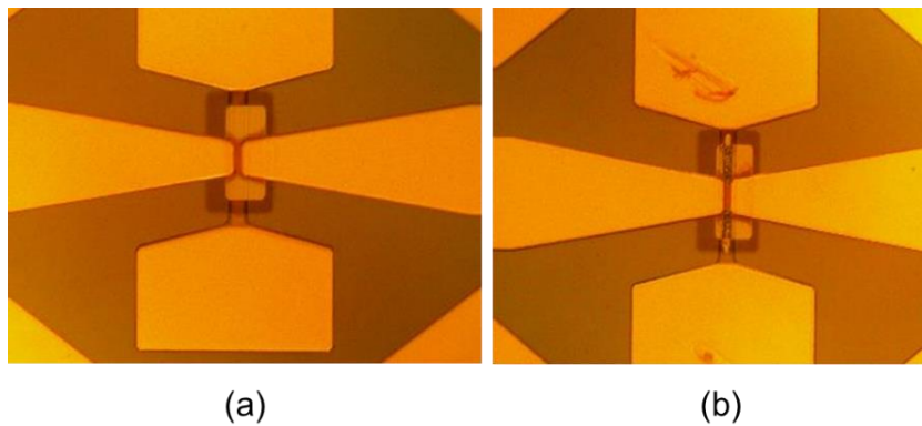
Figure 26. (a) Switch top view before applying OFF pulse, (b) Switch after applying OFF pulse.
