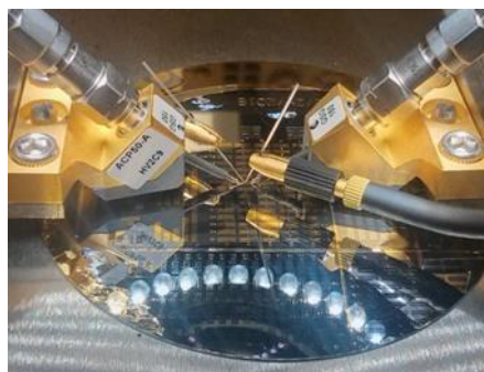
Figure 20. RF probe setup.
