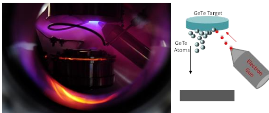
Figure 1. Pulsed Electron-beam Deposition (PED) in operation on the left along with a visualization on the right.
