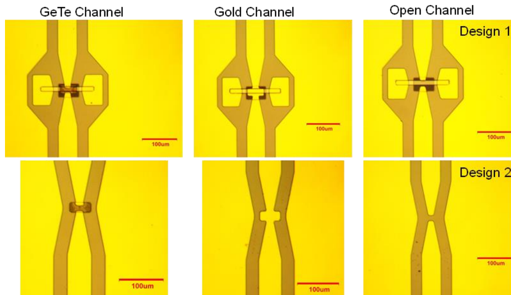
Figure 18. Devices included on the RF switch fabrication runs; left shows the devices with PCM, middle shows the short-circuited reference, and the right shows the open-circuited reference.
