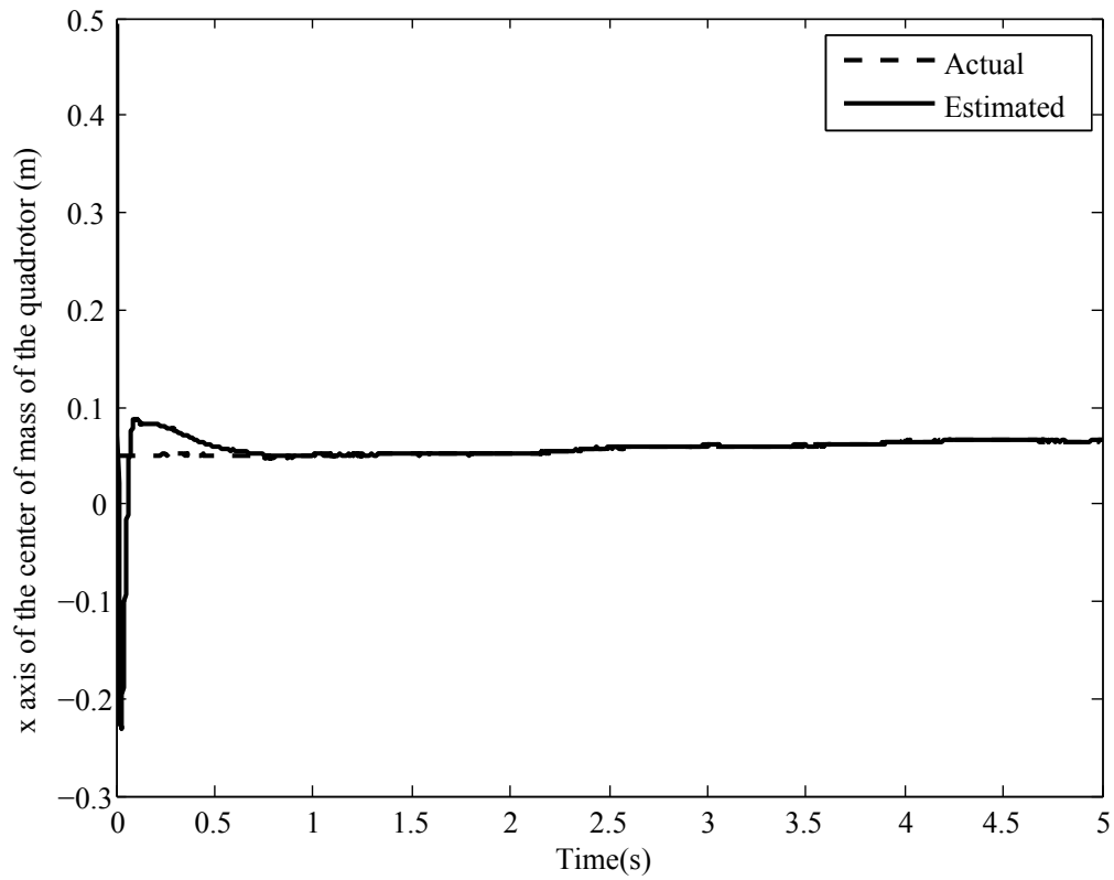
Figure 3.1.5. Estimation of x axis of the center of mass of the quadrotor for case 2
