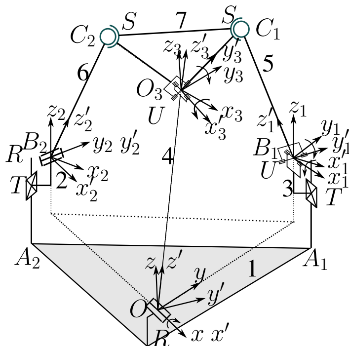
Figure 3.1. Parallel-mechanism system
