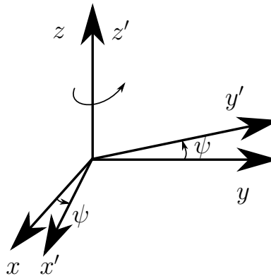
Figure 6.3. Yaw angle around z axis
