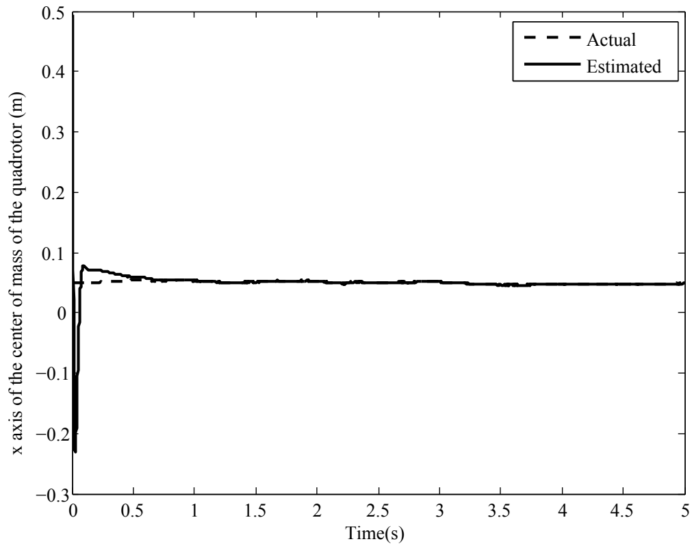
Figure 3.1.3. Estimation of x axis of the center of mass of the quadrotor for case 1
