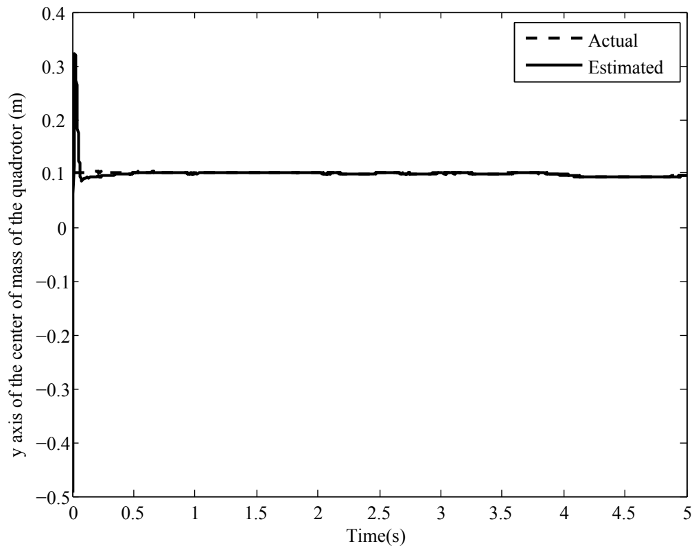
Figure 3.1.8. Estimation of y axis of the center of mass of the quadrotor for case 3
