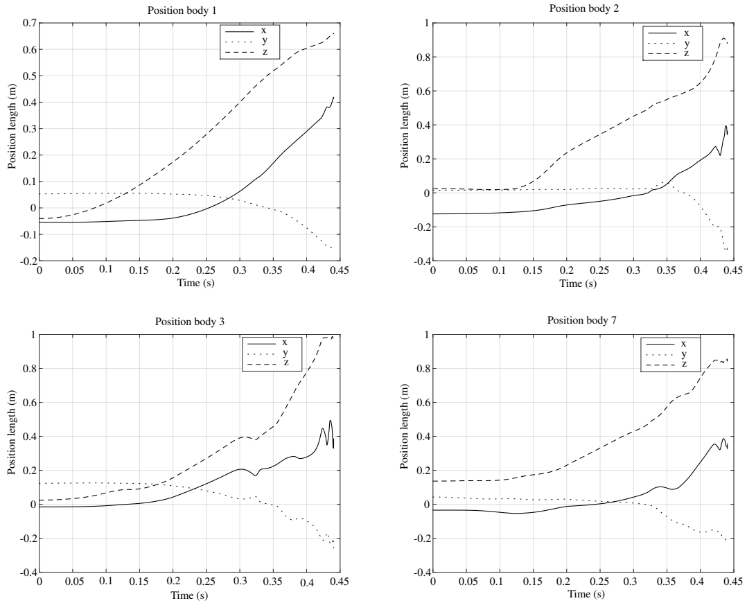
Figure 5.5. Case 3: Position of the epicenter of hexacopter (body 1), actuators (body 2 and 3), and platform attached solar panel (body 7) with respect to the global frame
