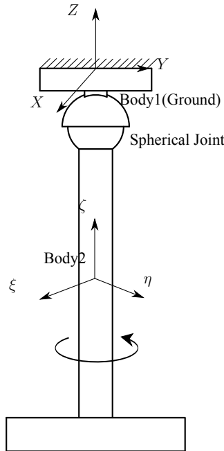
Figure 4.2. Two bodies connected by spherical joint
