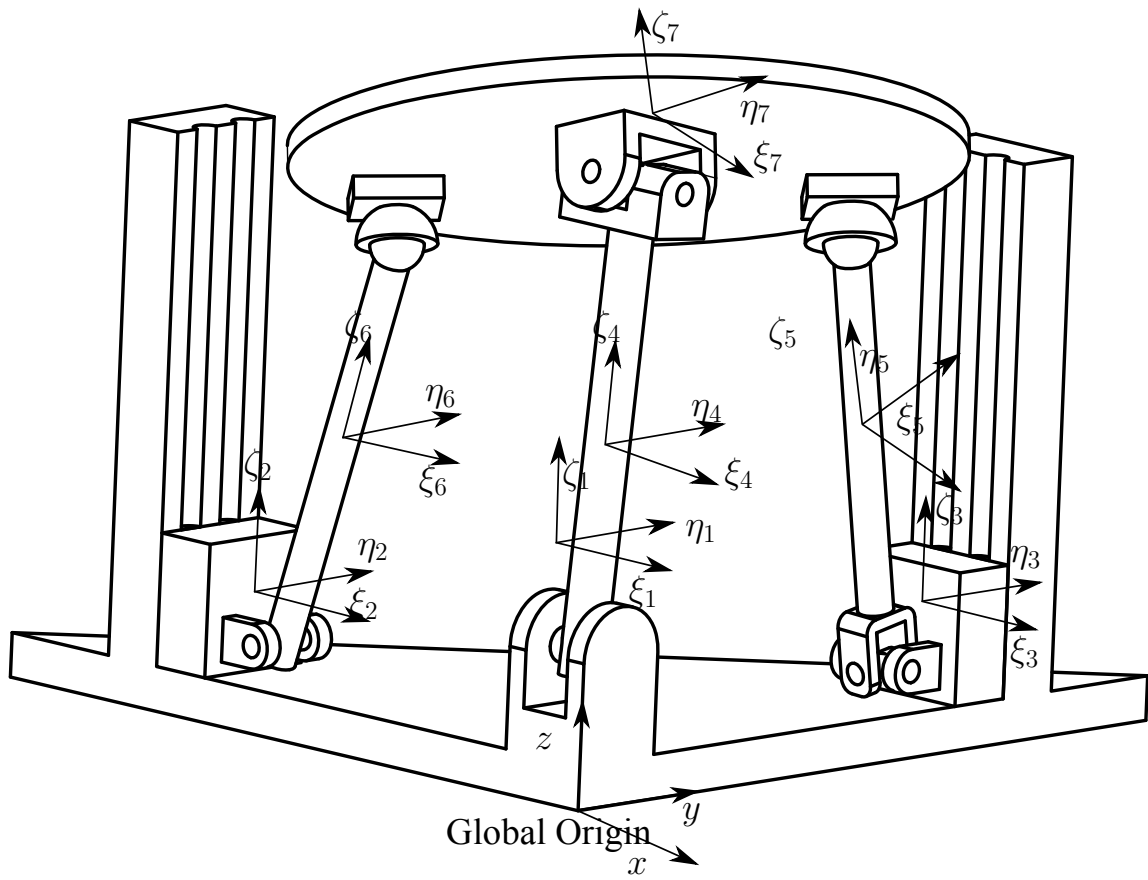
Figure 6.1. Global and Local coordinates
