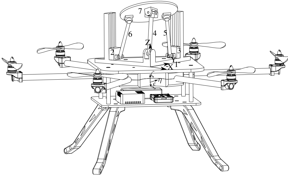
Figure 5.1. Parallel-mechanism-mounted UAV
