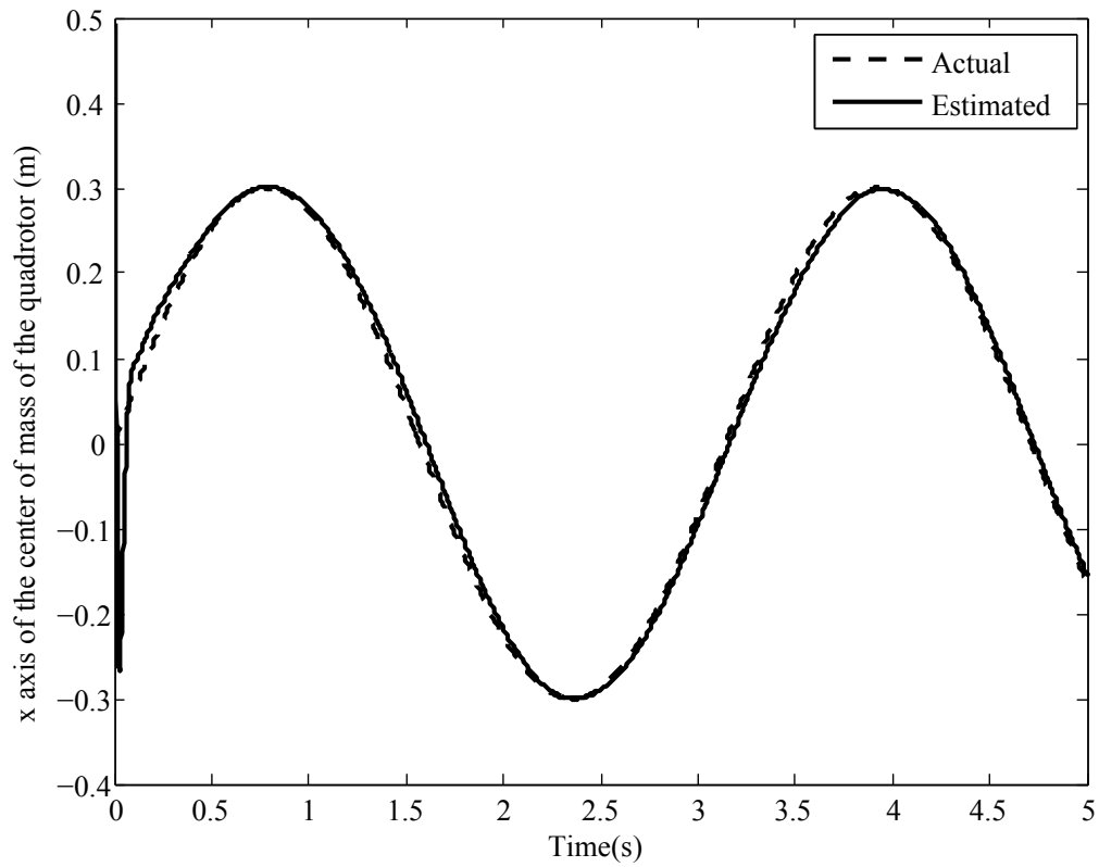
Figure 3.1.15. Estimation of x axis of the center of mass of the quadrotor for case 7
