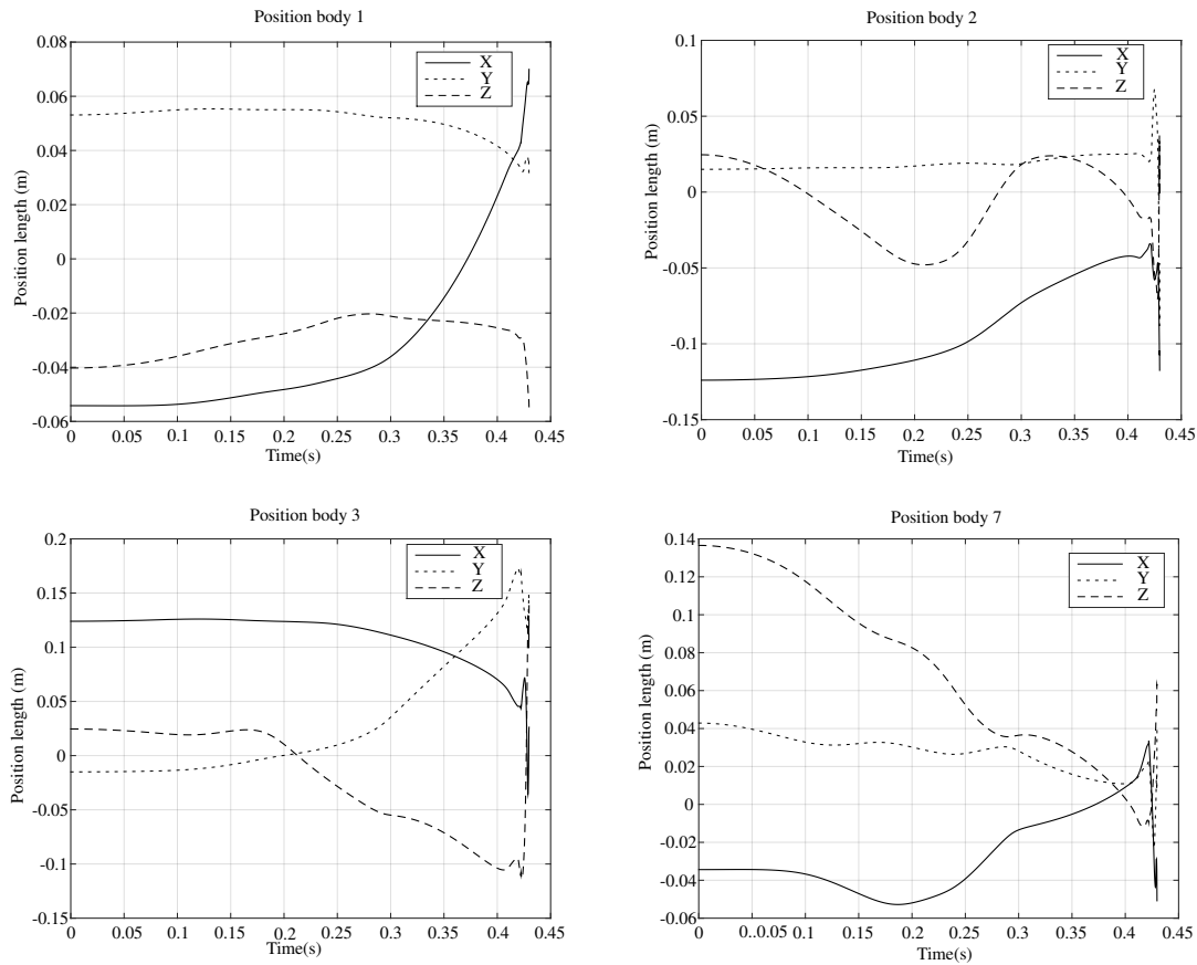
Figure 5.4. Case 2: Position of the epicenter of hexacopter (body 1), actuators (body 2 and 3), and platform attached solar panel (body 7) at the hover point with respect to the global frame
