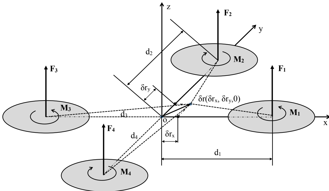
Figure 2.2.1. Free-body diagrams of the quadrotor which its the center of mass is not in the epicenter
