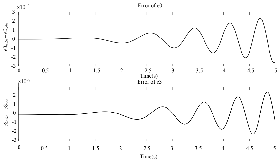
Figure 4.3. Error of Euler parameters between close form solution and Matlab ode
