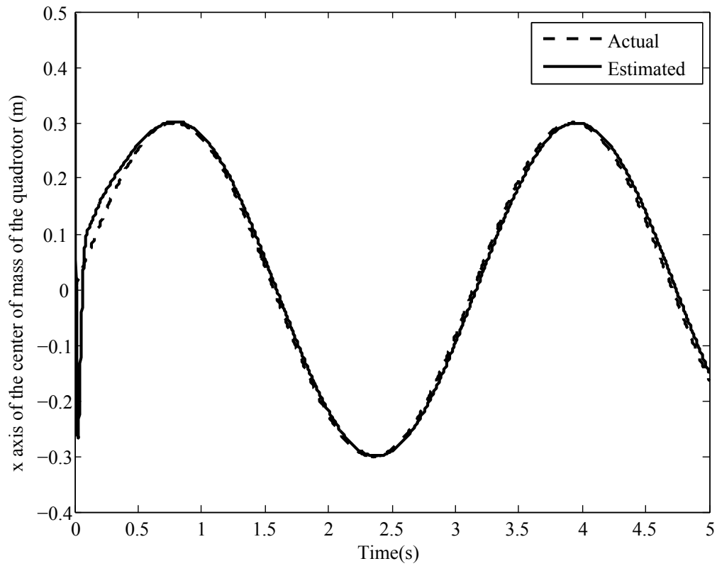
Figure 3.1.13. Estimation of x axis of the center of mass of the quadrotor for case 6
