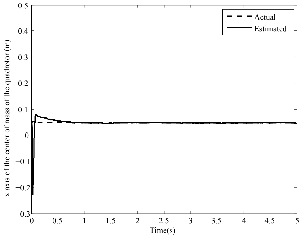
Figure 3.1.7. Estimation of x axis of the center of mass of the quadrotor for case 3
