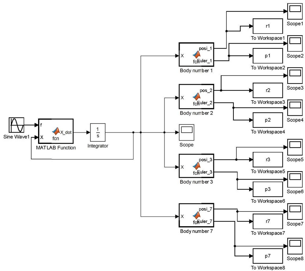
Figure 4.4. Flow simulation for a parallel-mechanism-mounted UAV
