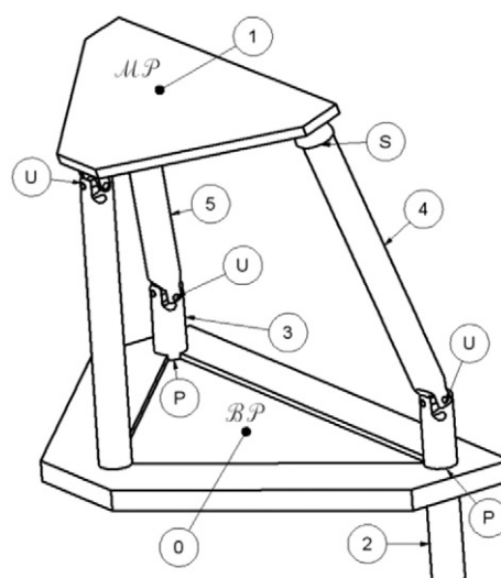
Figure 2.3. The U-2PUS parallel pointing system (Cammarata, 2015)
