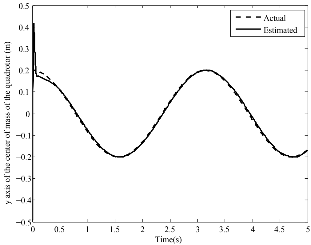
Figure 3.1.18. Estimation of y axis of the center of mass of the quadrotor for case 8
