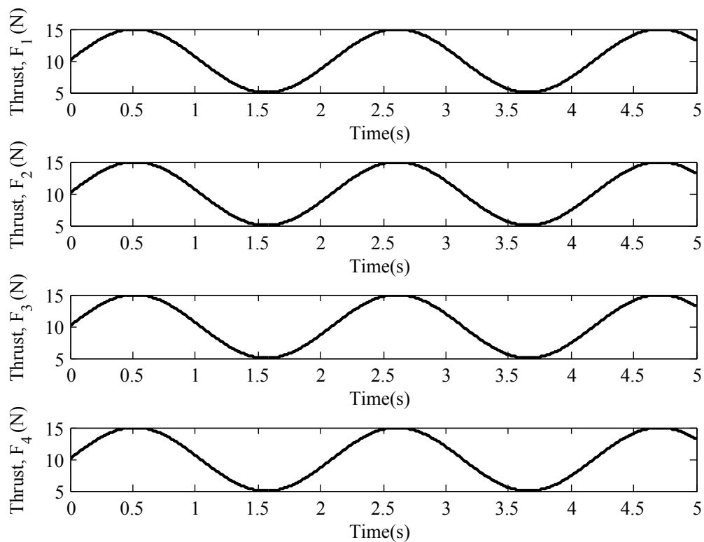
Figure 3.1.1. The value of thrusts F_1 , F_2 , F_3 and F_4 for case studies 3 and 7
