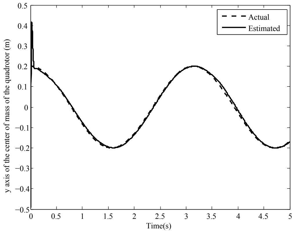
Figure 3.1.16. Estimation of y axis of the center of mass of the quadrotor for case 7
