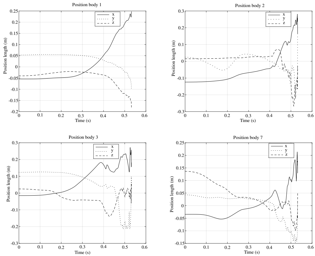
Figure 5.3. Case 1: Position of the epicenter of hexacopter (body 1), actuators (body 2 and 3), and platform attached solar panel (body 7) at the hover point with respect to the global frame
