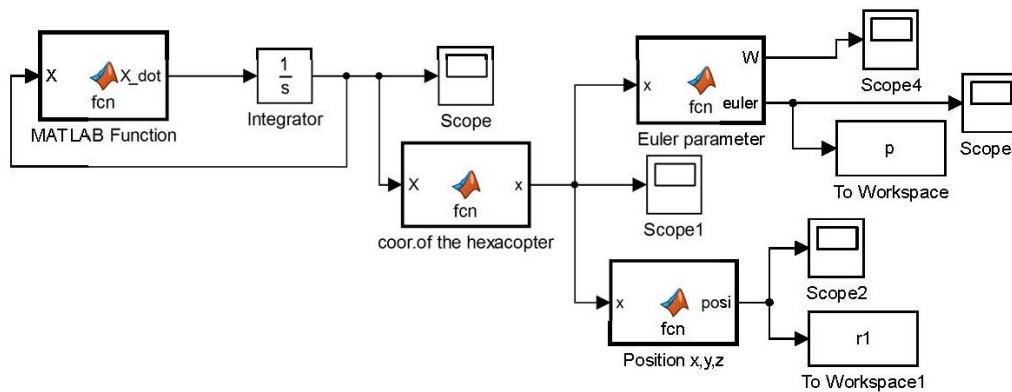
Figure 4.3. Flow simulation of hexacopter
