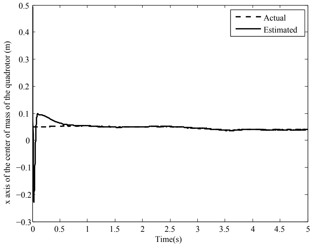
Figure 3.1.9. Estimation of x axis of the center of mass of the quadrotor for case 4
