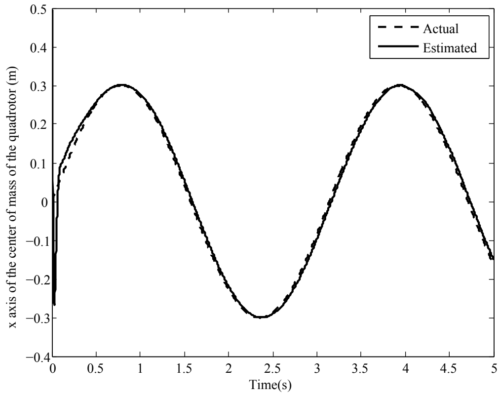
Figure 3.1.11. Estimation of x axis of the center of mass of the quadrotor for case 5
