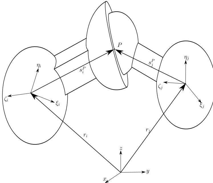
Figure 3.2. Spherical Joint
