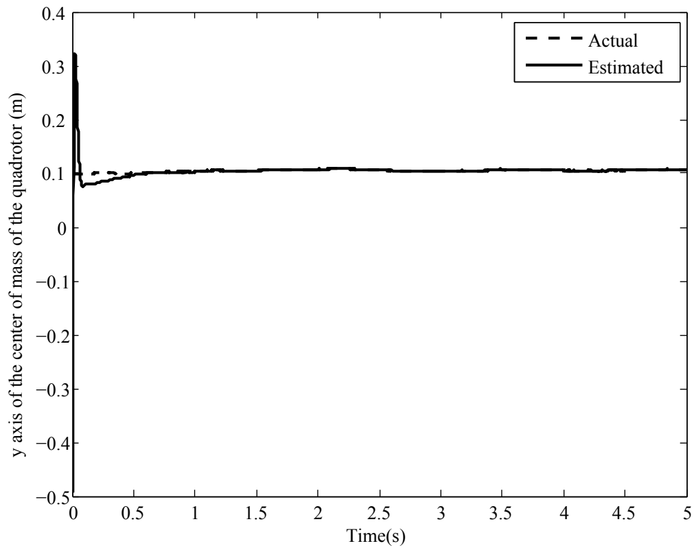
Figure 3.1.6. Estimation of y axis of the center of mass of the quadrotor for case 2
