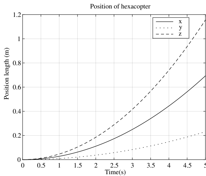
Figure 5.2. Position of the center of mass of hexacopter with respect to the global frame
