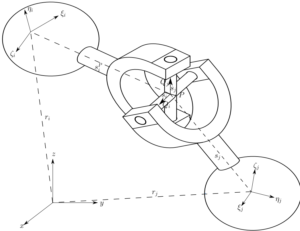
Figure 3.3. Universal Joint
