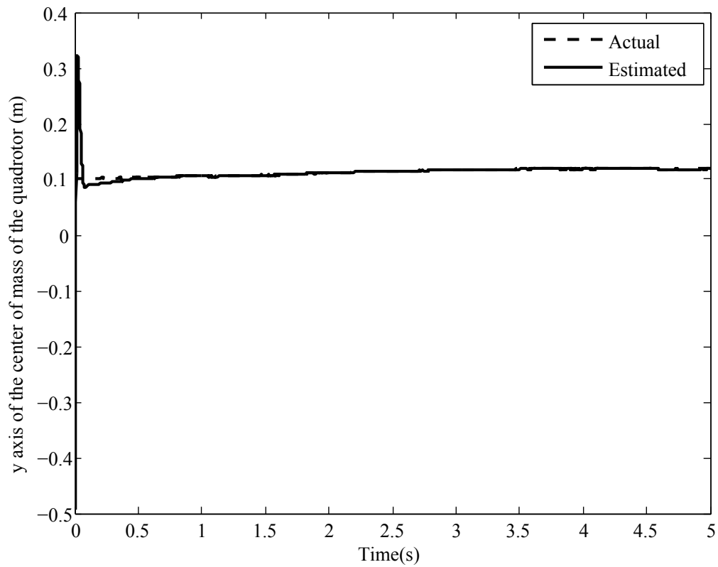
Figure 3.1.4. Estimation of y axis of the center of mass of the quadrotor for case 1
