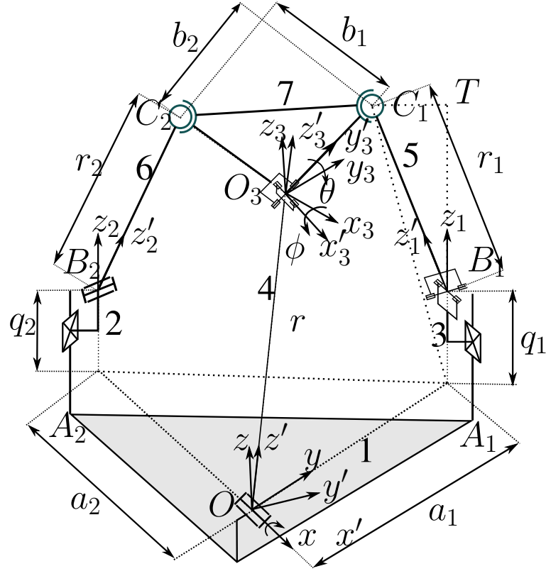
Figure 3.3. Variable length and angle of Parallel-mechanism system
