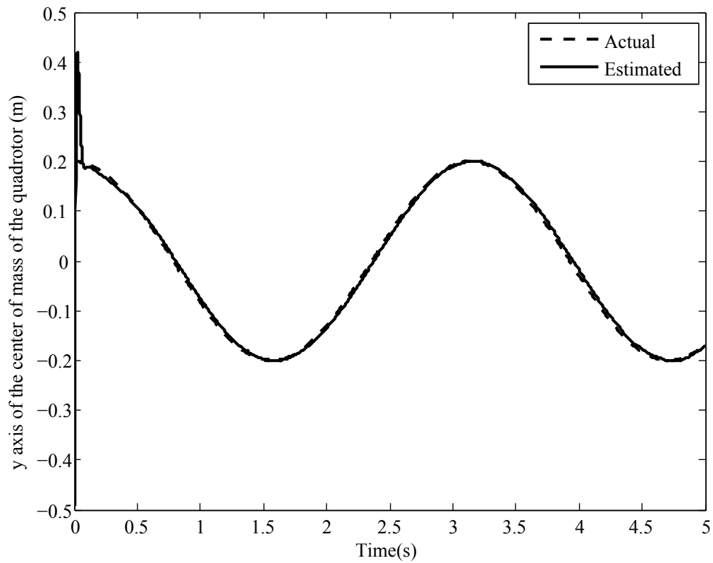
Figure 3.1.12. Estimation of y axis of the center of mass of the quadrotor for case 5
