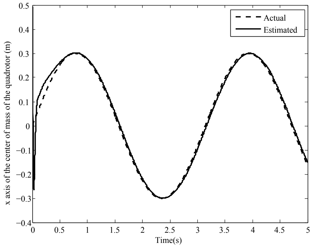
Figure 3.1.17. Estimation of x axis of the center of mass of the quadrotor for case 8
