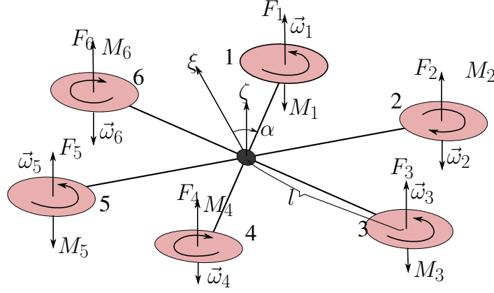
Figure 4.2. A model of hexacopter
