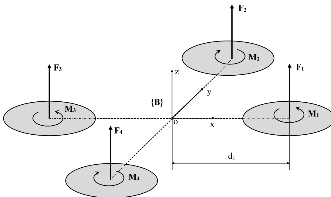
Figure 2.1.1. Notation for quadrotor equations of motion, [1]
