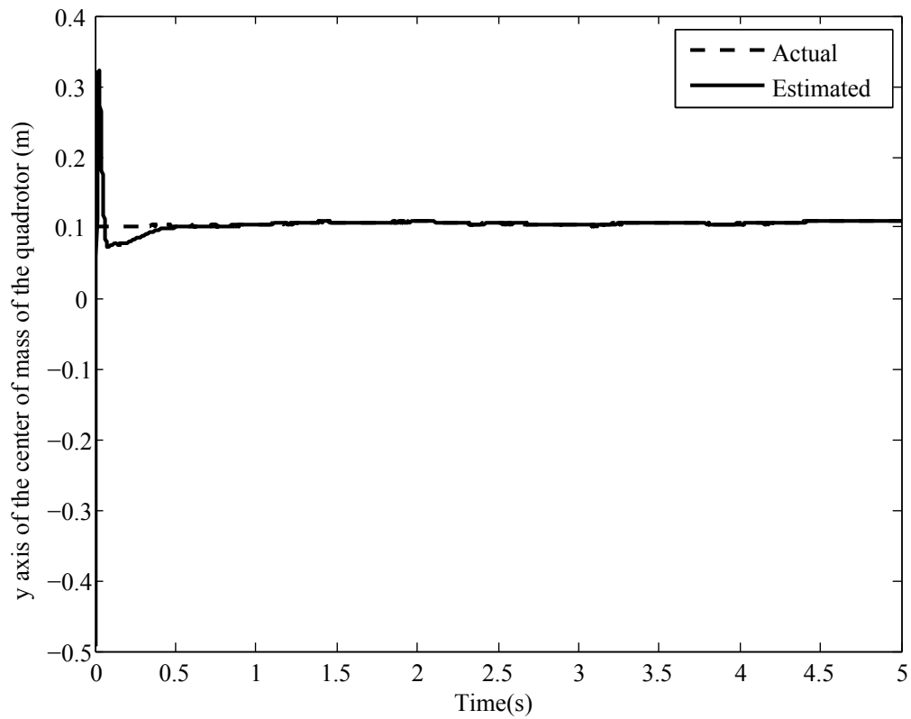
Figure 3.1.10. Estimation of y axis of the center of mass of the quadrotor for case 4
