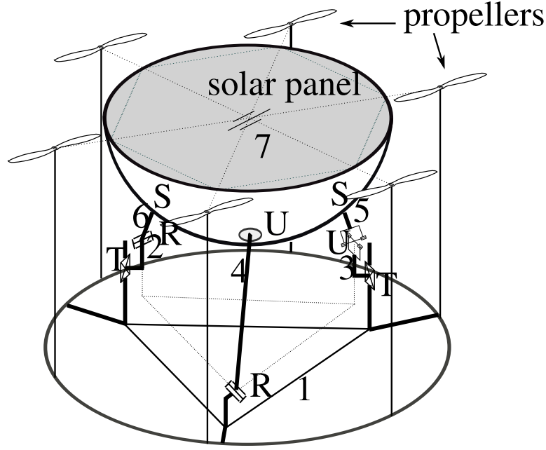
Figure 3.2. Parallel-mechanism-mounted UAV
