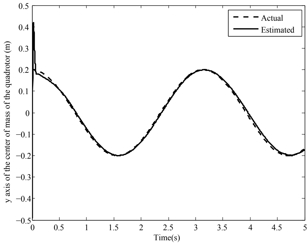
Figure 3.1.14. Estimation of y axis of the center of mass of the quadrotor for case 6
