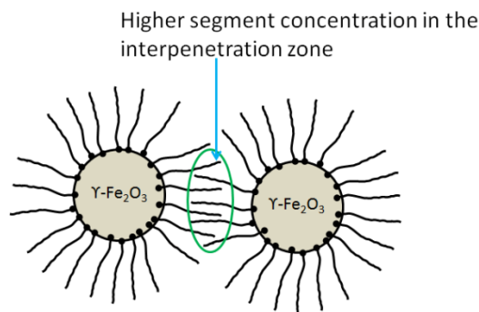
Fig. 3. Overlapping of the ligand (polymer segments) due to the magnetic attraction between two particles.
