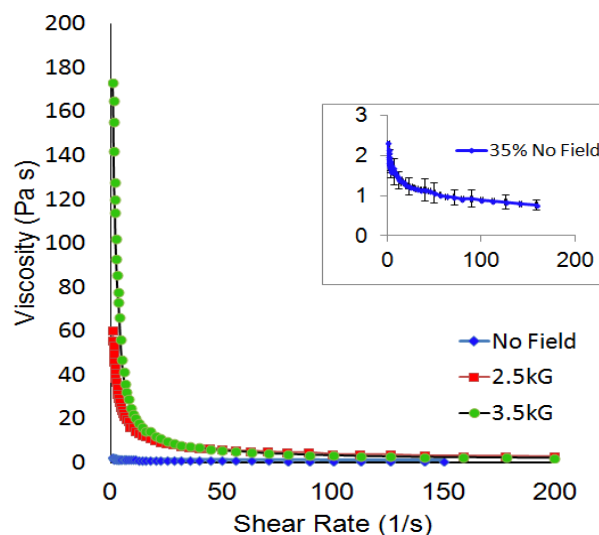
Fig. 9. Change in viscosity with shear rate and magnetic field for the ILFF containing 35 % (w/w) \gamma - \text{Fe}_2\text{O}_3 nanoparticles.
