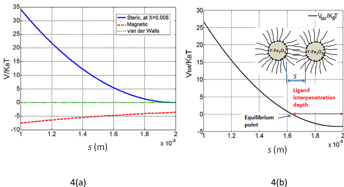
Fig. 4(a) shows individual components (steric, magnetic and van der Waals) of the interaction potentials ( V ) when the magnetization, M is 60 emu/g, and 4(b) shows the net interaction potential and the depth of ligand interpenetration caused by the attractive forces between the particles. K_B T is thermal units.
