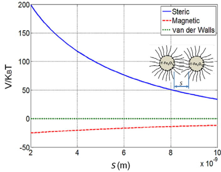
Fig. 7. The components of the total interaction potential when s < l at a magnetisation of 65 emu/g.
