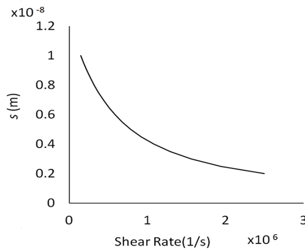
Fig. 8. Particle surface-to-surface separation distance ( s ) when the hydrodynamic and steric forces are at equilibrium vs the shear rate.
