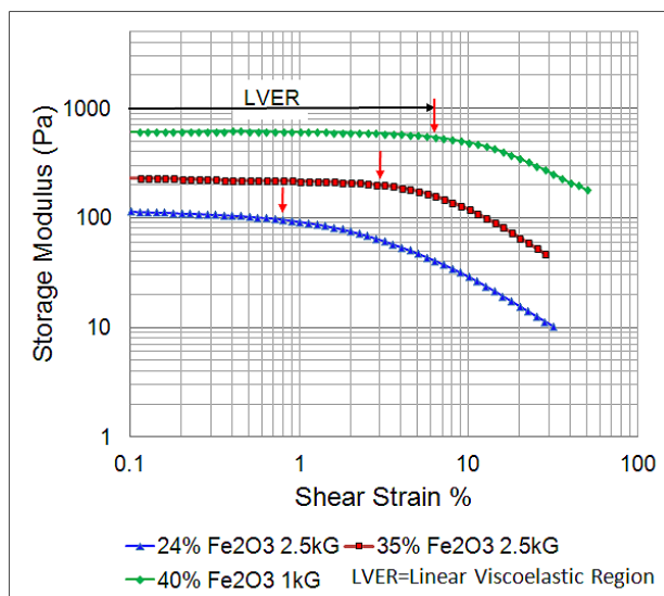
Fig. 10. Storage (Elastic) modulus of the ferrofluid containing 24 and 35 wt.% \text{Fe}_2\text{O}_3 under a high magnetic field strength of 2.5 kG, and 40 wt.% \text{Fe}_2\text{O}_3 under a magnetic field strength 1 kG.
