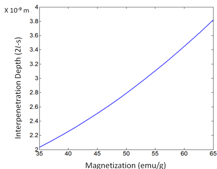
Fig. 5. Depth of interpenetration of the ligand with change in magnetization of the nanoparticles. l = the extended length of the ligand(10 nm).
